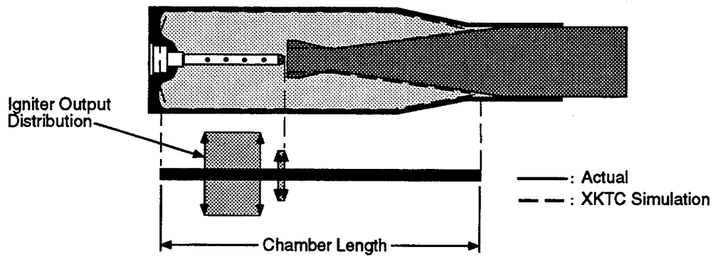
Baseline Igniter
