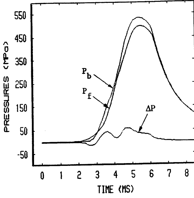
Figure 5. Pressure data for Igniter B.
