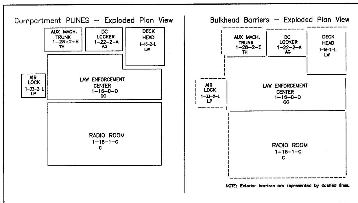
Figure IV-1 Compartment Polylines vs. Bulkhead Barriers
