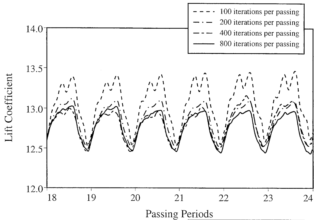
(a) vane
