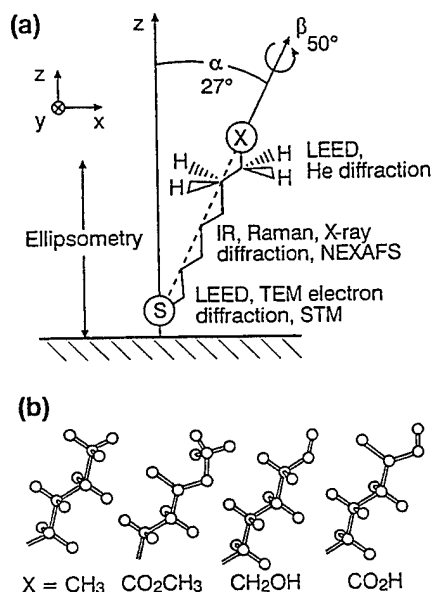
Fig. 2. (a) Schematic side-view of the orientation of a single, long-chain thiol molecule adsorbed on gold. The tilt angle ( \alpha ) is with respect to the surface normal, whereas the twist angle ( \beta ) is with respect to a plane established by the chain axis and the surface normal vectors. The techniques listed to the right are those used to determine the structure of that portion of the molecule. (b) The surface projections of several representative group. (From Dubois, L. H. and Nuzzo, R. G. (1992), Ann. Rev. Phys. Chem. , 43, 437; With permission.)
