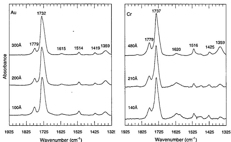
Figure 3. IRRAS spectra of BPDA-PDA on Au and \text{Cr/Cr}_2\text{O}_3 as a function of polymer film thickness.
