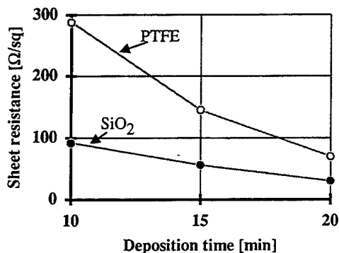
Fig. 3: Sheet resistance of TiN interlayer on PTFE and SiO 2 vs. deposition time
