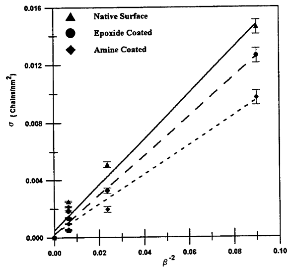
Figure 2: Scaling behavior for highly asymmetric polymers ( \beta > N_A^{0.5} ) on Native (▲), Epoxide (●) and Amine (◆) surfaces
