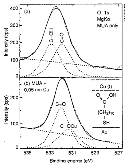
Fig. 5. Curve-resolved O 1s photoemission peaks for the \text{HS}(\text{CH}_2)_{10}\text{COOH} SAM on gold before (a) and after (b) deposition of 0.05 nm of copper.
