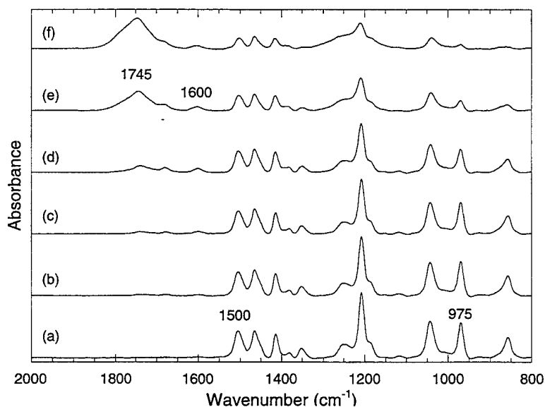
Figure 9. IRRAS spectra of 400\text{ \AA} films of MEH-PPV on Al. Spectra are shown for the as-coated film (a), and after exposure to dry air and UV irradiation for (b) 2h, (c) 5h, (d) 12 h, (e) 24 h, and (f) 36 h.
