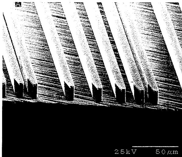
Figure 1: Secondary electron SEM image of edge of fully processed uncleved (110) Si trench die used in experiments. Trench walls and bases consist of Si. Trench depth is 15 \mu\text{m} .
