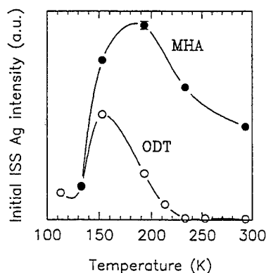
Fig. 8. Initial ISS peak intensities for 1.0 nm Ag on MHA and ODT after deposition at temperatures from 113 K.
