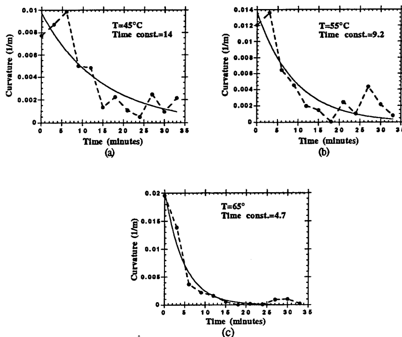
Figure 1. Measured change in curvature of the bonded structure as a function of time at (a) 45^{\circ}\text{C} , (b) 55^{\circ}\text{C} , and (c) 65^{\circ}\text{C} . The exponential relaxation curve fit is shown with the time constants.
