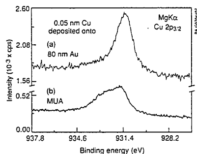
Fig. 6. Copper photoemission peaks for 0.05 nm of copper on (a) 80 nm of gold and (b) the \text{HS}(\text{CH}_2)_{10}\text{COOH} SAM on gold.
