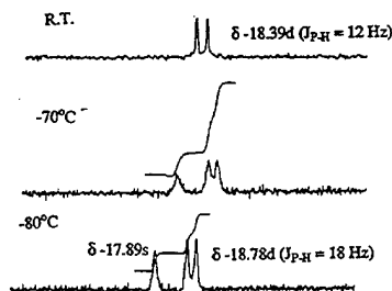
Figure 2. Variable Temperature ^1\text{H} NMR Spectra of (4)
