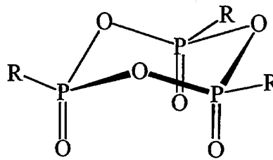
C_{3v} symmetry, A_3 spin system; R = 2,4,6 -Trimethylphenyl
