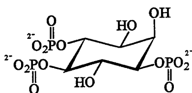
D-Ins(1,4,5)P 3 (1)
