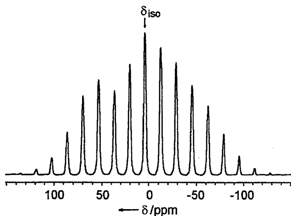
FIGURE 1 31 P CP/MAS spectrum of Ph-C(O)-P(O)(OH)(ONa)
