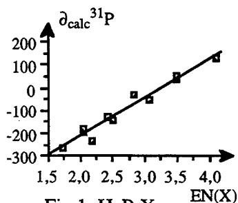
Fig.1: \text{H}_2\text{P-X}
