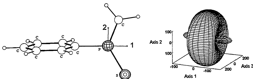
FIGURE 1 Orientation of the principal axes 1, 2 and 3 in the molecular framework of \text{C}_6\text{H}_5\text{P(=S)(=CH}_2\text{)} with the corresponding ^{31}\text{P} tensor ovaloid
