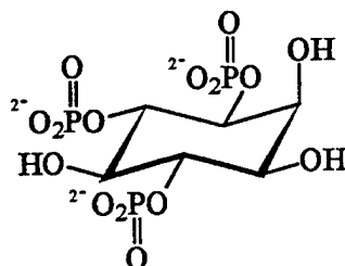
L-Ins(1,4,6)P 3 (3)
