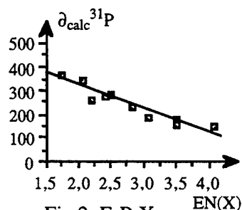
Fig.2: \text{F}_2\text{P-X}
