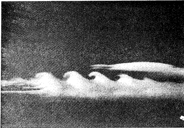
Waves associated with atmospheric windshear can cause turbulent regions at all flight levels. Often occurring in the vicinity of mountains, turbulence can exist without visible cloud formations to provide cues for pilots to avoid (Photograph © B. Martner).
