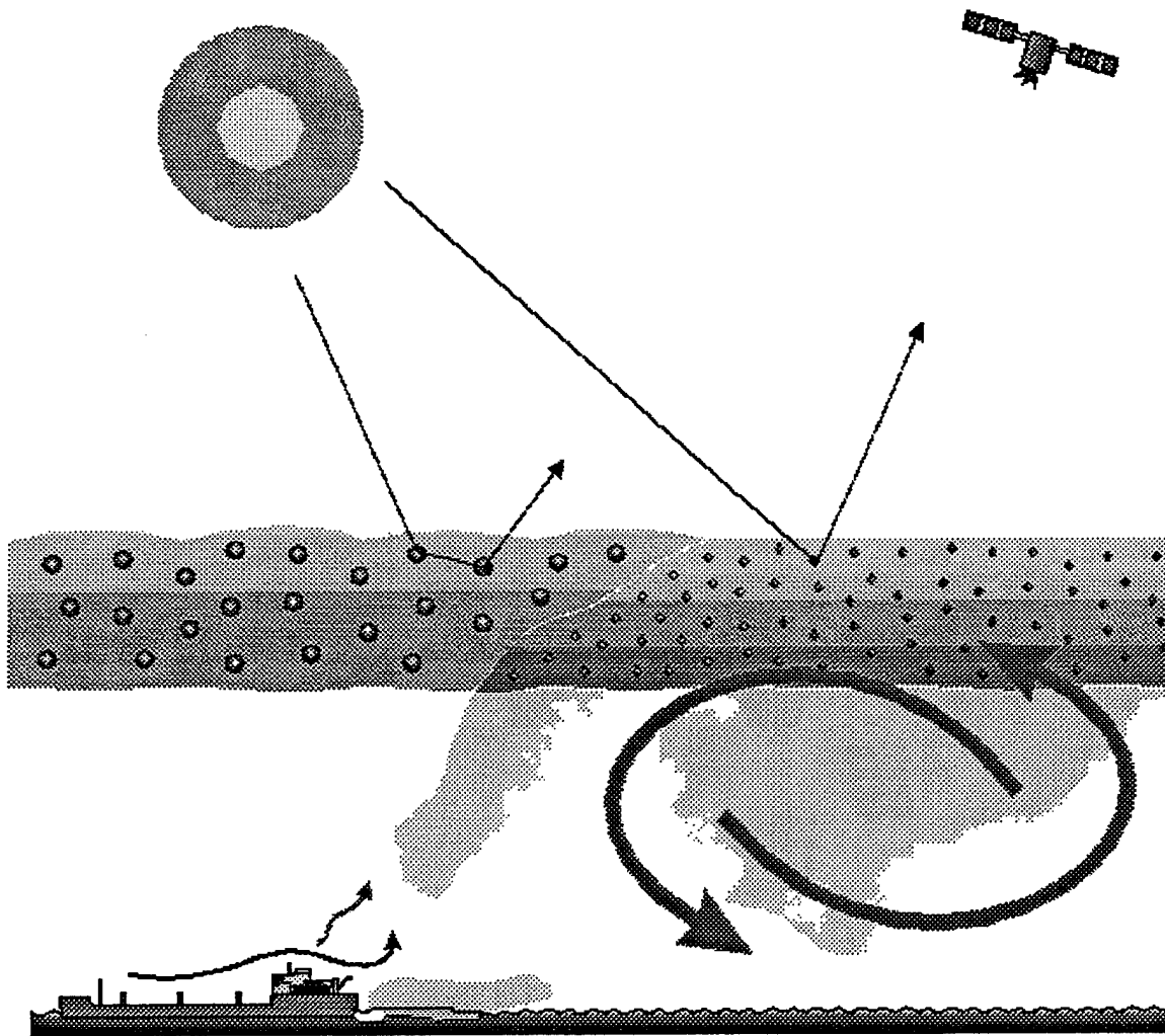
Figure 2 The formation of shiptracks in the Marine Atmospheric Boundary Layer. The cloud layer is represented by the shaded layer with droplet sizes and numbers represented within the layer. The thin lines represent the 3.7 \mu\text{m} solar radiation and the modified scattering. Turbulent mixing is indicated by the large arrows, while the thin curved lines represent buoyancy due to exhaust heat and mechanical turbulence produced by the ships motion. From Brown (1995).
