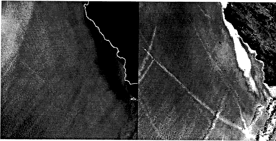
Figure 1. A comparison of AVHRR shiptrack signatures for the visible 0.63 micron wavelength (left) and near-infrared 3.7 micron wavelength (right). The image were taken on 27JUN87 2247GMT passing over the west coast of the United States. Notice the increased number and clarity of shiptracks in the 3.7 micron image.
