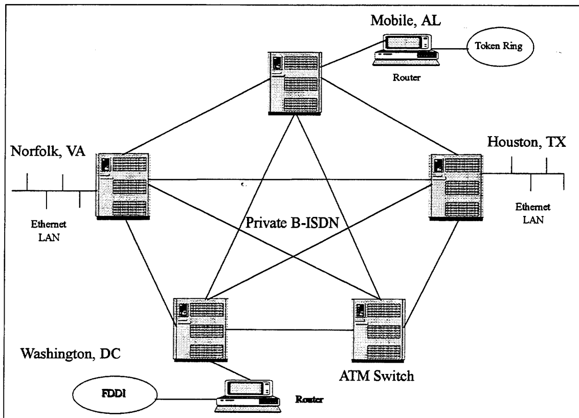
Figure 2.13 ATM WAN
