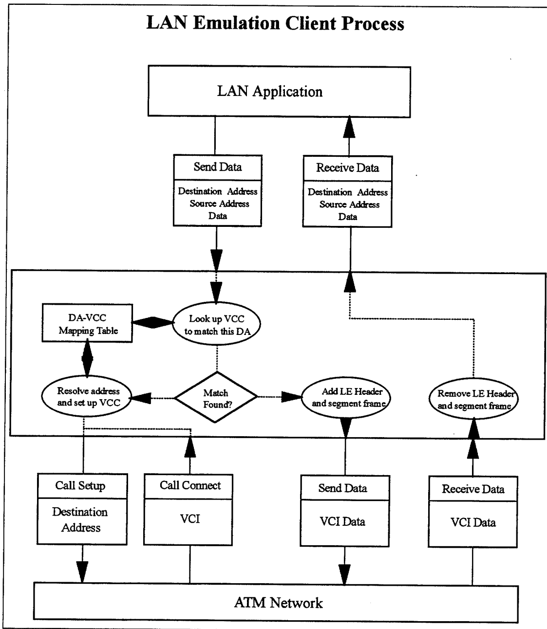
Figure 5.9 LAN Emulation Client Process
