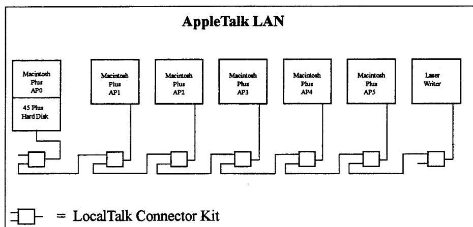
Figure 4.6 AppleTalk LAN
