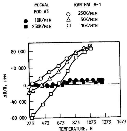
FIGURE 13. - FRACTIONAL RESISTANCE CHANGE OF KANTHAL A-1 AND FECrAl MOD #3 AS A FUNCTION OF TEMPERATURE.
