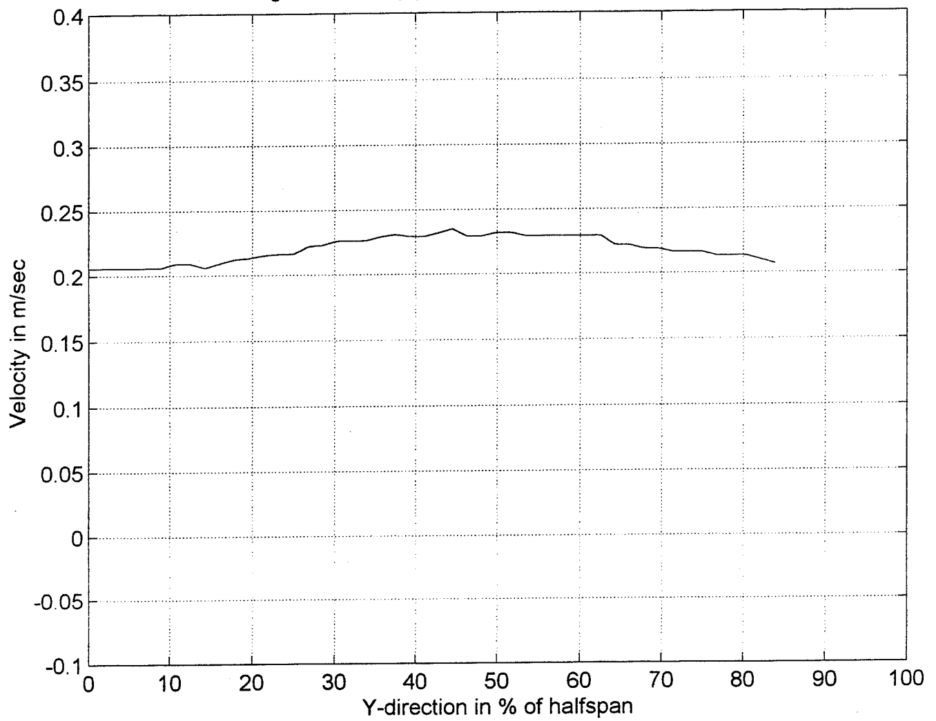
Fig.113: Velocity profile at x=38.62\% , z=27.73 mm
