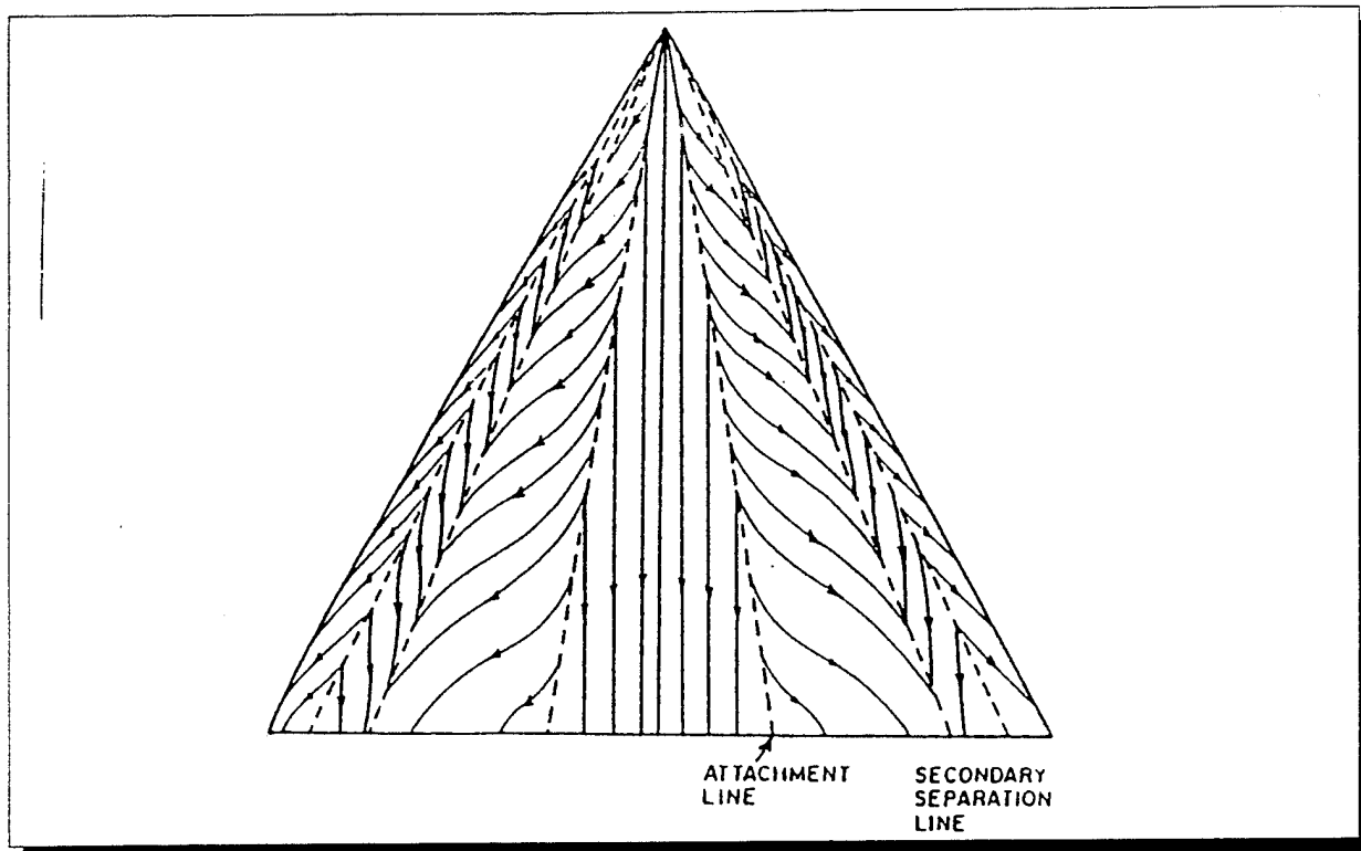
Fig. 7: Surface flow pattern over a single delta - wing
