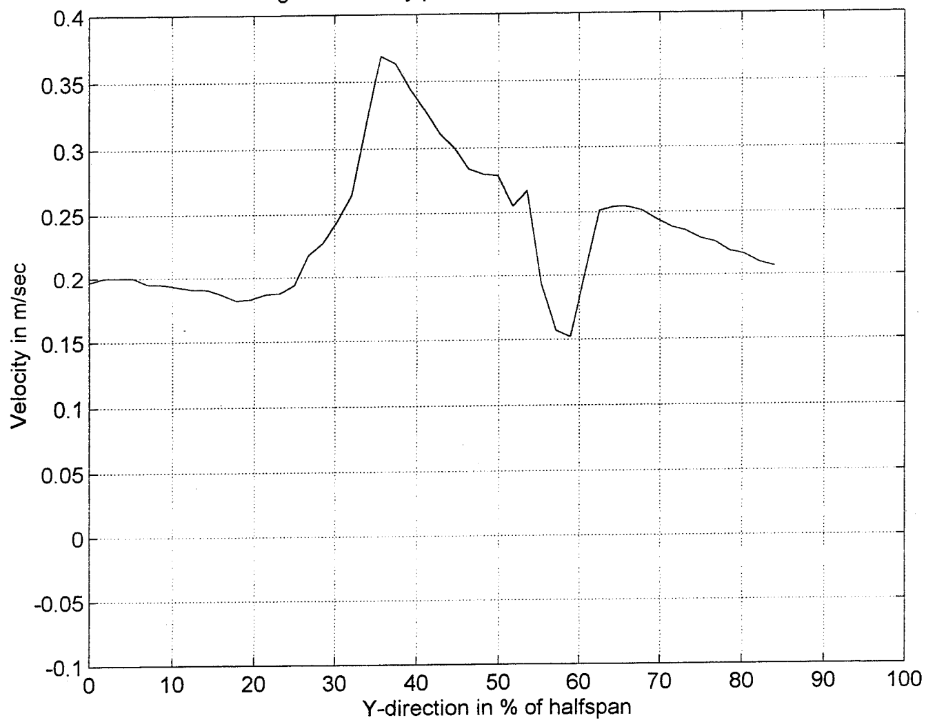
Fig.107: Velocity profile at x=38.62\% , z=9.73 mm
