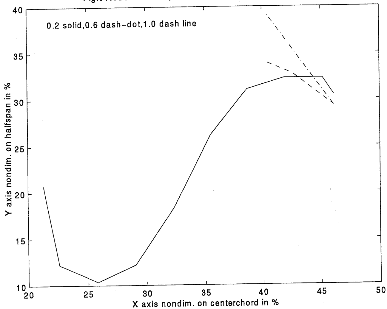
Fig.91:Strake vortex, AOA=22.5 deg, V=0.2-0.6-1.0 ft/sec
