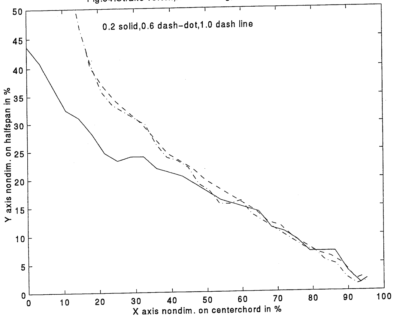
Fig.84:Strake vortex, AOA=10 deg, V=0.2-0.6-1.0 ft/sec
