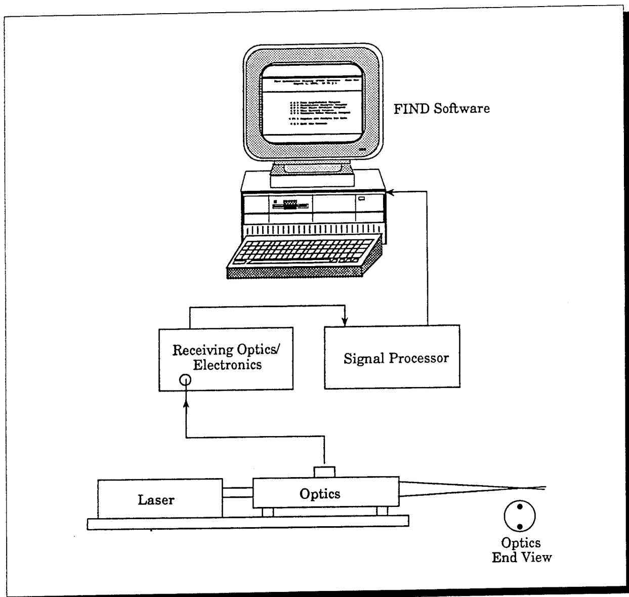
Fig. 16: FIND Software
