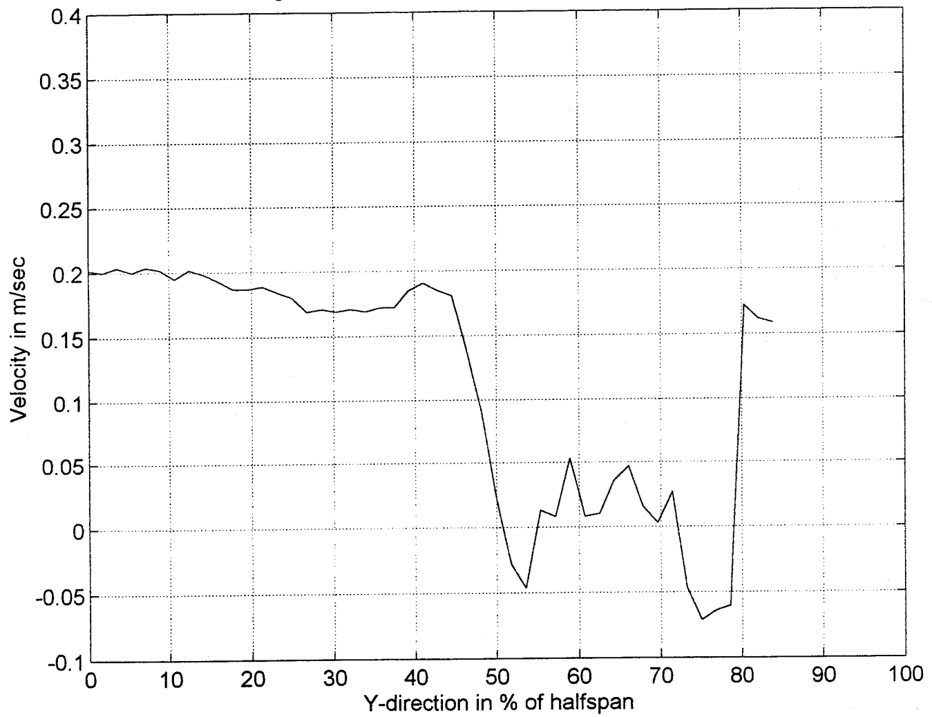
Fig.104: Velocity profile at x=38.62\% , z=0.73 mm
