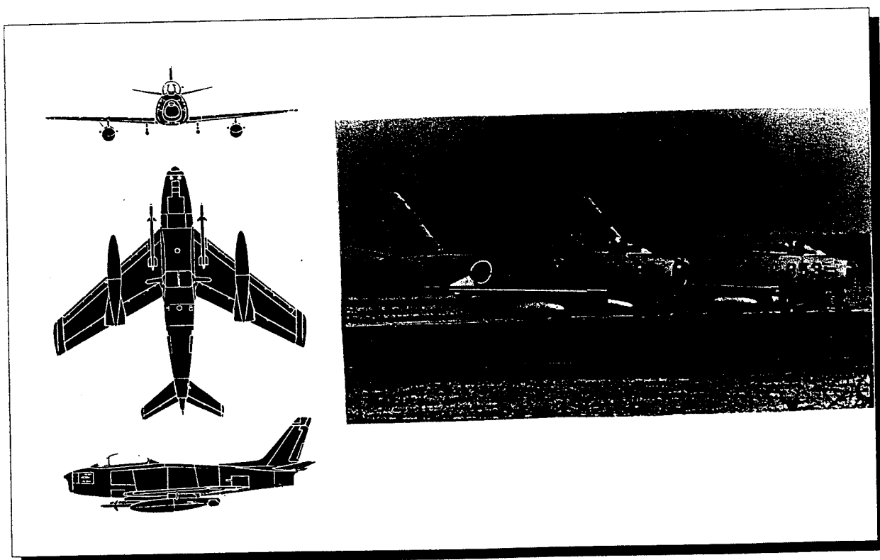
Fig. 2: North American F - 86 Sabre Midget
