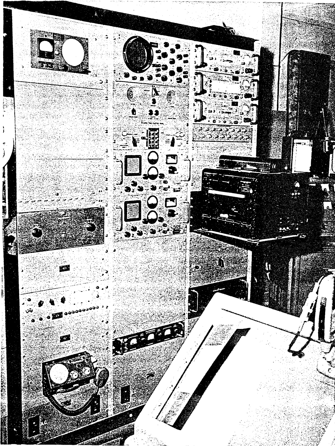
Fig. 3—Ground station.
