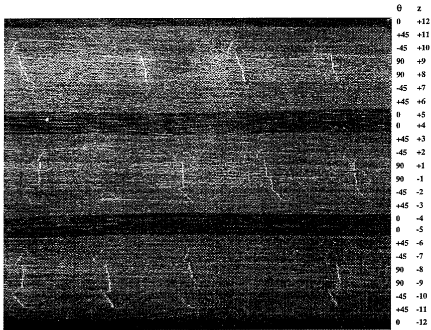
FIGURE 2. PHOTOMICROGRAPH OF [0/45/-45/90]_{s3} LAMINATE SHOWING PLY CRACKS
