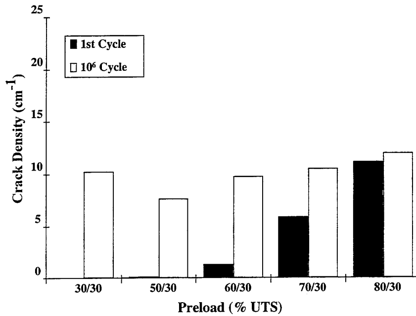
FIGURE 30. 30% UTS FATIGUE CRACK DENSITIES AT 1 AND 10 6 CYCLES VS. PRELOAD FOR 90° PLYS
