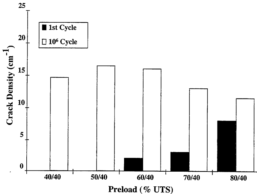
FIGURE 33. 40% UTS FATIGUE CRACK DENSITIES AT 1 AND 10 6 CYCLES VS. PRELOAD FOR -45° PLYS
