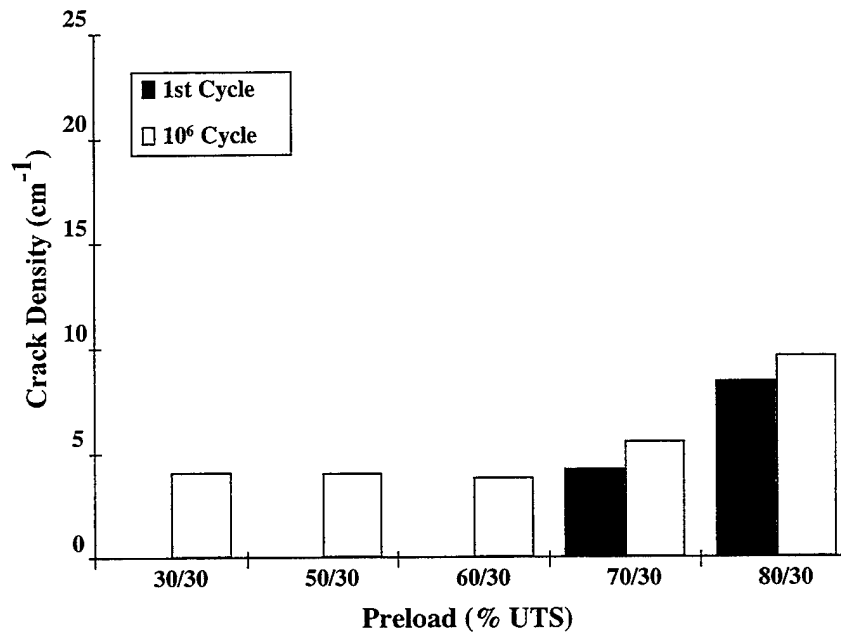
FIGURE 31. 30% UTS FATIGUE CRACK DENSITIES AT 1 AND 10 6 CYCLES VS. PRELOAD FOR -45° PLYS
