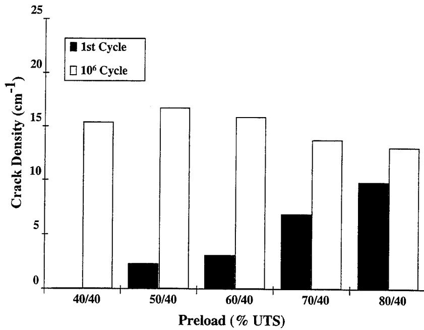
FIGURE 32. 40% UTS FATIGUE CRACK DENSITIES AT 1 AND 10 6 CYCLES VS. PRELOAD FOR 90° PLYS
