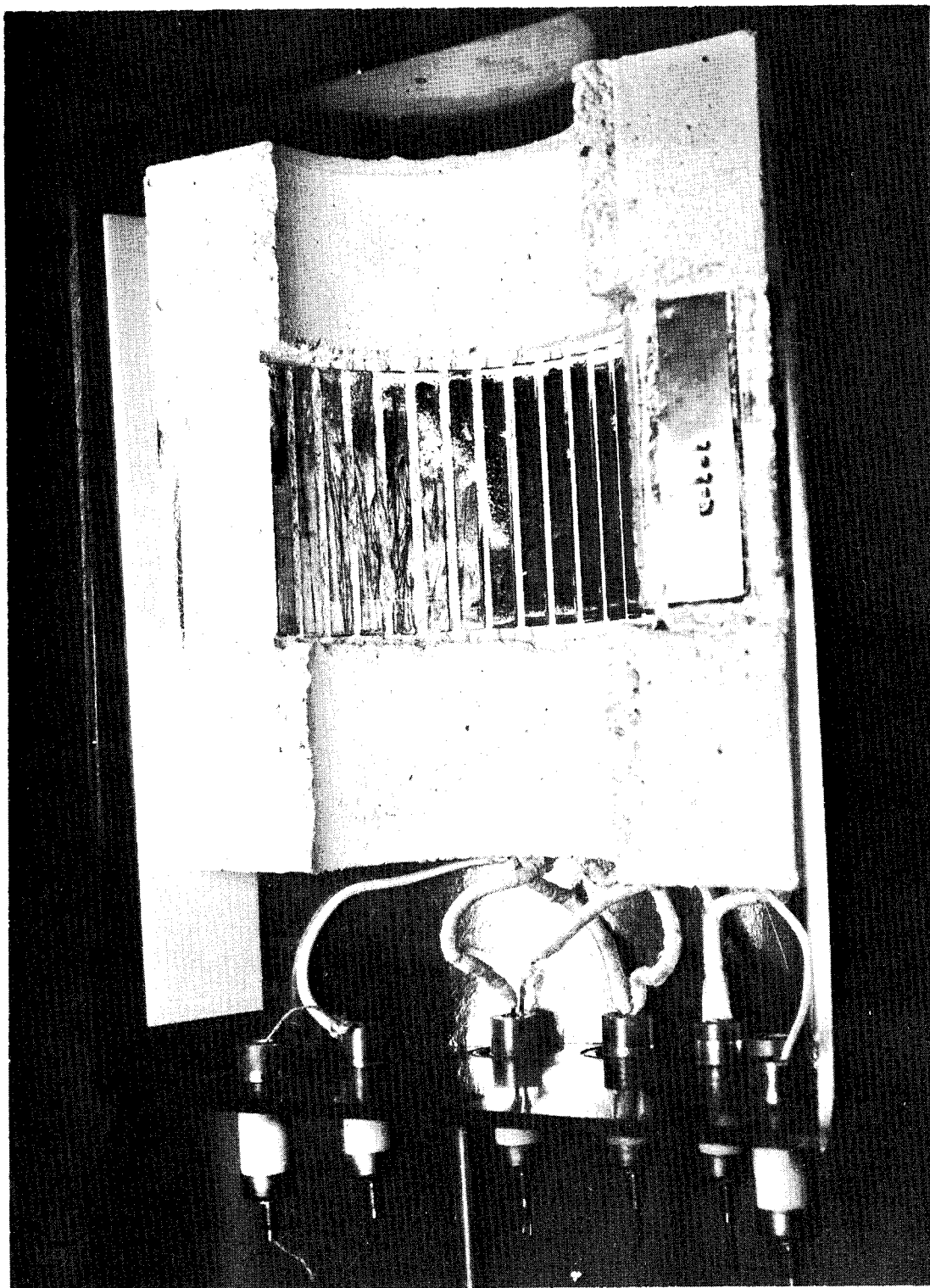
FIGURE 11-15 XI-2R, STATORETTE PRIOR TO CLOSURE
