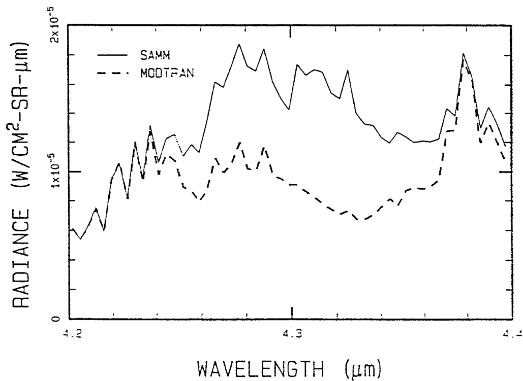
Figure D-8. SAMM/MODTRAN Test Case 6 Comparison in the 4 \mu\text{m} Region.
