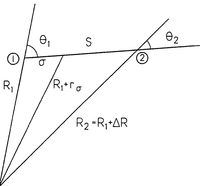
Figure H-1. Straight Layer Segment From Point 1 to Point 2.
