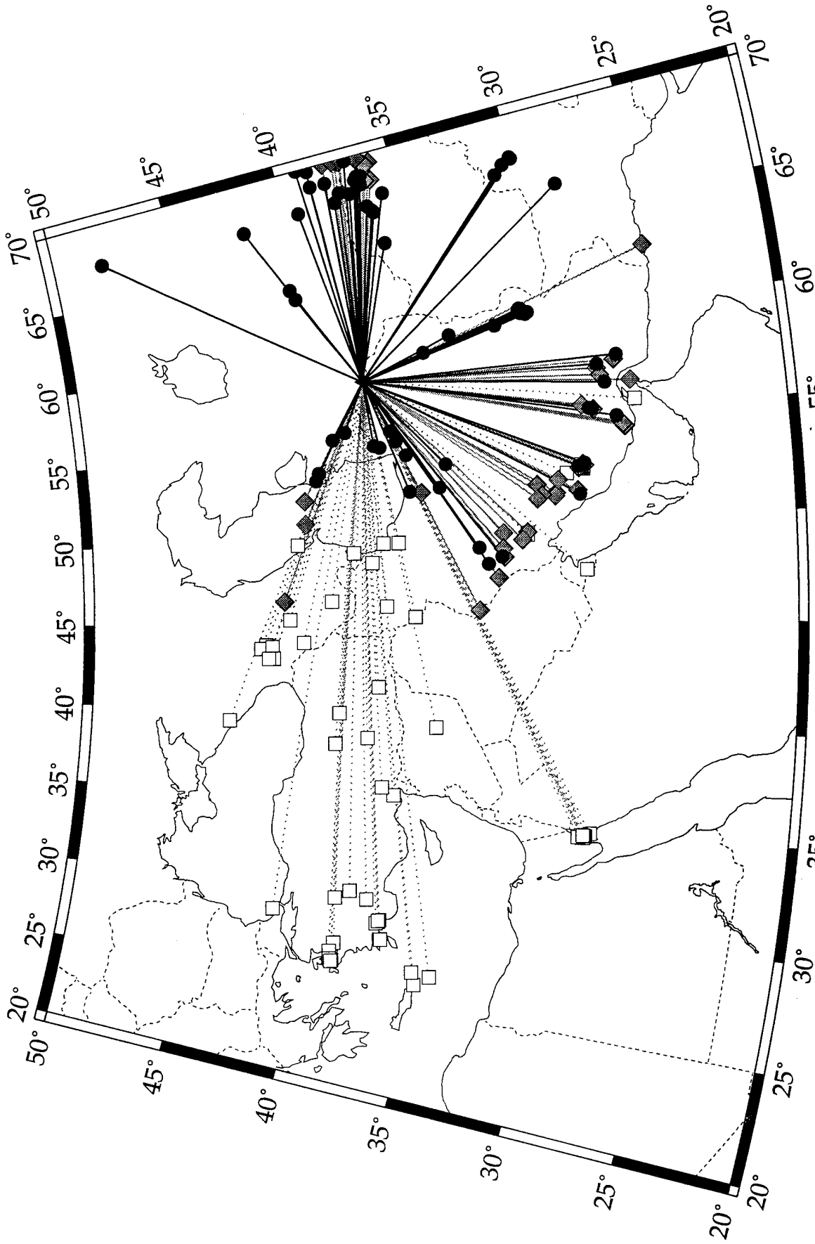
Figure C1: Map showing the efficiency of Lg wave raypaths at station ABKT.
