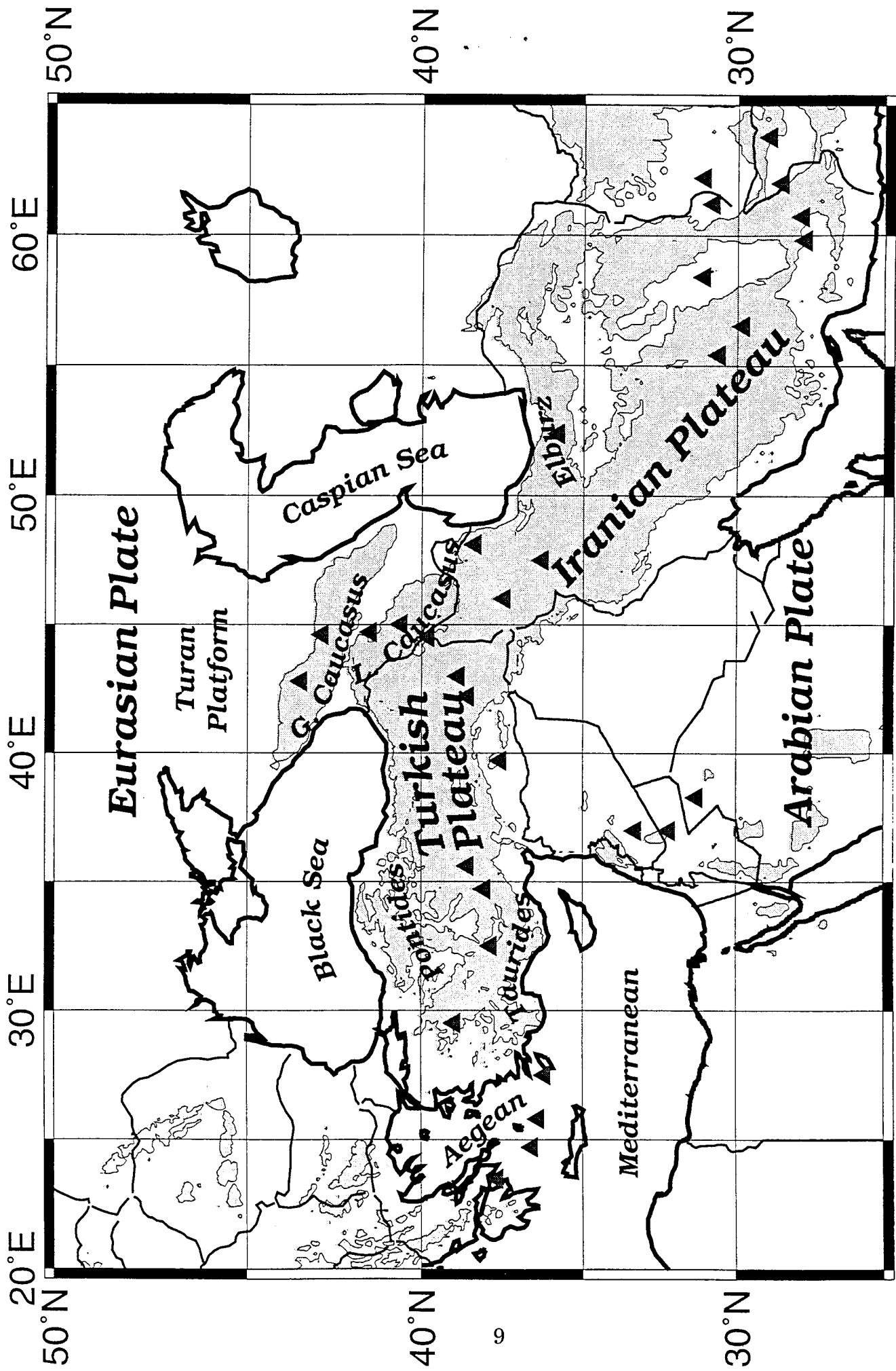
Figure 2: Location map for the Middle East. Shaded regions indicate regions over 1 km elevation.
