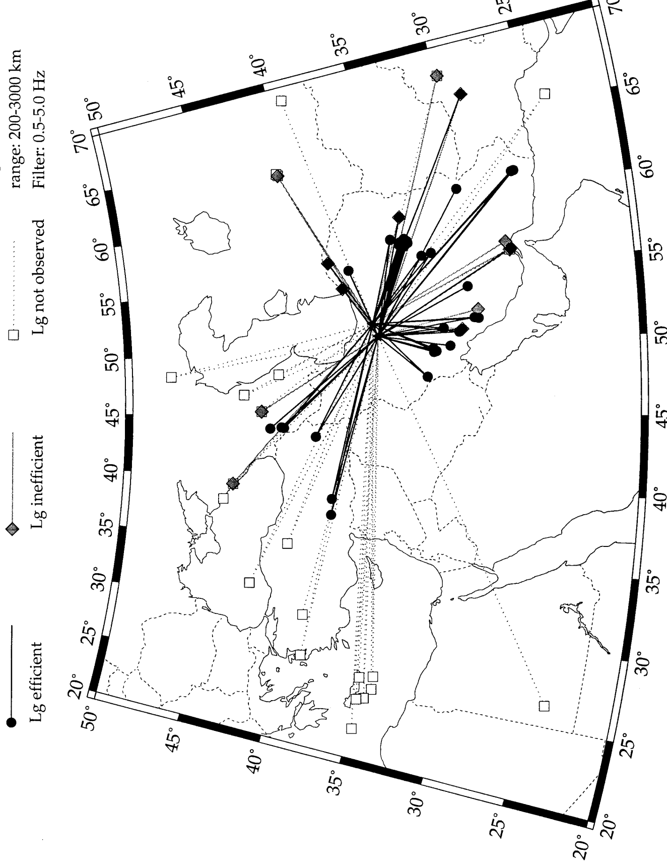
Figure C5: Map showing the efficiency of Lg wave raypaths at ILPA stations. 54
