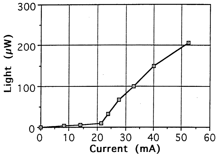
Figure 3. Light vs. current for the 10- \mu m-diameter, 725-nm-emitting VCSEL.
