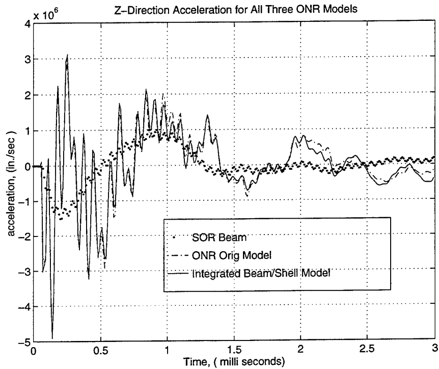
Figure 62. Whipping Motion Comparison At Deep Frame Location
