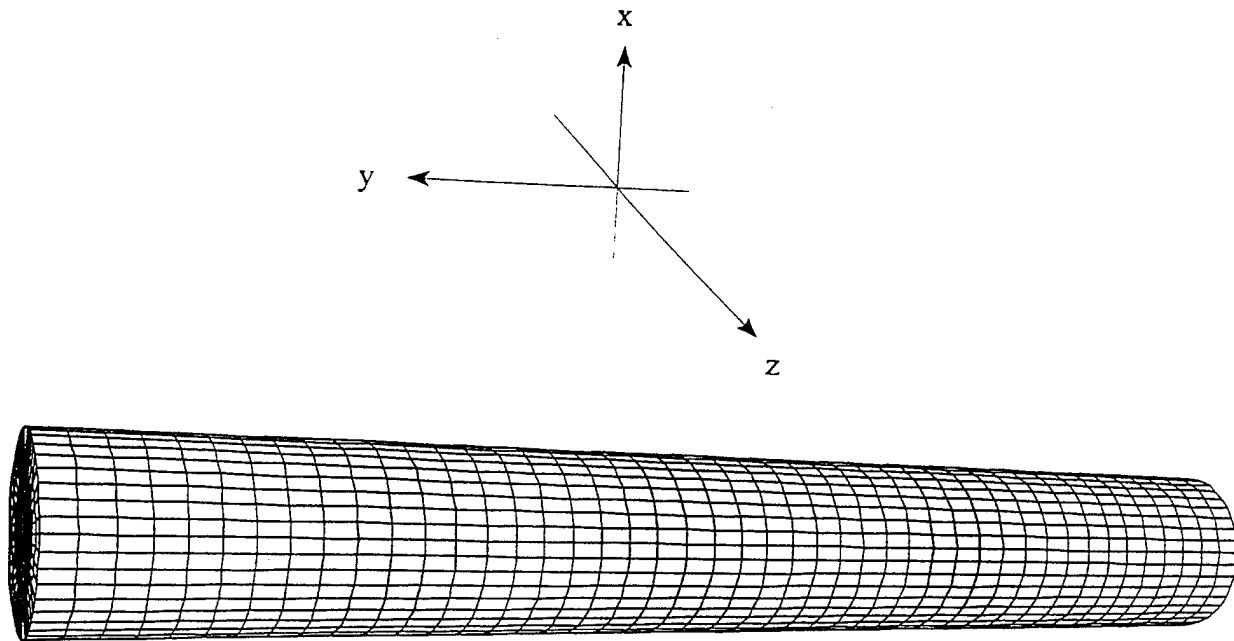
Figure 34. Orthotropically Smeared Model of ONR Stiffened Cylinder
