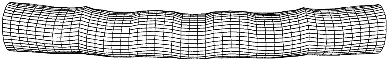
Figure 46b) Orthotropically Smeared ONR Cylinder at 0.5 msec
