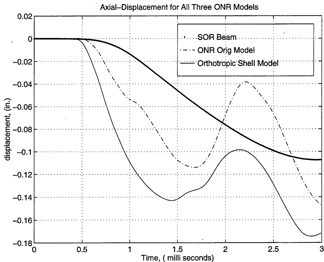
Figure 47. Axial Displacement Comparison at Left Endplate
