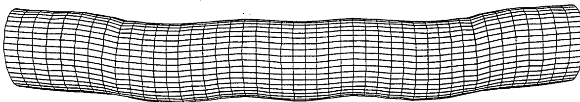
Figure 35d) State time of 2.0 msec
