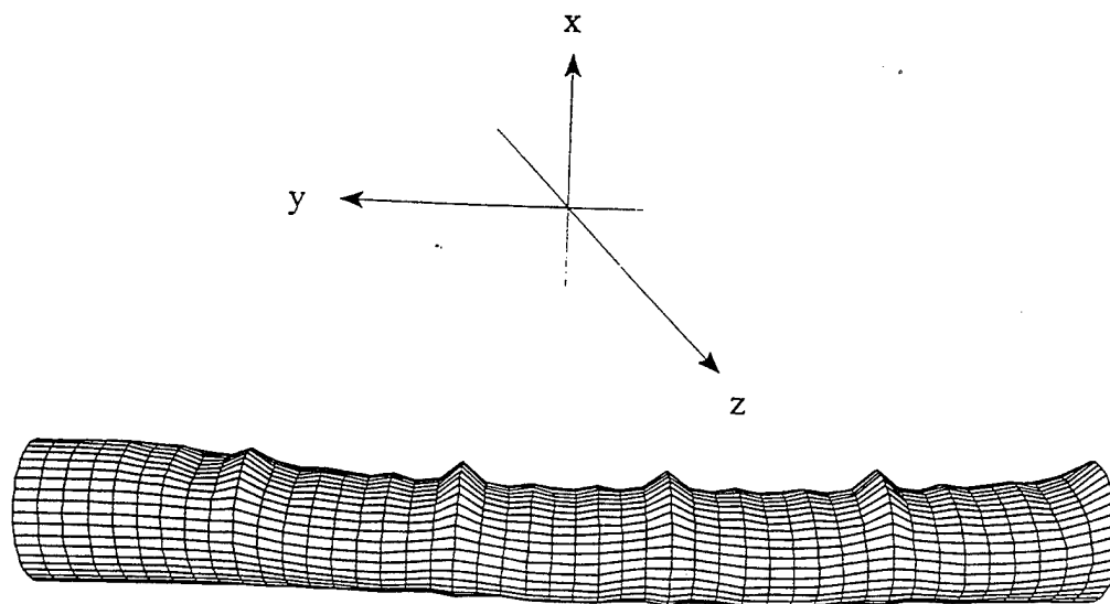
Figure 56a) ONR Stiffened Cylinder at 0.5 msec
