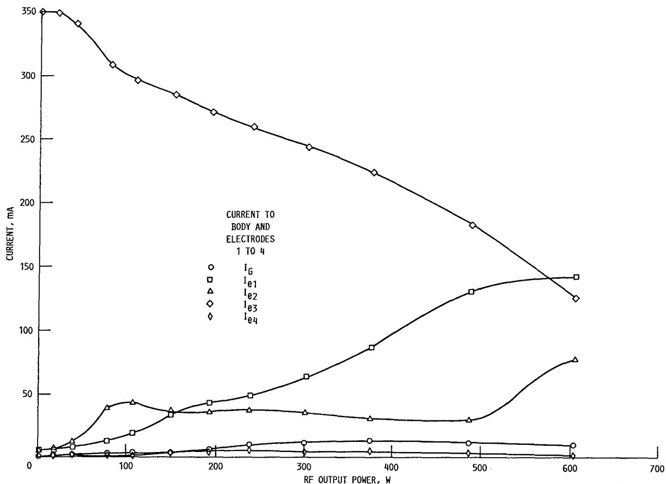
Figure 15.—Four-stage collector current distribution as function of RF output power at 8.0 GHz.
