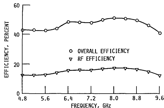
Figure 9.—Overall and RF efficiencies as functions of frequency at saturation.
