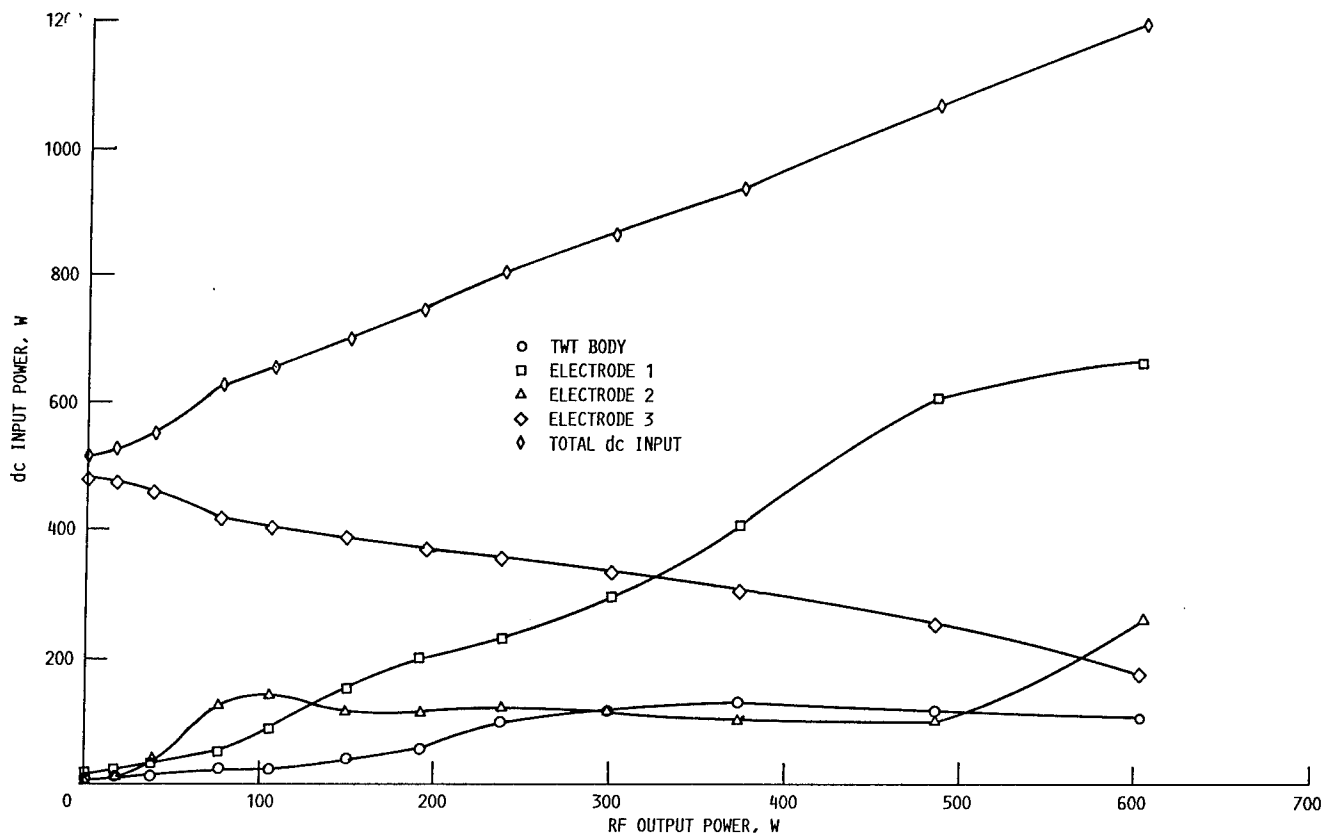
Figure 16.—Direct current input power per electrode in four-stage collector as function of RF output power at 8.0 GHz.
