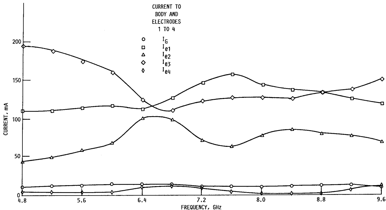
Figure 11.—Four-stage collector electrode current distribution as function of frequency at saturation.
