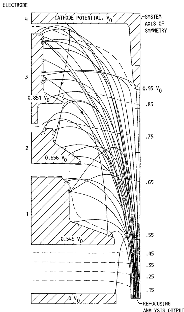
Figure 1.—Active geometry and trajectories of primary- and secondary-electron-emission charges in four-stage, 2.4-cm-diameter collector. TWT operating at saturation at 8.4 GHz in low mode.
