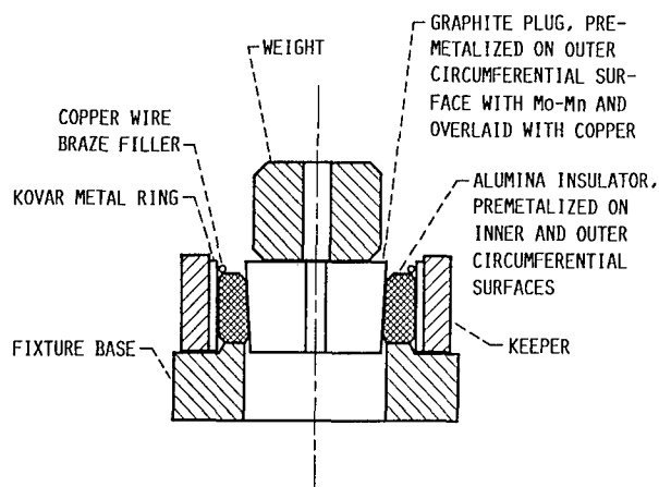
Figure 3.—Typical collector electrode module with fixturing prior to dry hydrogen brazing with copper braze filler metal.
