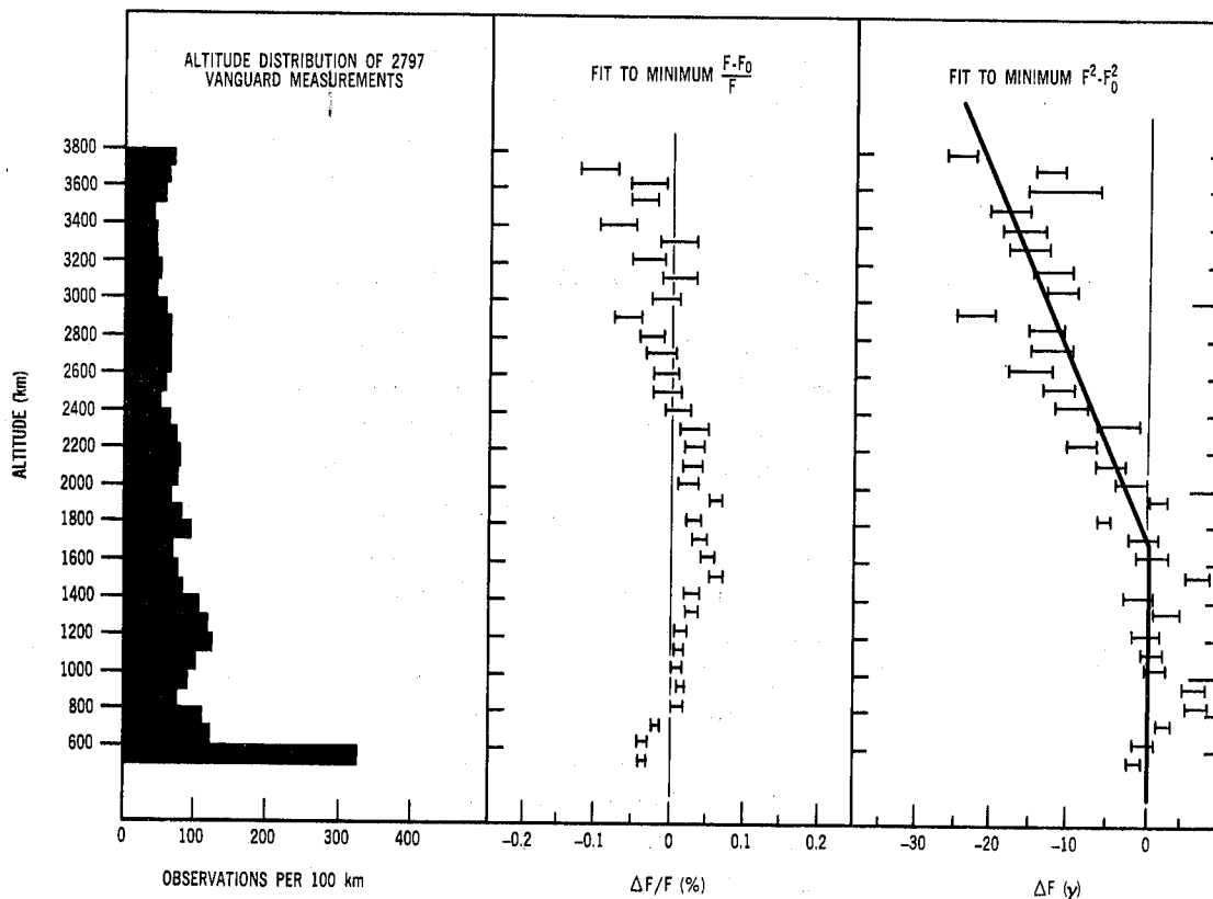
Figure 4— Average residuals of Vanguard III data relative to two different, n = m = 7 , spherical harmonic reference fields as a function of altitude. Error bars show the standard errors of the mean residuals.
