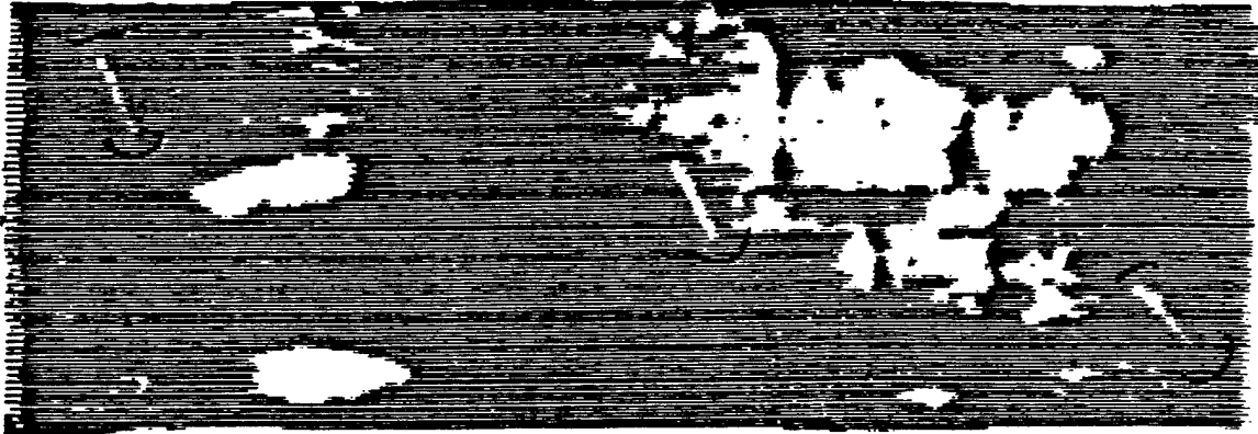
Figure 44. C-scan of PDA/6-FDA/Celion 12000 laminate.
