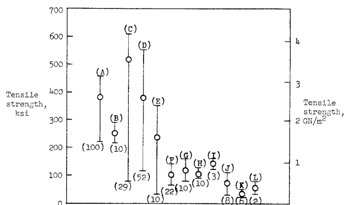
Figure 5.- Average tensile strength of all filaments tested. Gage length, 1 inch ( 2.54\ \text{cm} ). Letters in parentheses indicate filament type. Numbers in parentheses indicate number of tests upon which each point is based.
