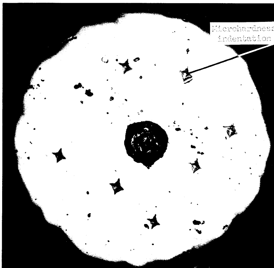
L-65-7936 Figure 18.- Photomicrograph of polished cross section of boron filament C showing microhardness indentations. Diameter, 0.0046 inch (0.117 mm). Indentations made with a 0.1-kgf (0.98-N) load on a 136^\circ (2.38-rad) diamond pyramid.
