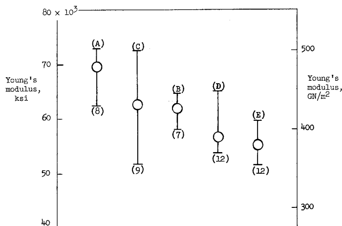
Figure 8.- Average Young's moduli for halide-process boron filaments. Gage length, 10 inches (25.4 cm). Letters in parentheses indicate filament type. Numbers in parentheses indicate number of tests upon which each point is based.
