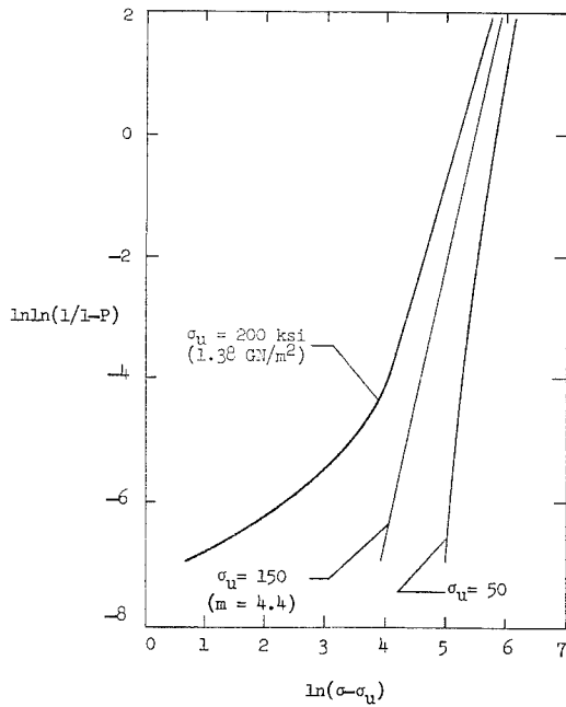
Figure 30.- Plot of Weibull's distribution function parameters for 120 tensile failures of boron filament A, reel 1. Gage length, 1 inch (2.54 cm).
