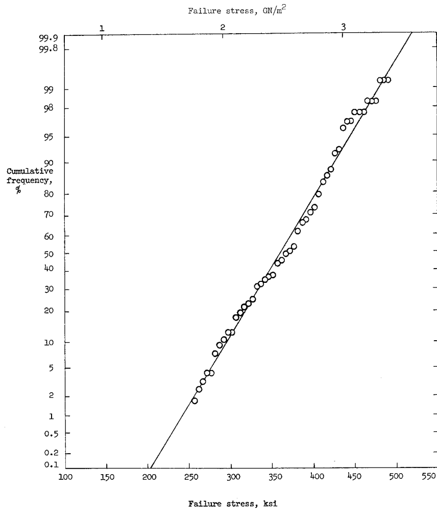
Figure 29.- Cumulative failure frequency plot on normal probability scale for boron filament A, reel no. 1. Gage length, 1 inch (2.54 cm).
