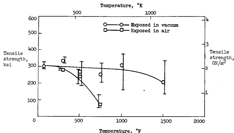
Figure 14.- Effect of elevated-temperature exposure on tensile strength of boron filament A. Exposure time, 15 minutes. Gage length, 10 inches (25.4 cm). Each point represents 10 tests.
