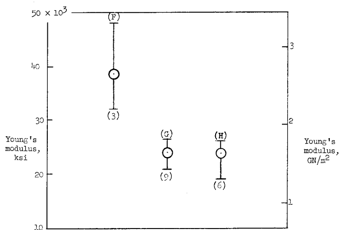
Figure 10.- Average Young's moduli for organometallic-process boron filaments. Gage length, 10 inches (25.4 cm). Letters in parentheses indicate filament type. Numbers in parentheses indicate number of tests upon which each point is based.
