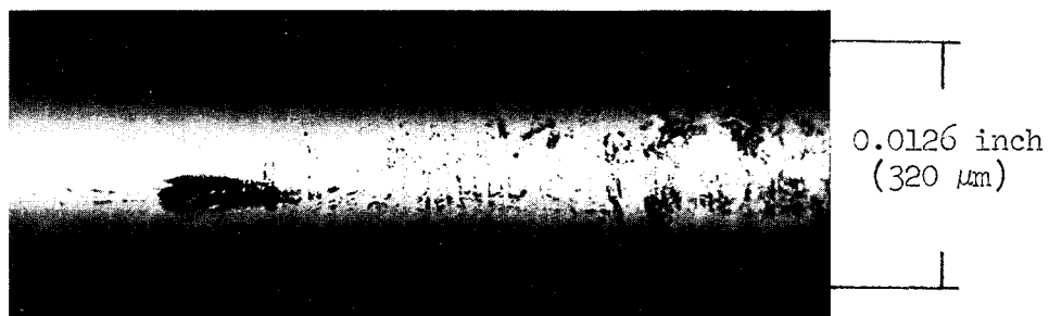
(a) Boron filament; diameter, 0.0126 inch (320 \mu\text{m} ).
