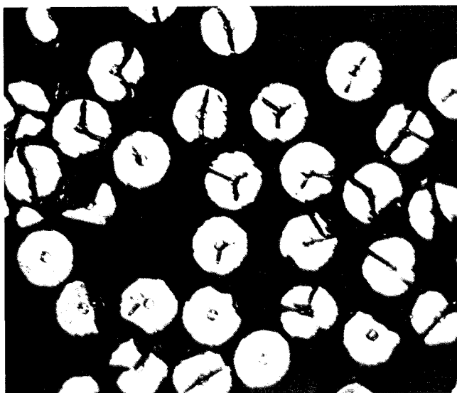
L-65-7942 Figure 24.- Photomicrograph showing typical polished cross sections of halide-process boron filament. Diameter, 0.0046 inch (0.117 mm).
