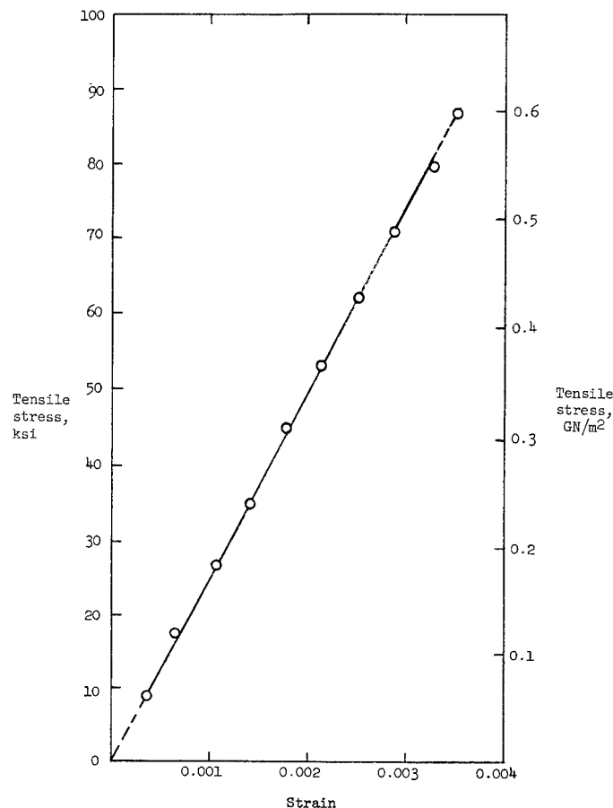
Figure 9.- Typical stress-strain curve for boron filament H. Gage length, 10 inches (25.4 cm). Diameter 0.0038 inch (97 \mu m). Dashed segments of curve represent extrapolation of experimental data.
