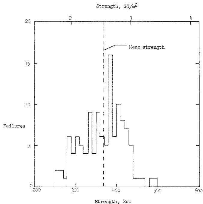
Figure 28.- Frequency histogram of tensile failures for boron filament A, reel 1. Frequency based on 1-inch (2.54-cm) gage length, 10 ksi (0.069 \text{GN/m}^2 ) stress intervals, and 120 tests.
