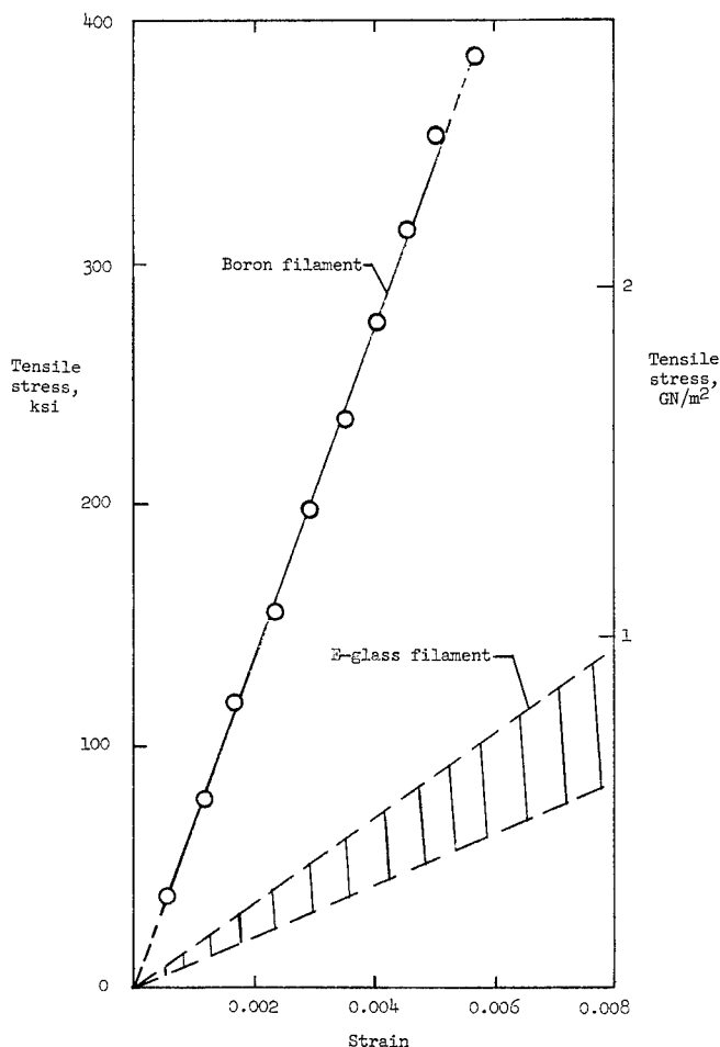
Figure 7.- Typical stress-strain curve for boron filament A. Gage length, 10 inches (25.4 cm). Diameter, 0.0018 inch (46 \mu m). Dashed segments of boron curve represent extrapolations of experimental data.
