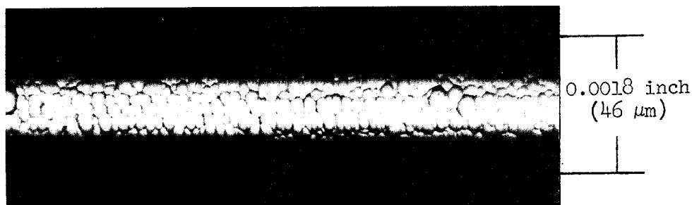
Figure 19.- Typical halide-reduction-process filament surface; diameter, 0.0018 inch (46 μm).
