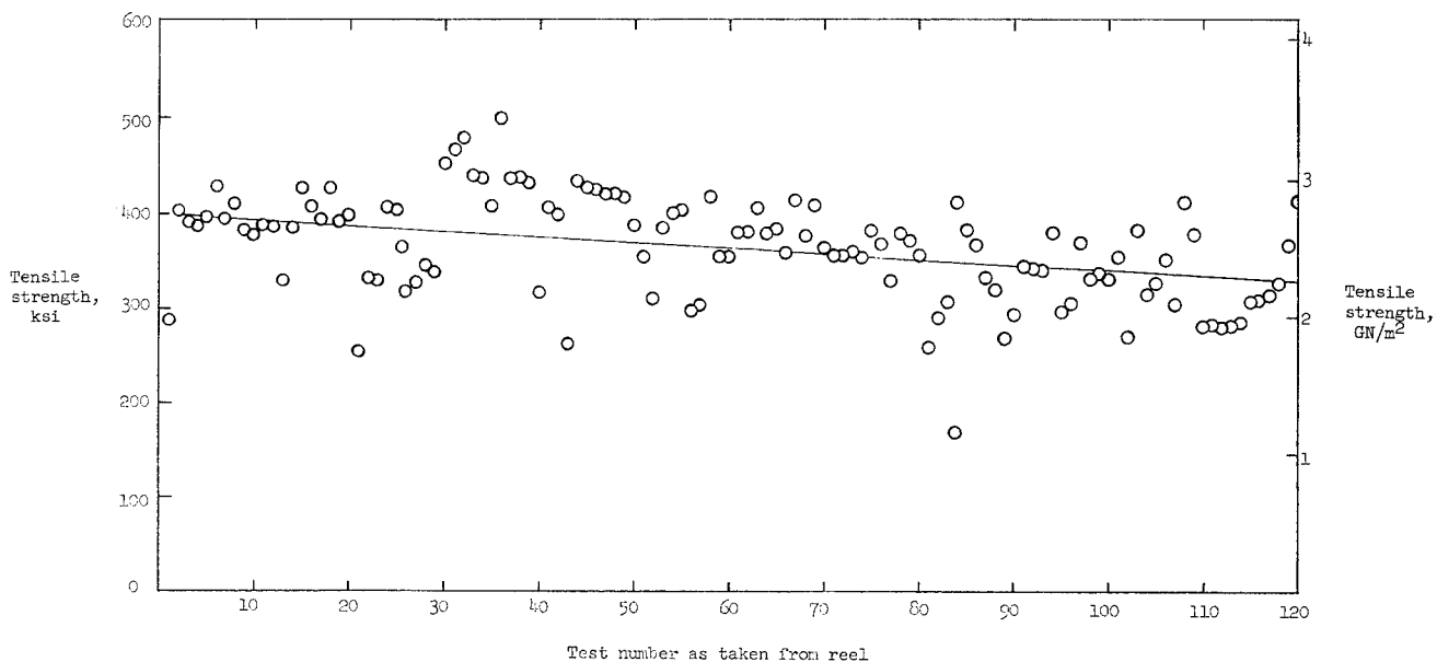
Figure 32.- Tensile strength of boron filament A. Reel 1; 120 tests of 1-inch (2.54-cm) gage-length specimens plotted consecutively as removed from the reel.
