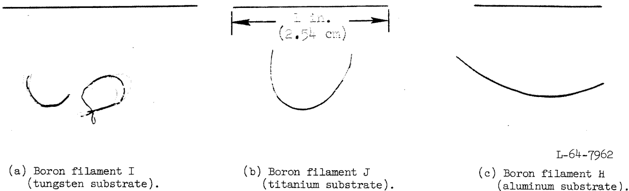
Figure 16.- Effect of elevated-temperature exposure on physical appearance of filaments made from diborane. Straight specimens exposed 30 minutes at 750° F (672° K), and 1 \times 10^{-5} torr ( 1.3 \text{ mN/m}^2 ) pressure; curved specimens exposed 30 minutes at 1000° F (811° K), and 1 \times 10^{-5} torr ( 1.3 \text{ mN/m}^2 ) pressure.
