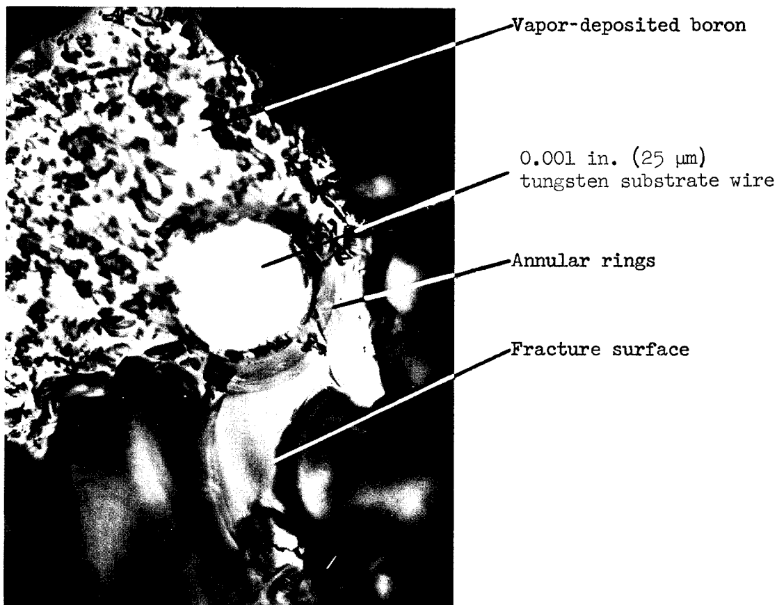
Figure 26.- Photomicrograph of boron filament F cross section showing fracture surfaces. L-65-7944 X1000.
