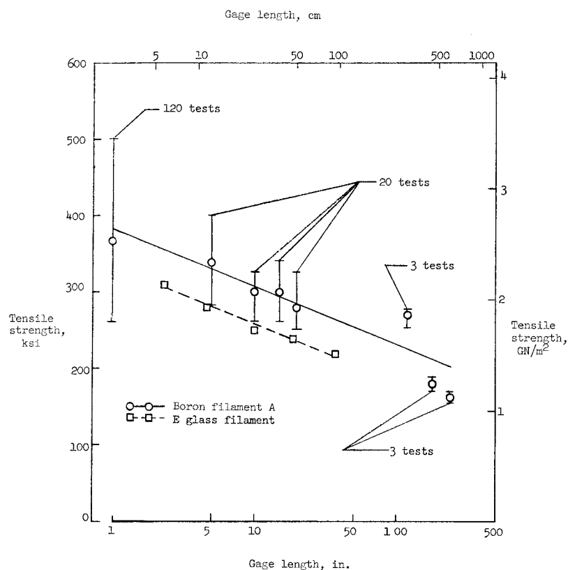
Figure 6.- Effect of gage length on tensile strength of boron filament A. Filament diameter, 0.0018 inch (46 \mu\text{m} ). Similar data for E-glass filament shown for comparison.
