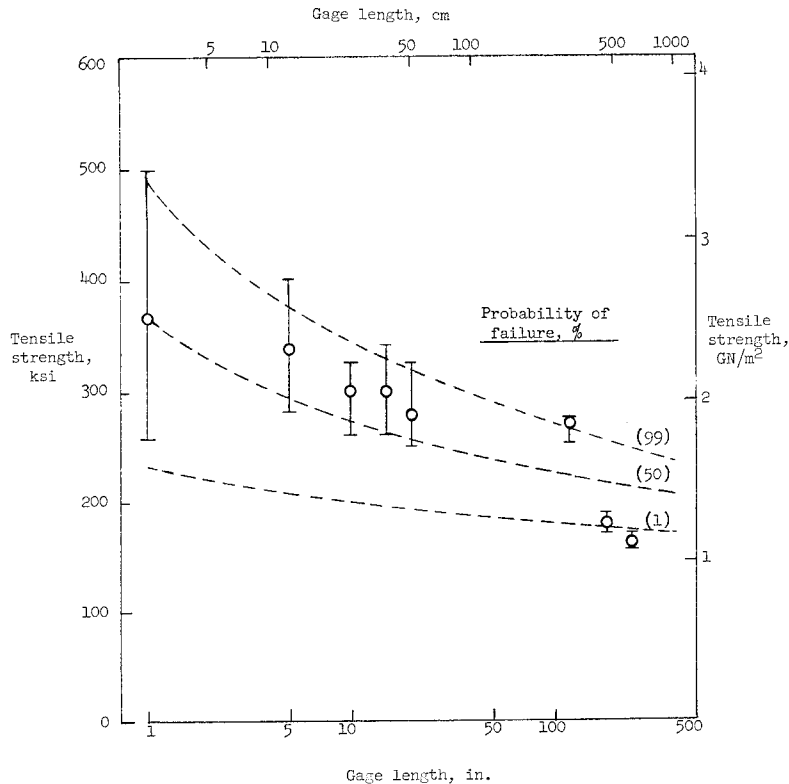
Figure 31.- Tensile strength of boron filament A, reel 1 as a function of gage length. Dashed lines represent constant-probability curves generated from an analysis of the distribution of 120 test breaks of 1-inch (2.54-cm) gage-length specimens based on the Weibull distribution function.
