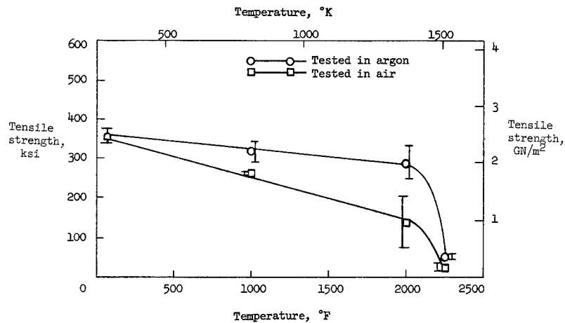
Figure 12.- Effect of temperature on tensile strength of boron filament C. Specimens held at temperature for 60 seconds before load was applied. Each point represents 2 tests. Gage length, 10 inches (25.4 cm).
