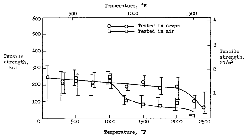
Figure 13.- Effect of temperature on tensile strength of boron filament E. Specimens held at temperature for 60 seconds before load was applied. Each point represents 5 tests. Gage length, 10 inches (25.4 cm).
