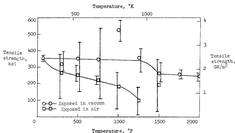
Figure 15.- Effect of elevated-temperature exposure on tensile strength of boron filament C. Exposure time, 15 minutes. Gage length, 10 inches (25.4 cm). Each point represents 5 tests.
