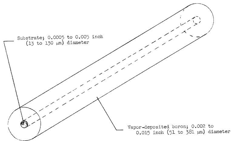
Figure 1.- Schematic representation of a boron filament.
