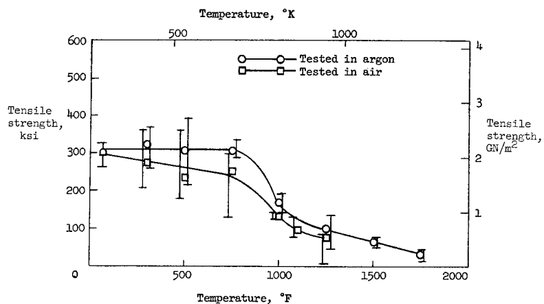
Figure 11.- Effect of temperature on tensile strength of boron filament A. Specimens held at temperature for 60 seconds before load was applied. Each point represents 10 tests. Gage length, 10 inches (25.4 cm).
