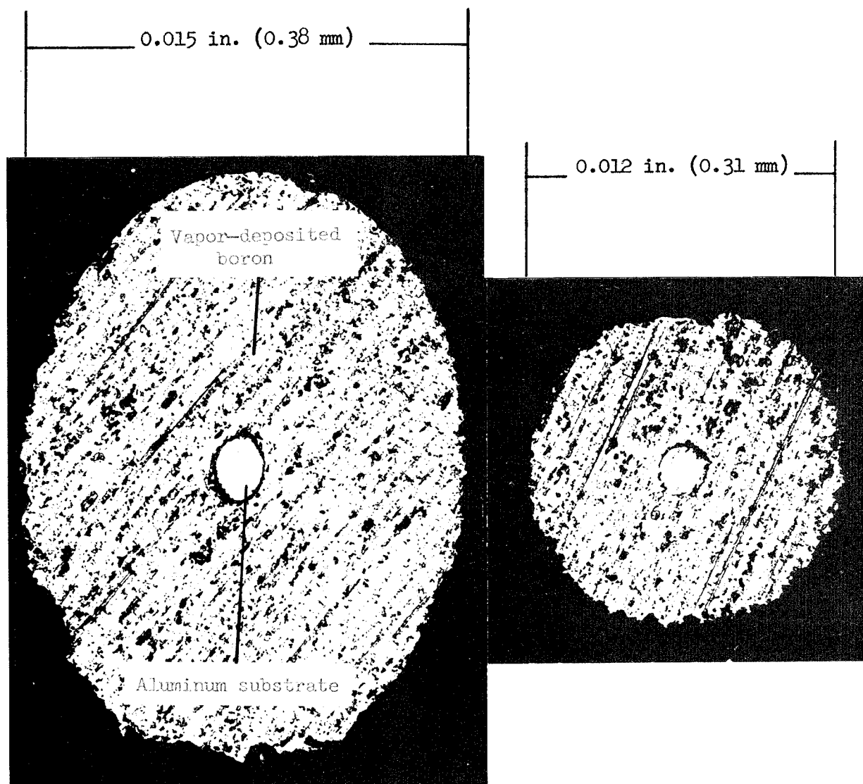
L-65-7943 Figure 25.- Cross sections of boron filament H made from diborane on aluminum substrate wire.
