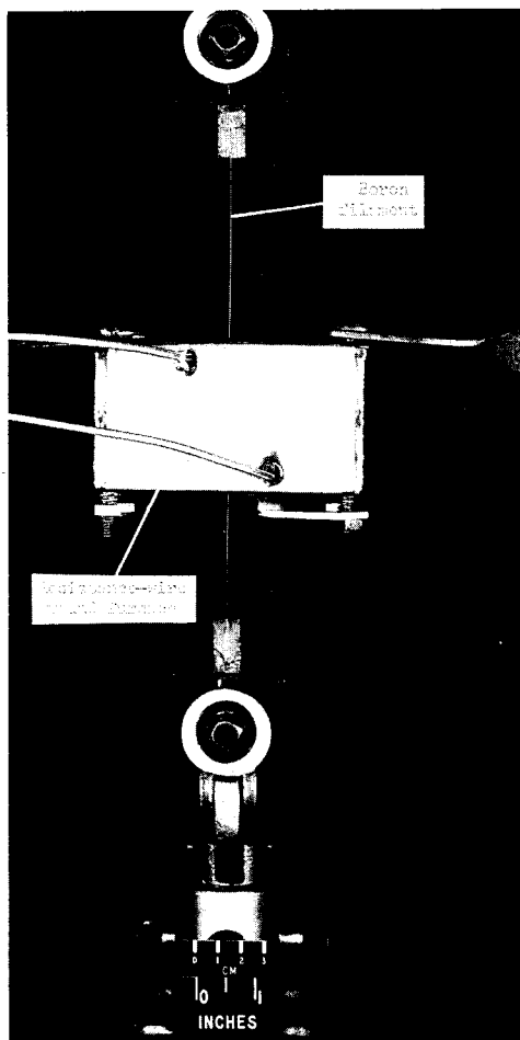
Figure 4.- Apparatus for elevated-temperature tensile testing of boron filaments.
