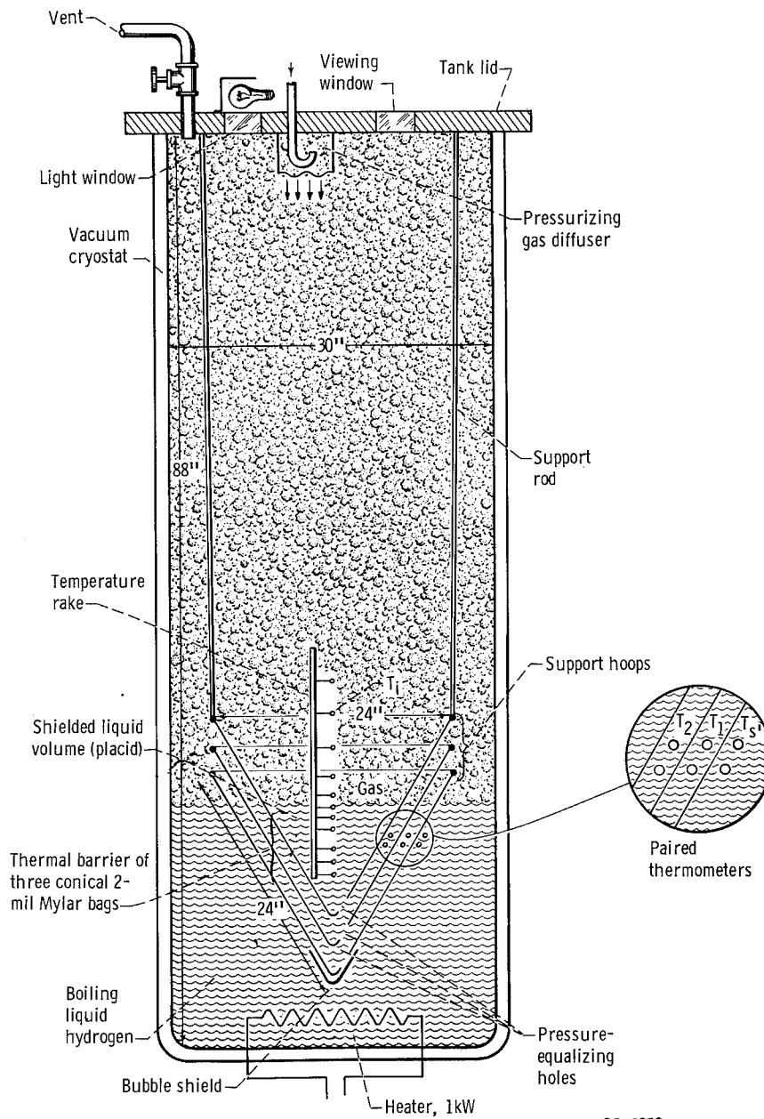
(a) Schematic drawing of test setup.
