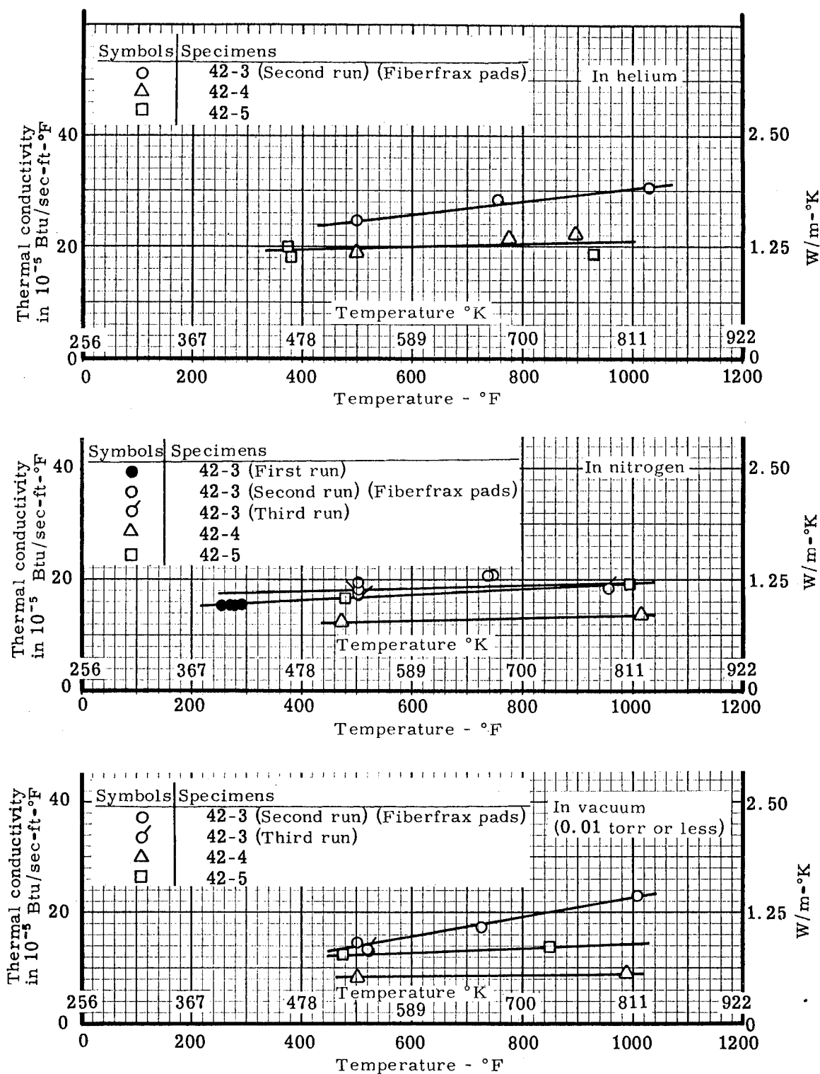
Figure 17. The thermal conductivity of phenolic-nylon char of 0.79 porosity (42 lb/ft³ virgin density) in vacuum, nitrogen and helium
