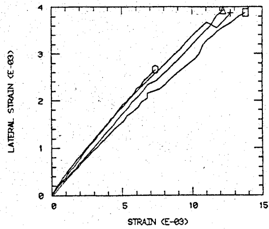
AS5/5245C, POISSONS, 100 C, DRY
