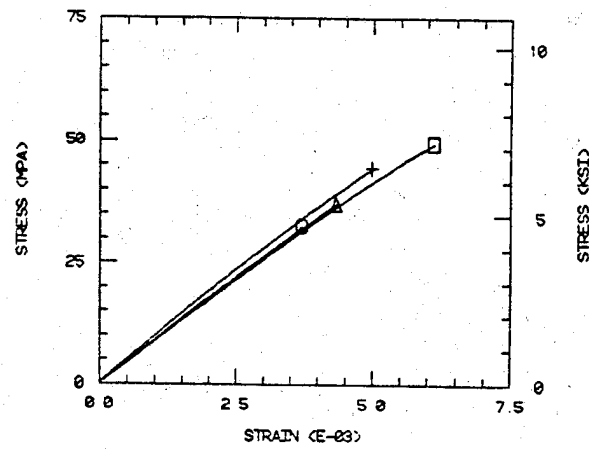
AS6/S245C, TRANSVERSE TEN, 121 C, DRY
