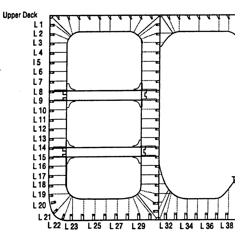
Figure 14. Midship Section
