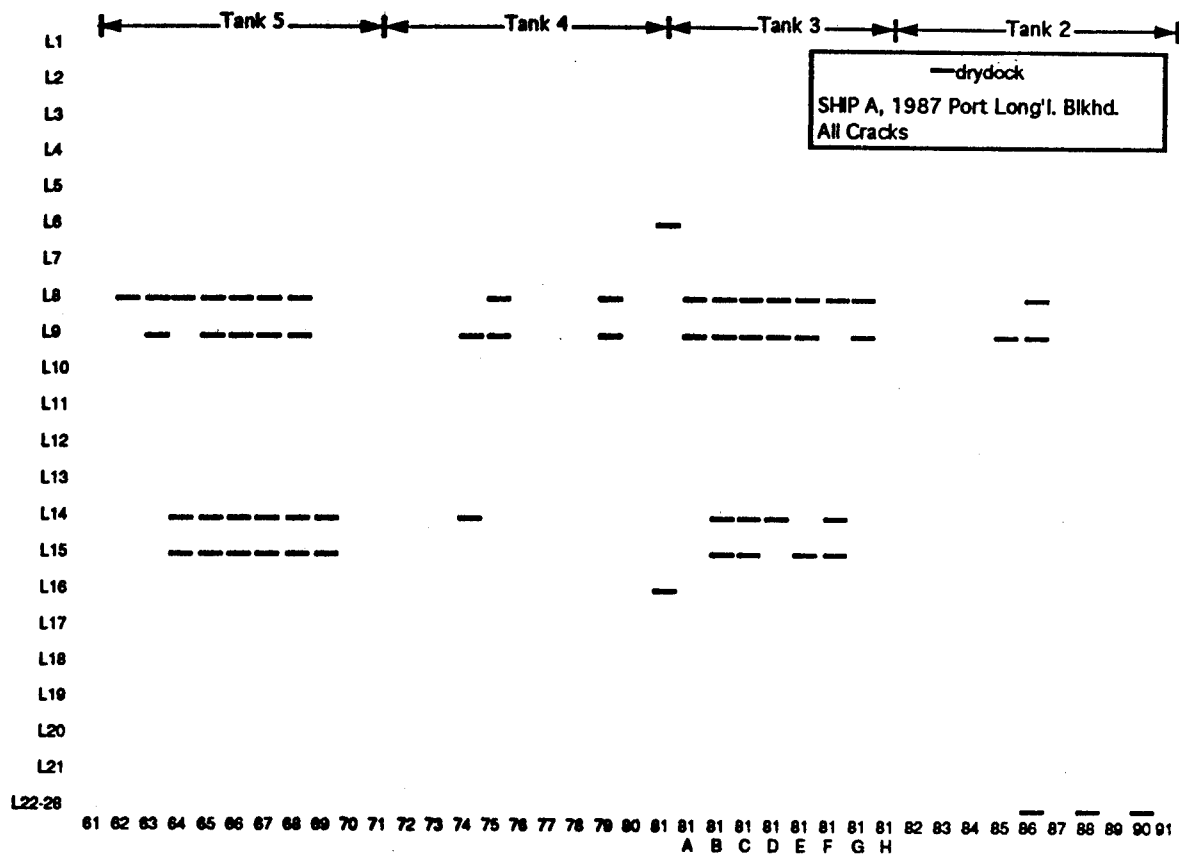
Figure C2a. Ship A 1987 Drydock Inspection, Port Longitudinal Bulkhead Cracks
