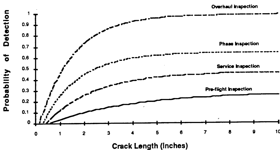
Figure 9. Probability of Detecting Cracks in Aircraft, after [Dinkeloo 1978].
