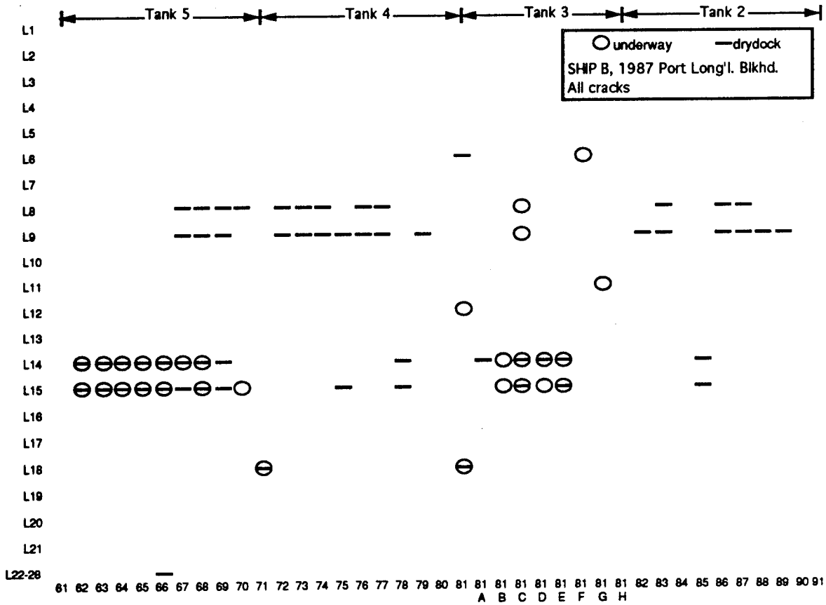
Figure 16a. Ship B 1987 Inspections, Port Longitudinal Bulkhead Cracks
