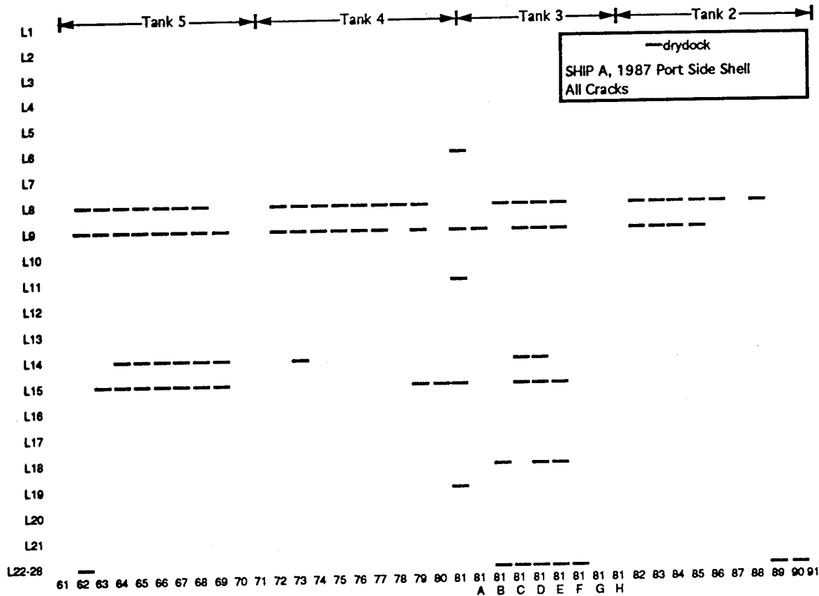
Figure C1a. Ship A 1987 Drydock Inspection, Port Side Shell Cracks
