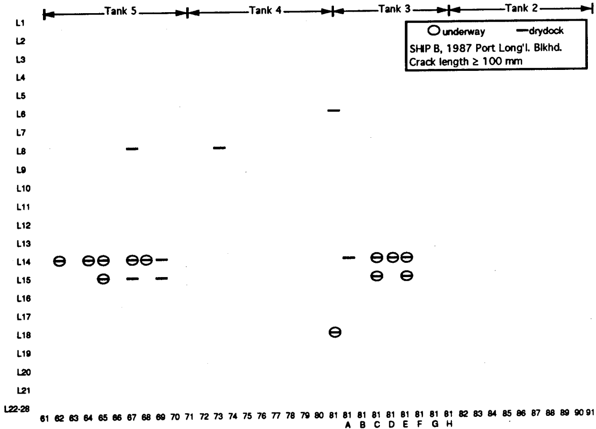
Figure 16b. Ship B 1987 Inspections, Port Longitudinal Bulkhead Cracks ≥ 100mm
