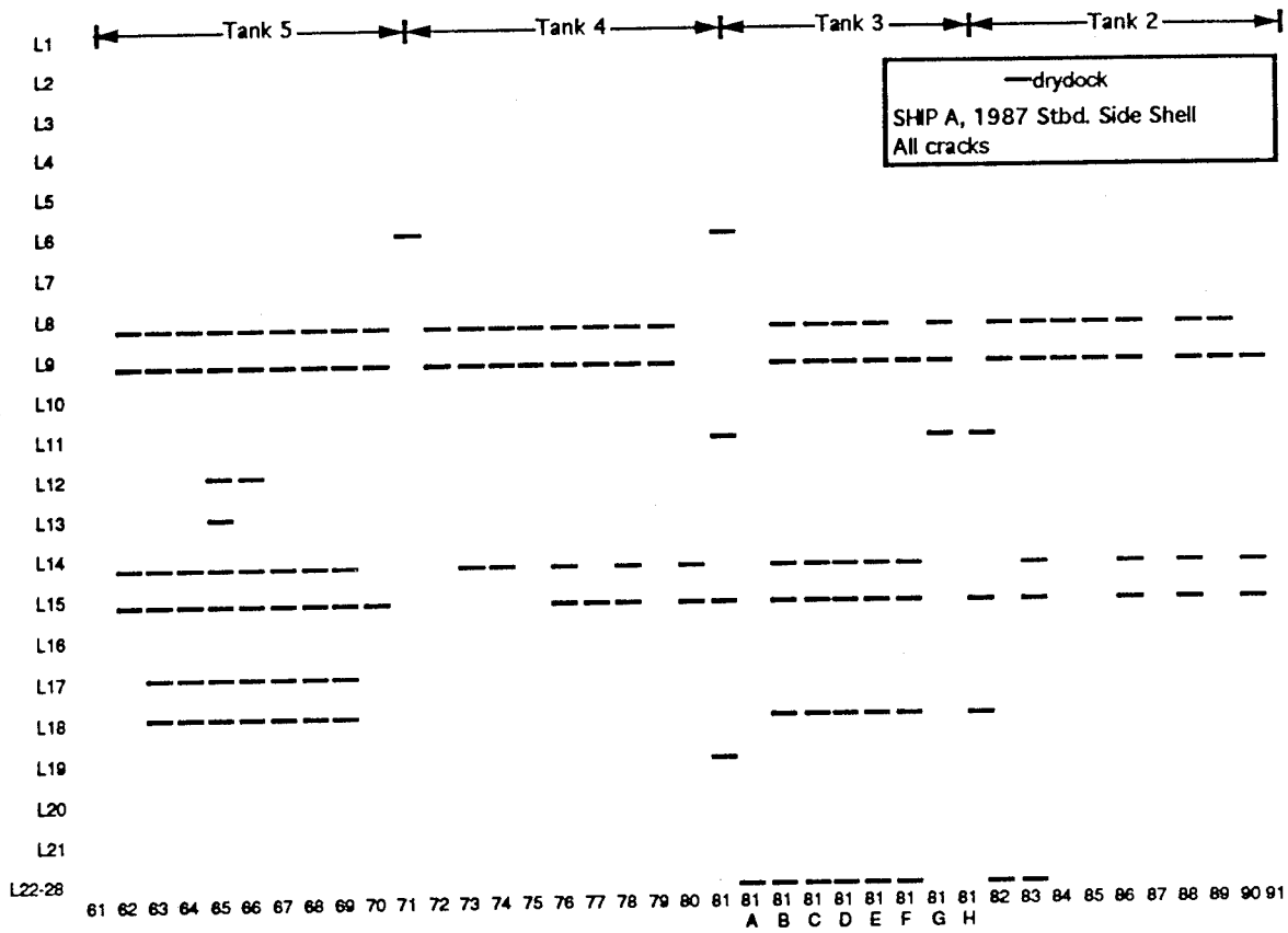
Figure C3a. Ship A 1987 Drydock Inspection, Starboard Side Shell Cracks
