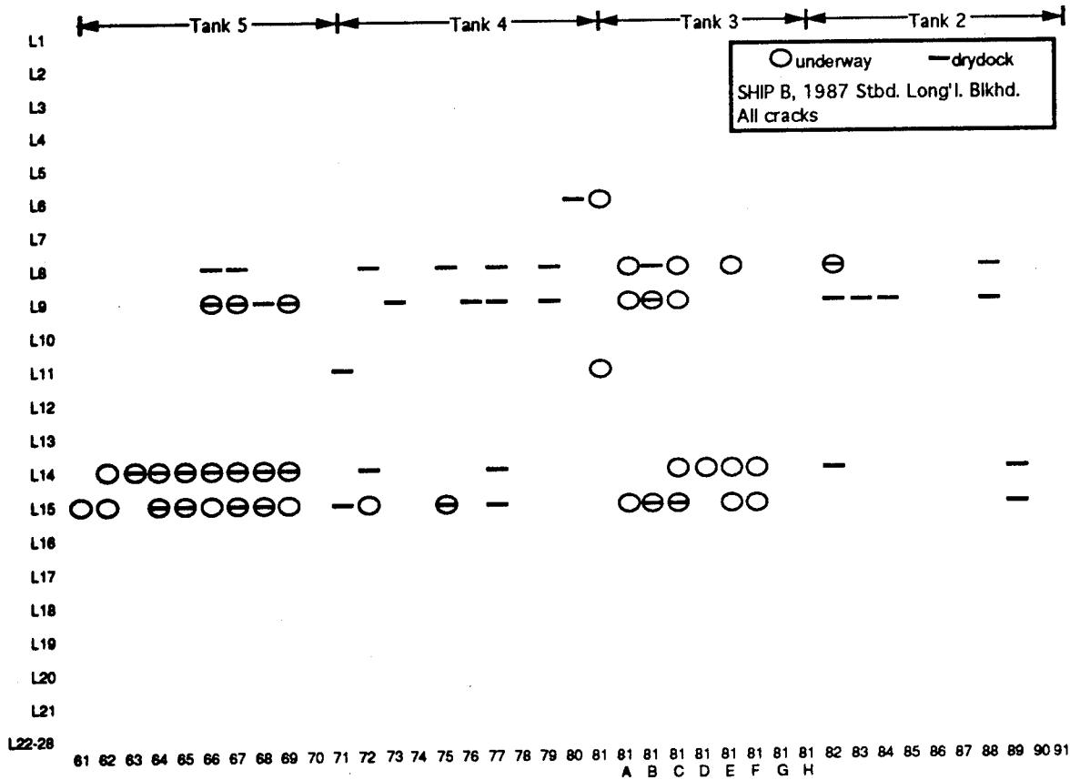
Figure 18a. Ship B 1987 Inspections, Stbd. Longitudinal Bulkhead Cracks
