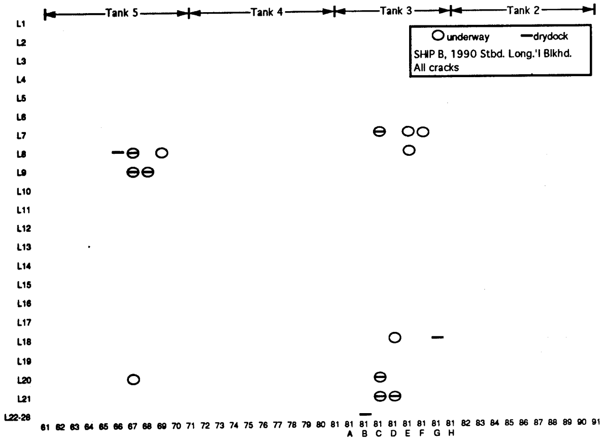
Figure 22a. Ship B 1990 Inspections, Starboard Longitudinal Bulkhead Cracks
