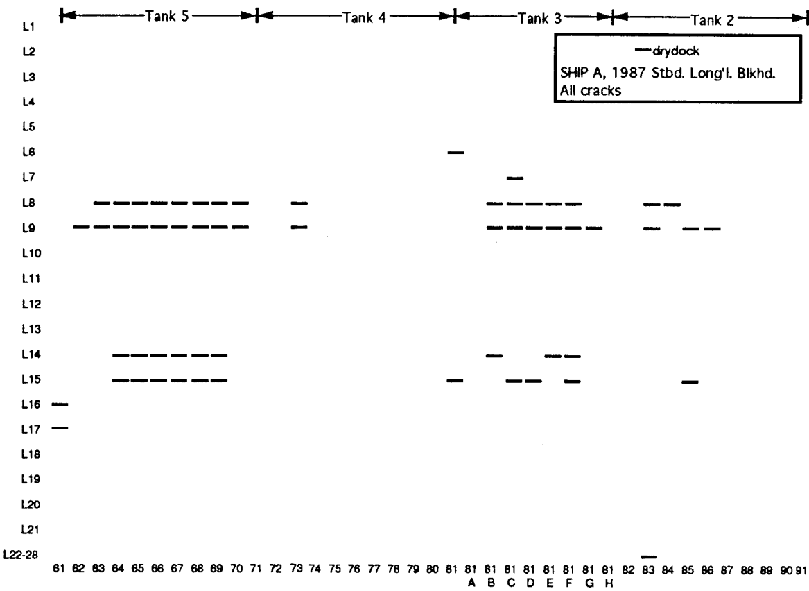
C4a. Ship A 1987 Drydock Inspection, Stbd. Longitudinal Bulkhead Cracks
