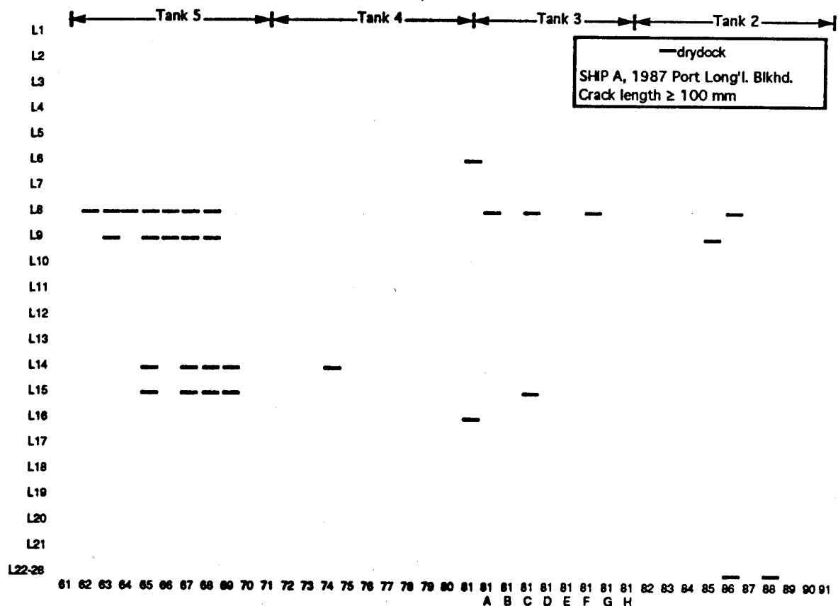
Figure C2b. Ship A 1987 Drydock Inspection, Port Long'l. Bulkhead Cracks \geq 100 mm
