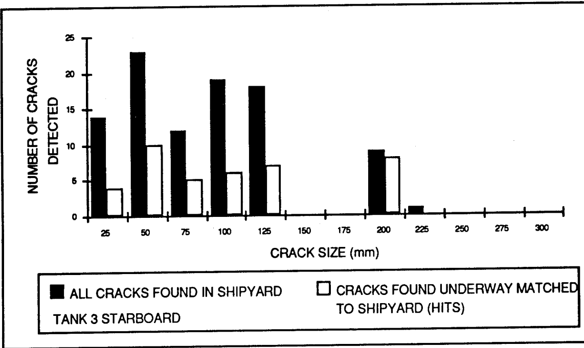
Figure 23. "Hits" and All Drydock Cracks, 1987 Inspection, Tank 3 Starboard
