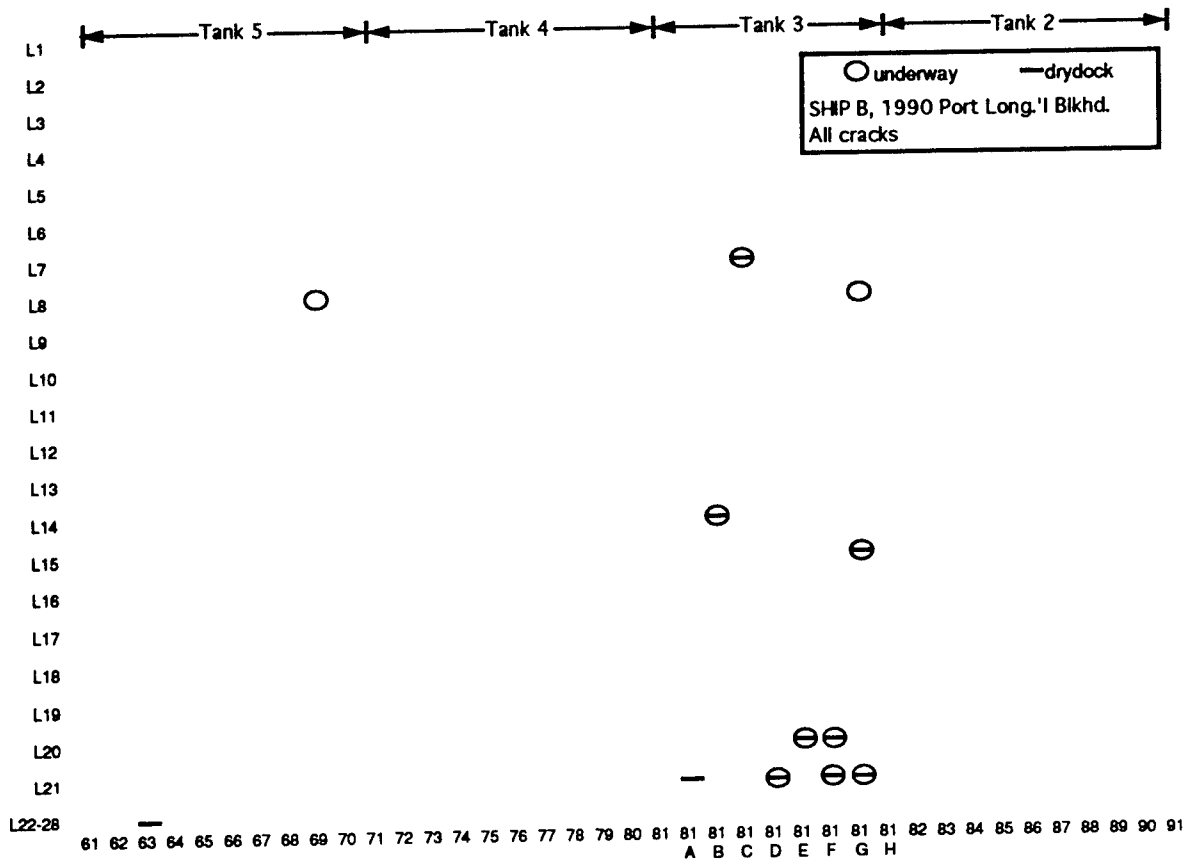
Figure 20a. Ship B 1990 Inspections, Port Longitudinal Bulkhead Cracks
