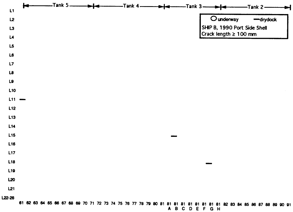
Figure 19b. Ship B 1990 Inspections, Port Side Shell Cracks \geq 100 mm
