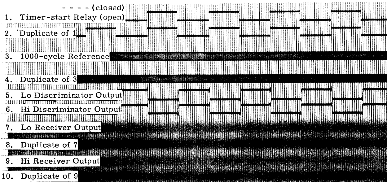
Fig. 7 -- Oscillograph Record of Preflyaround Test
