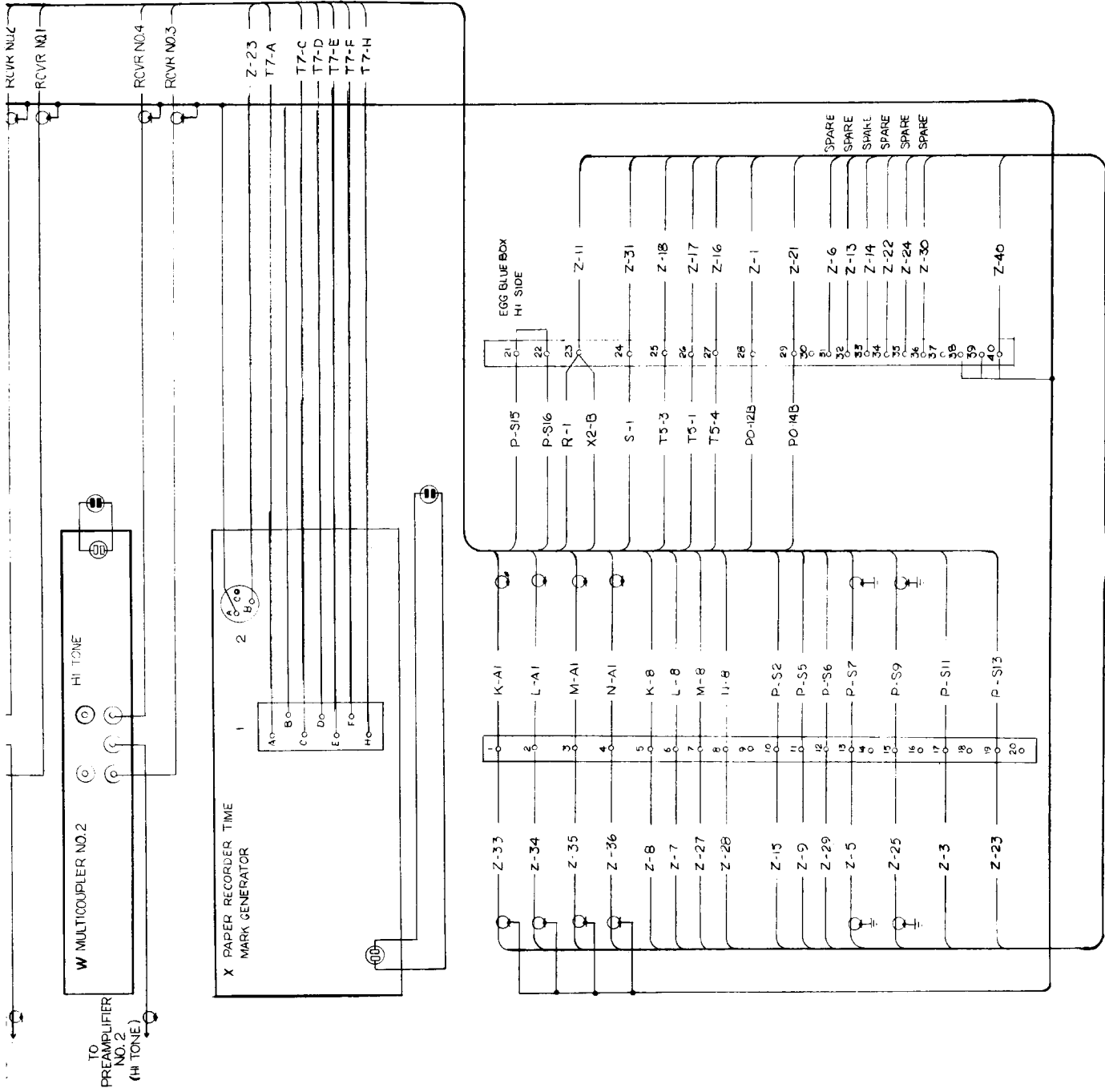
. 11 -- Wiring Diagram, Rack No. 2
