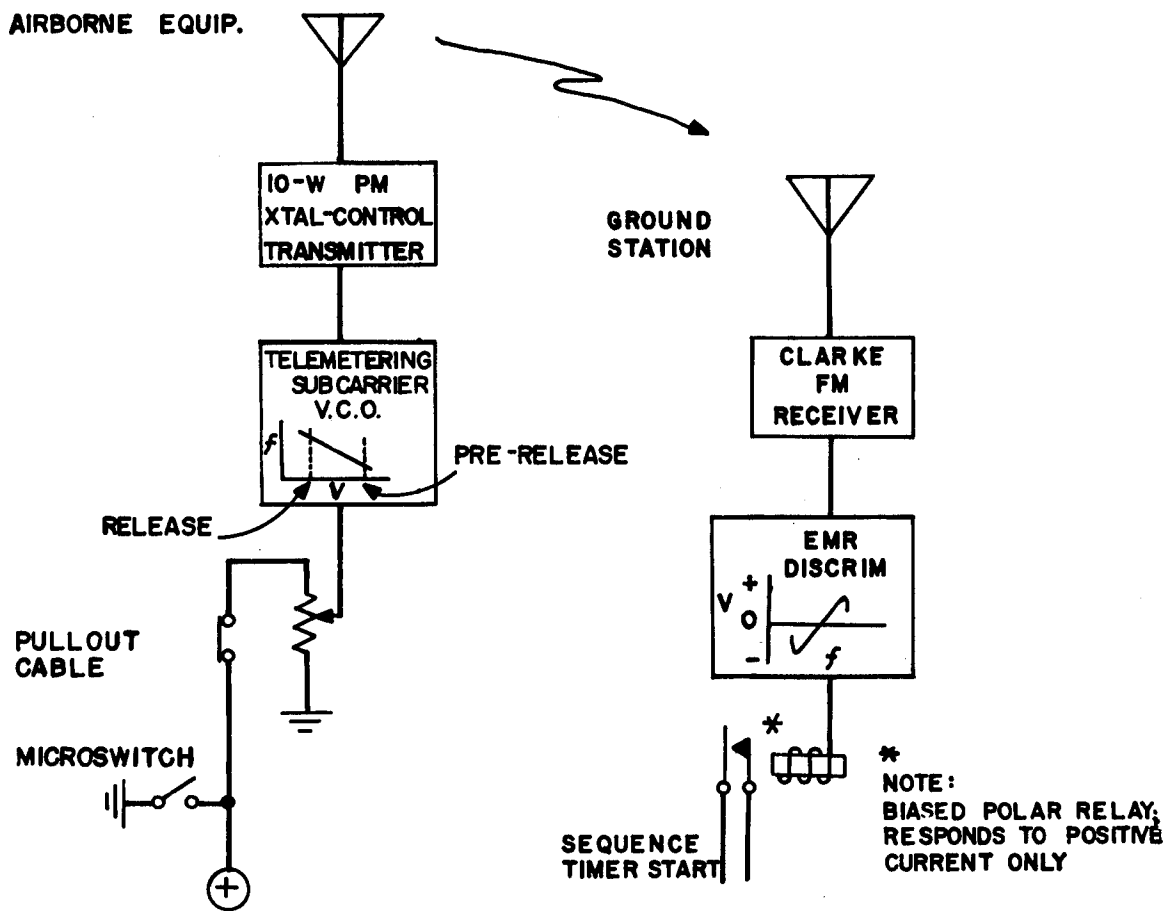
Fig. 4 -- Release Tone System, Basic Block Diagram
