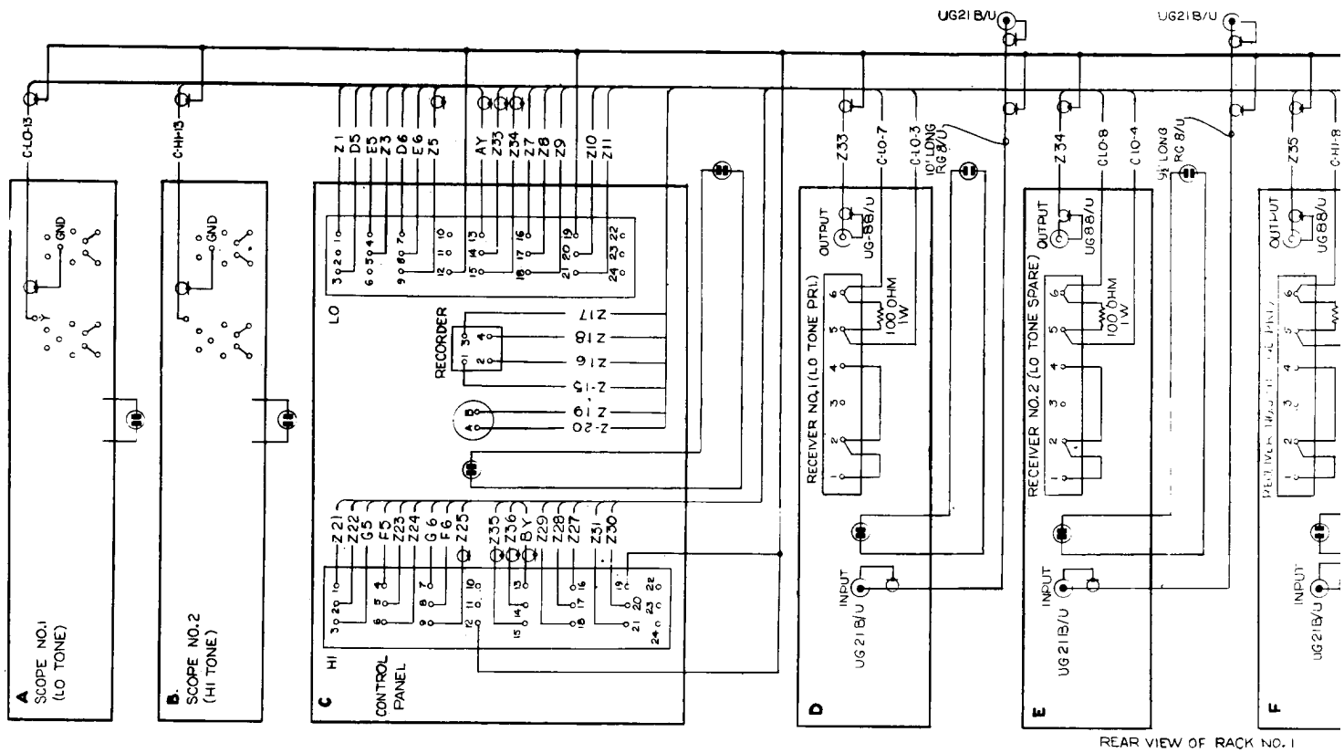
REAR VIEW OF RACK NO. 1
