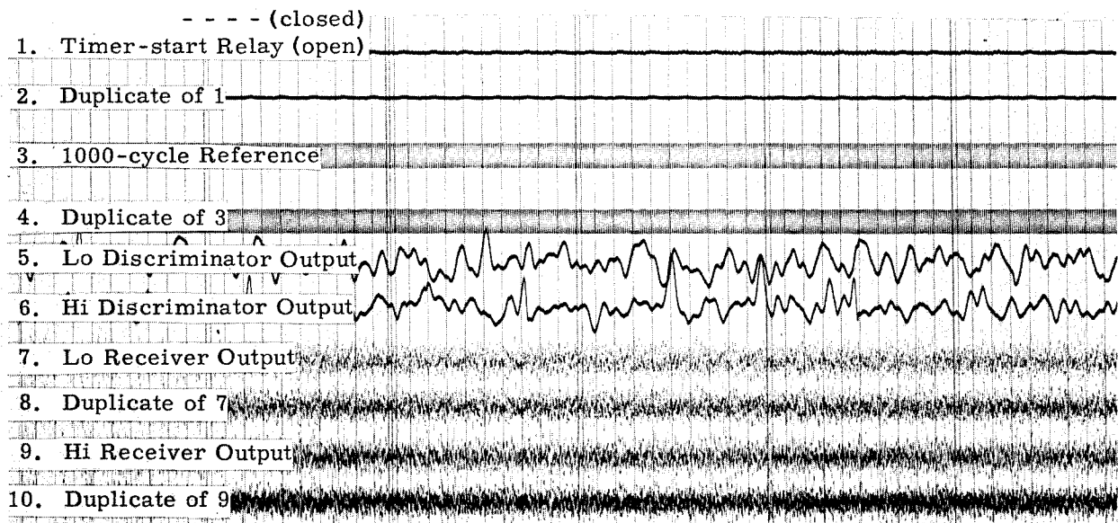
Fig. 6 -- Oscillograph Record of Noise Only
