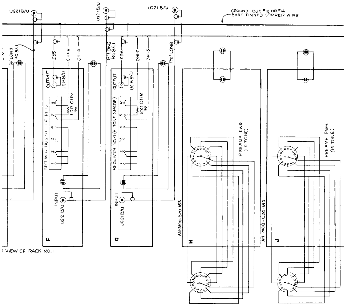
Fig. 10 -- Wiring Diagram, Rack No. 1
