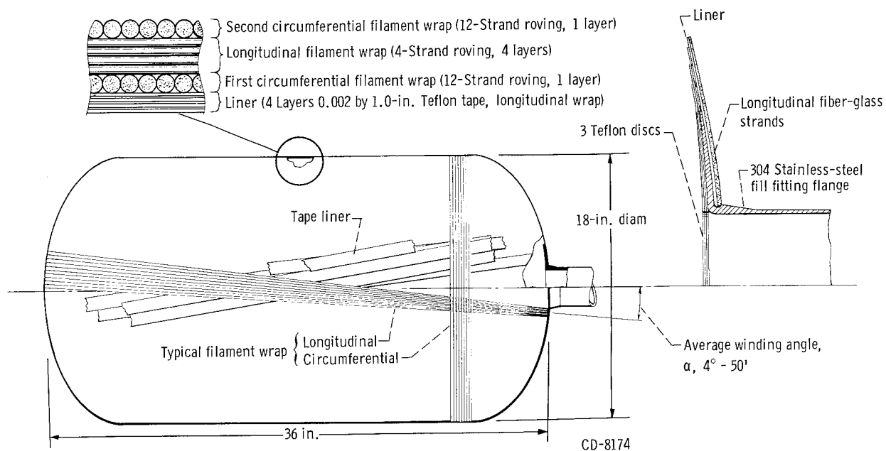
Figure 1. - Schematic of tank 1 with bonded Teflon tape liner.
