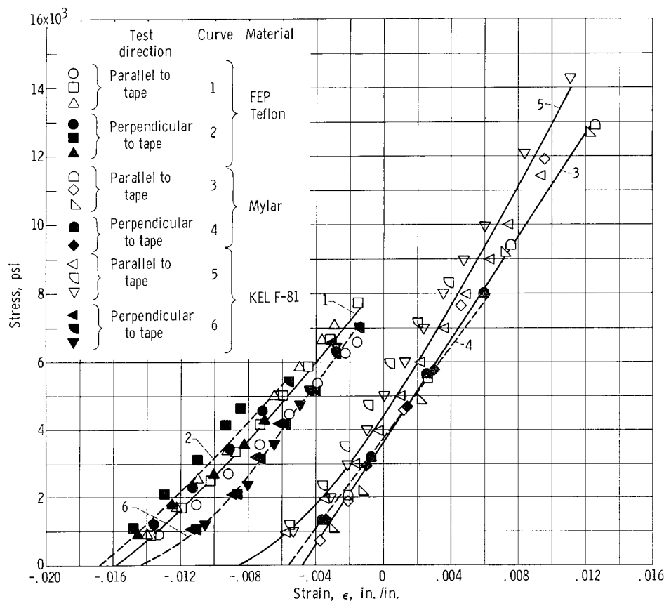
Figure 18. - Thermal shrinkage from room temperature and stress-strain at 76° K (-320° F) for plastic tape liner materials.
