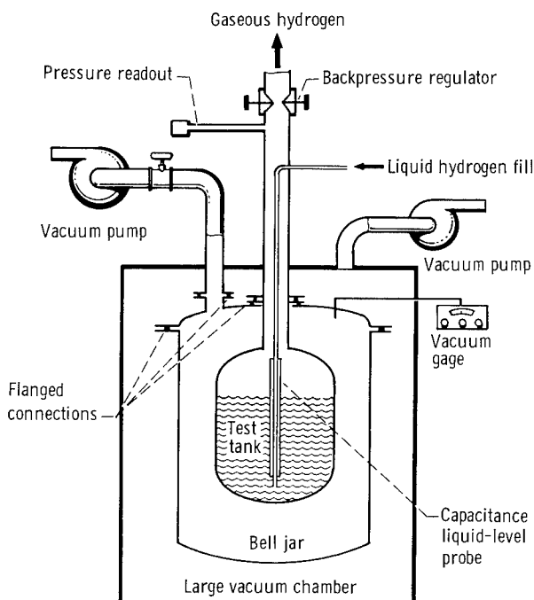
Figure 3. - Liquid-hydrogen test facility.
