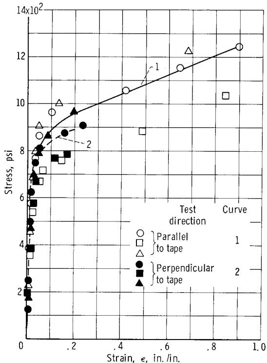
Figure 15. - Stress as function of strain for Teflon tape liner material at room temperature.
