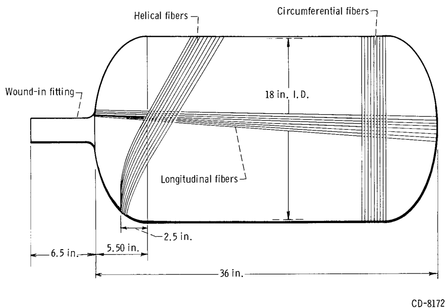
Figure 2. - Schematic of tank 2 (Mylar tape liner) with additional helical wrap.
