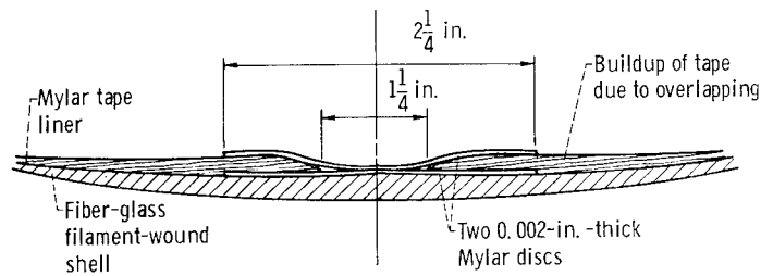
Figure 12. - Cross section of lower dome of filament-wound tank 2 (Mylar liner).
