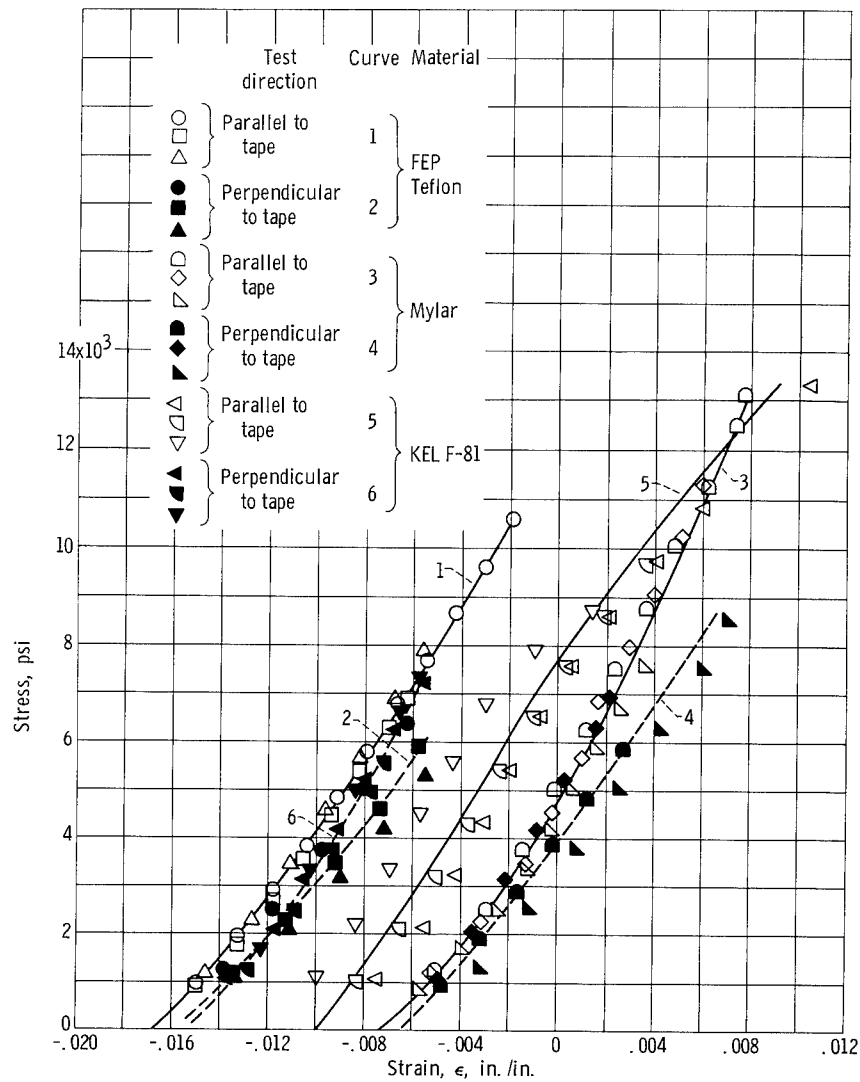
Figure 19. - Thermal shrinkage from room temperature and stress-strain at 20° K (-423° F) for plastic tape liner materials.
