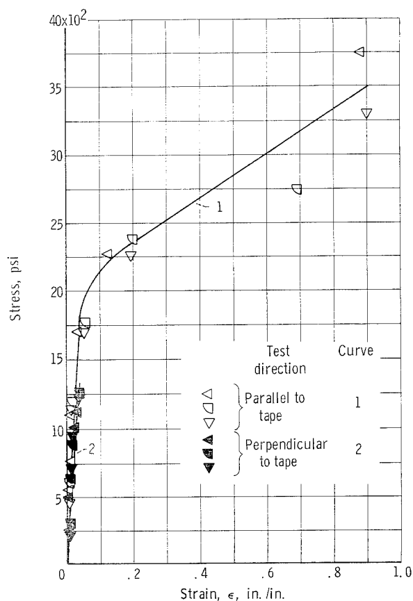
Figure 17. - Stress as function of strain for KEL F-81 tape liner material at room temperature.
