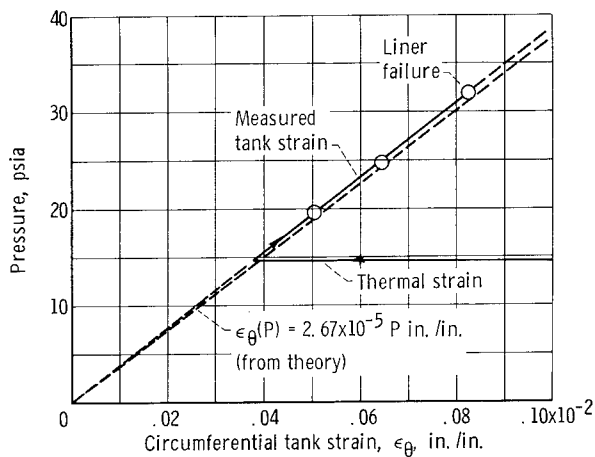
Figure 13. - Tank 2 (Mylar liner) strain as function of pressure at -423° F.
