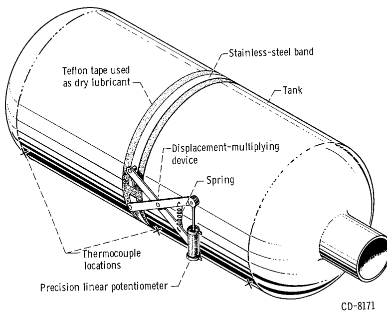
Figure 4. - Additional instrumentation for tank 2. (Mylar tape liner).
