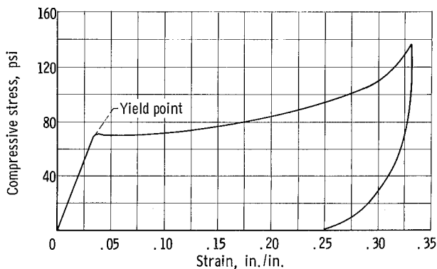
Figure 3. - Typical stress-strain curve for polyurethane foam. Room-temperature compression test; density, 4 pounds per cubic foot; modulus of elasticity, 2500 pounds per square inch.
