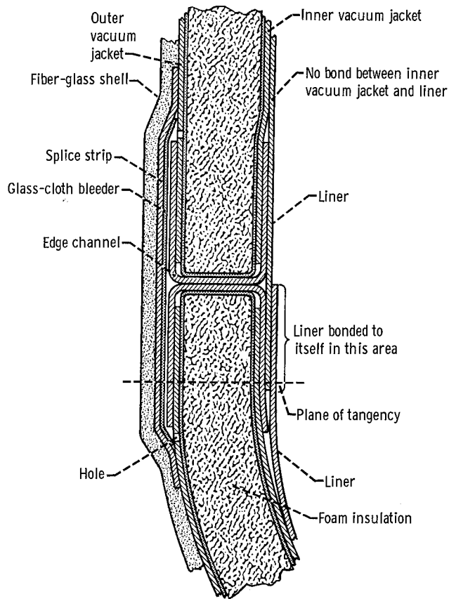
(e) Detail of section through bleeder patch (doubblers not shown).
