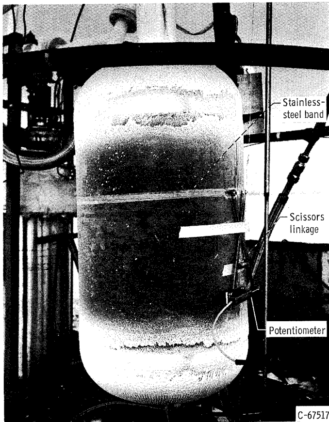
Figure 12. - Strain-gage equipped tank in outdoor test facility.
