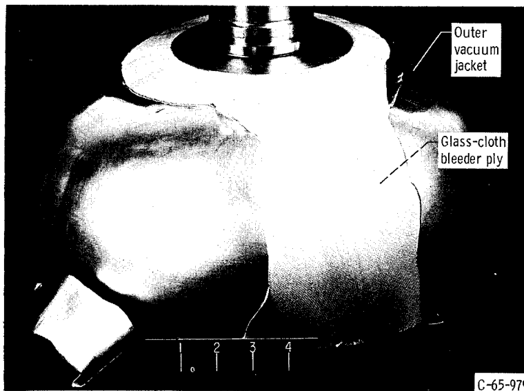
Figure 5. - Top dome insulation (outer vacuum jacket peeled away to expose bleeder ply).
