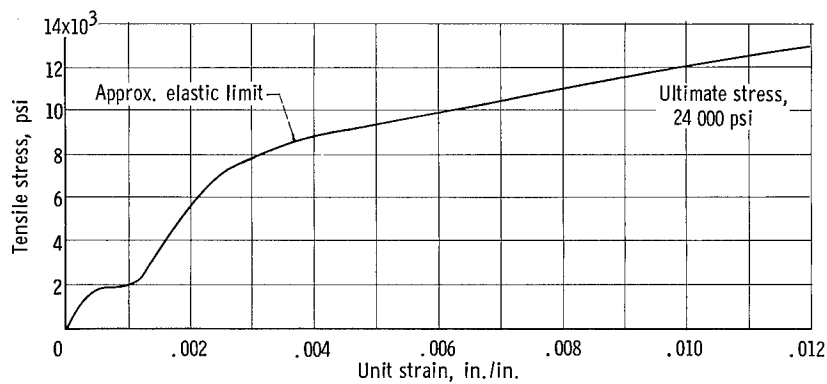
Figure 7. - -300° F stress-strain curve for AMA laminate (0.0007 in. aluminum, 0.001 in. Mylar, 0.0007 in. aluminum).
