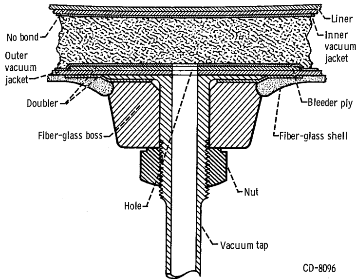
(f) Detail of vacuum tap.
