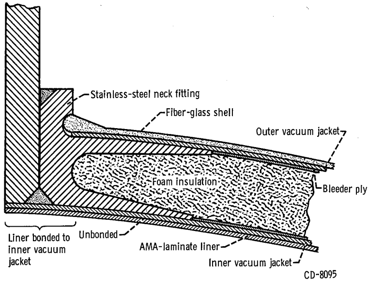
(c) Detail of neck fitting (doublers not shown).
