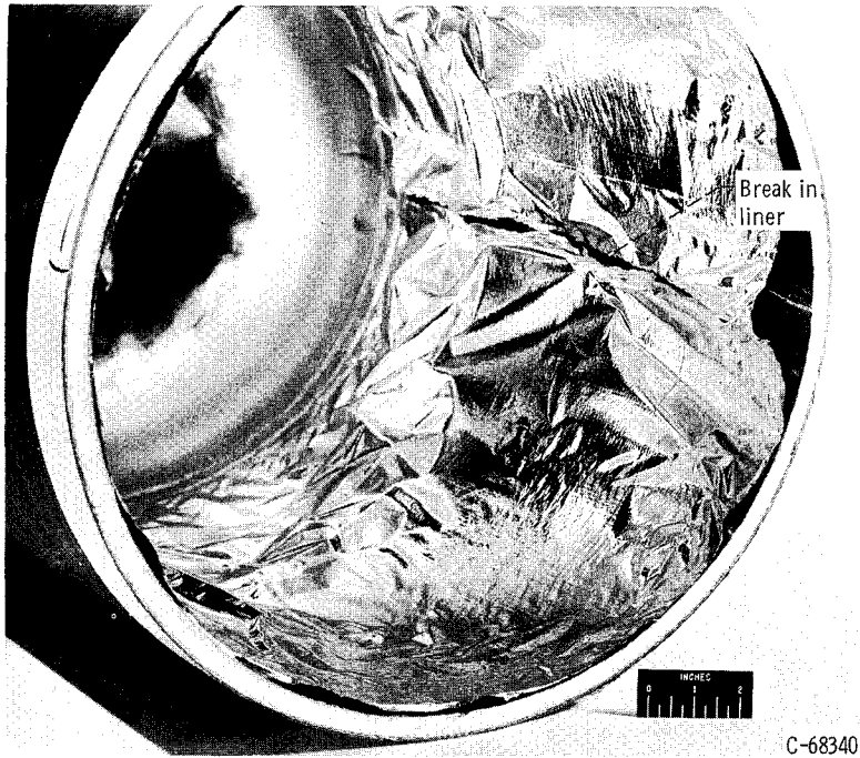
Figure 17. - Inside of tank (showing failure in liner).
