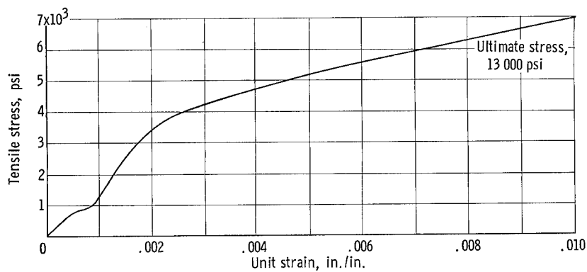
Figure 6. - Room-temperature stress-strain curve for AMA laminate (0.0007 in. aluminum, 0.001 in. Mylar 0.0007 in. aluminum).
