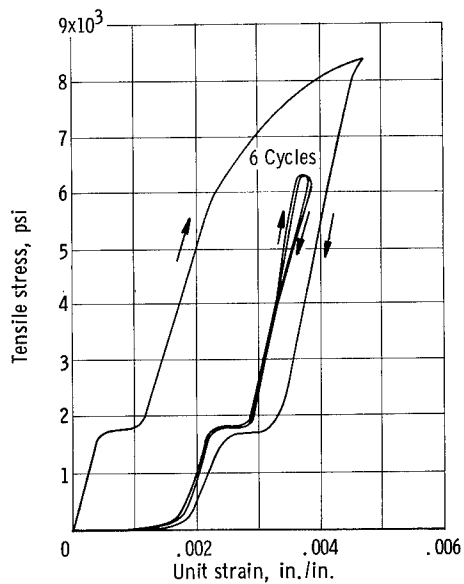
Figure 8. - Stress-strain curve of AMA laminate showing six loading cycles after an initial stress of 8300 pounds per square inch. Temperature, -300° F.
