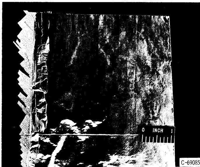
Figure 18. - Section of liner material at break.
