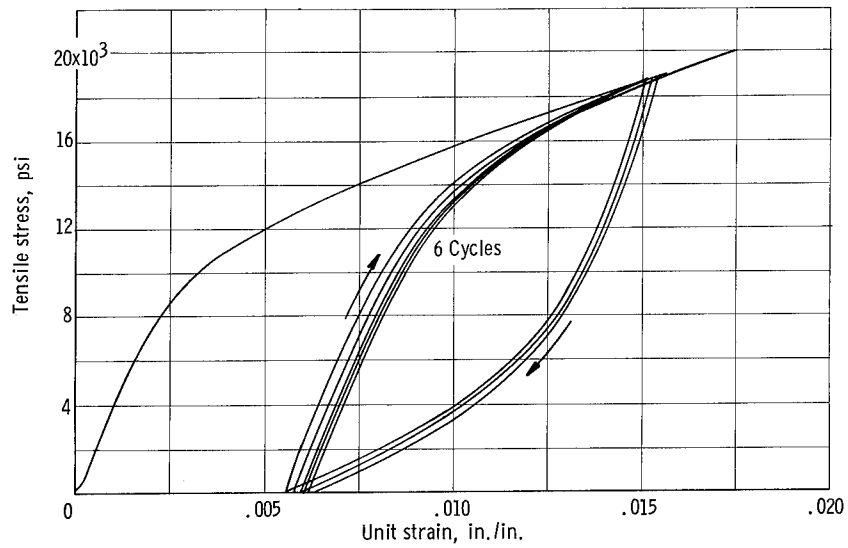
Figure 9. - Stress-strain curve for prestressed (10 040 psi at room temperature) AMA laminate at -300^{\circ} F.
