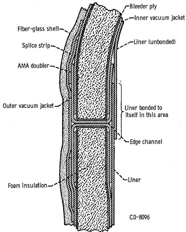
(d) Detail of typical splice between dome and cylinder.
