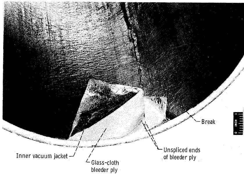
Figure 19. - Failure in inner vacuum jacket (liner removed from tank).
