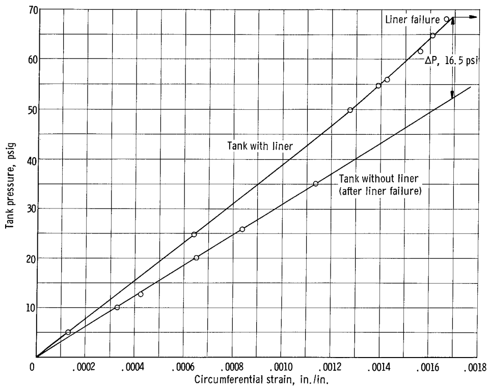
Figure 20. - Effect of liner failure on circumferential strain of tank wall.
