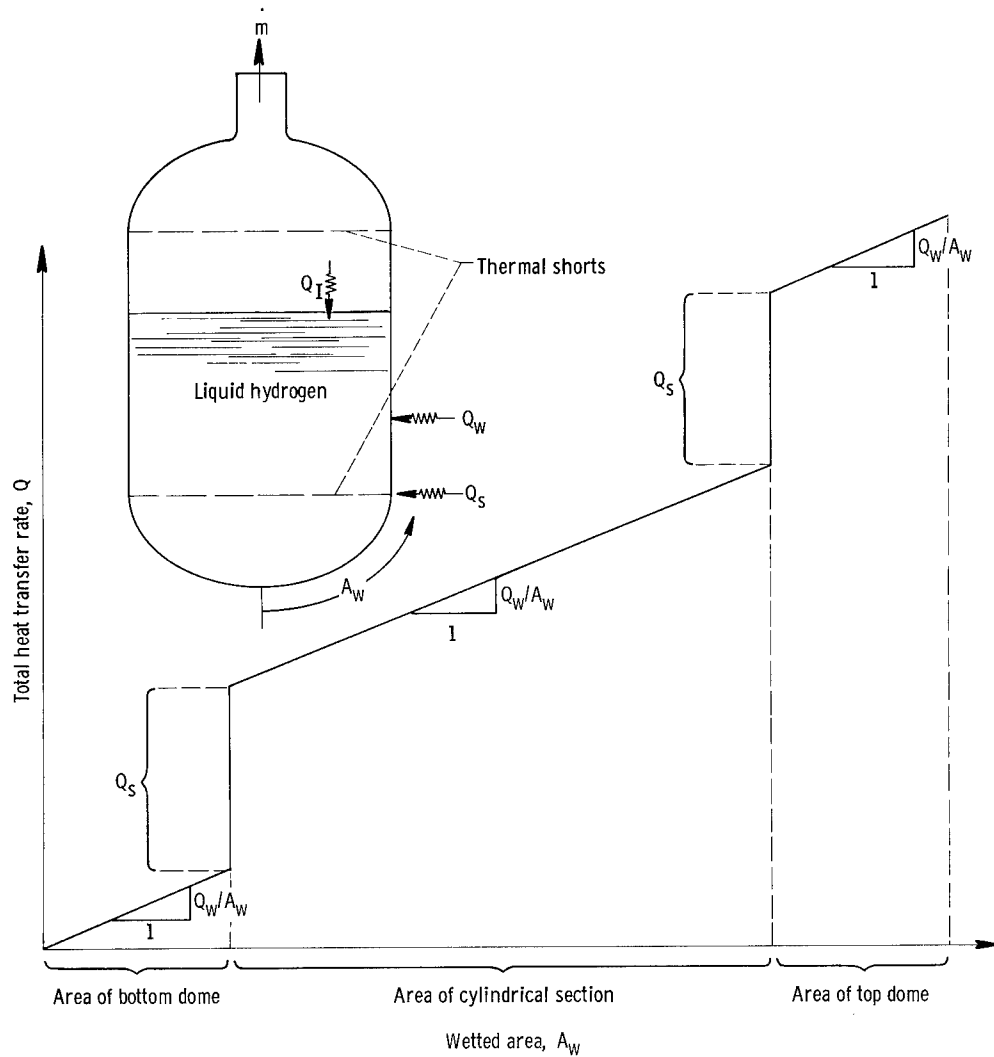
Figure 13. - Idealized curve of heat-transfer rate and wetted area for a liquid-hydrogen tank.
