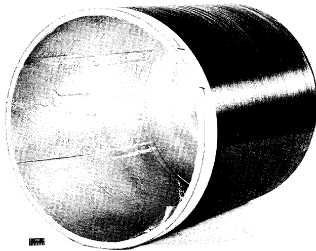
Figure 21. - Inner vacuum jacket after testing.
