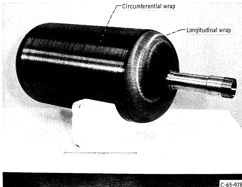
Figure 2. - Completed filament-wound test tank.
