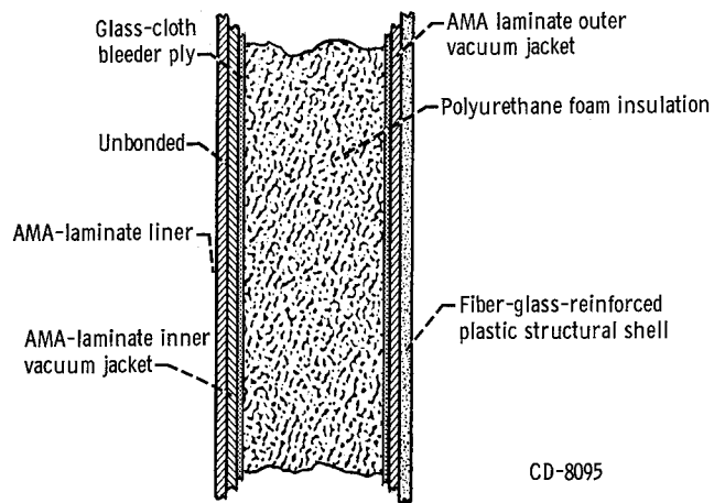
(b) Enlarged typical section through tank wall.
