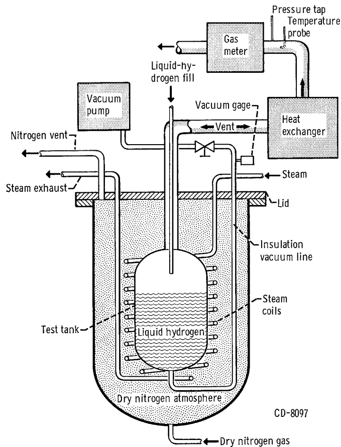
Figure 11. - Controlled-environment test facility.
