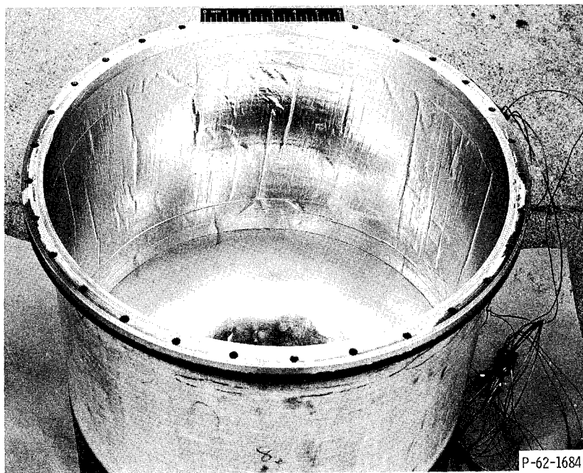
Figure 10. - Uninsulated filament-wound tank with test liner wrinkles after two temperature and pressure cycles.
