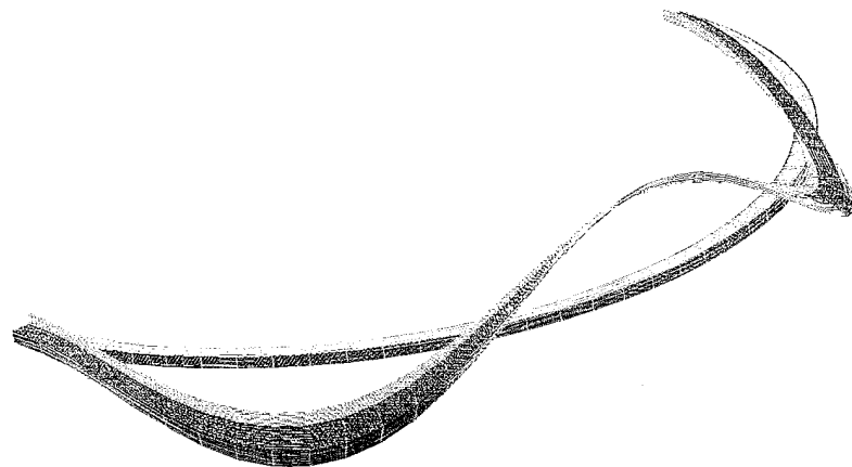
Figure 9. Vibration mode shapes for semicircular beam with symmetric Z-section shown in figure 8. Numbers in parentheses are converged thin-walled beam frequencies (in hertz); other numbers are frequencies obtained by two-dimensional model.
