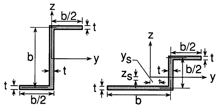
Symmetric section
