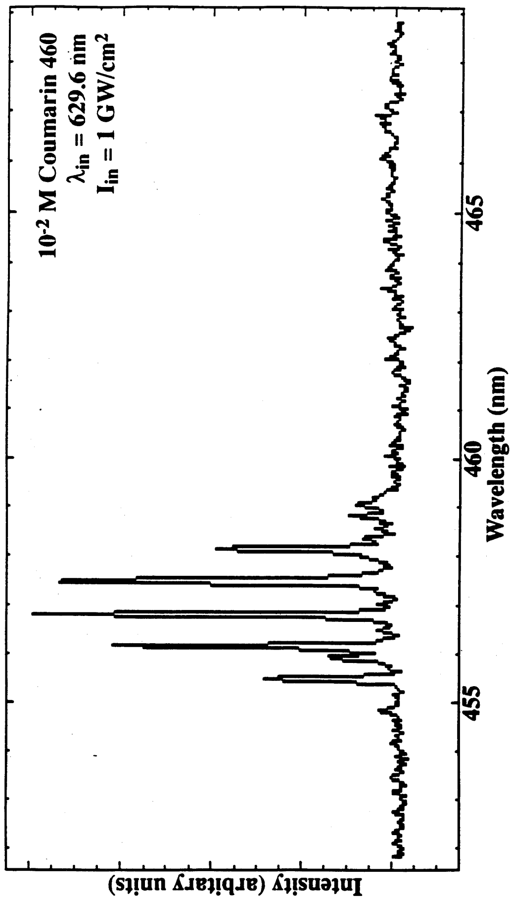
Figure 8. TPA pumped lasing spectrum of 10^{-2} M coumarin 460 in ethanol droplets with an input laser at 629.6 nm and an input intensity of 1 \text{ GW/cm}^2 . The periodic peaks correspond to the MDR
