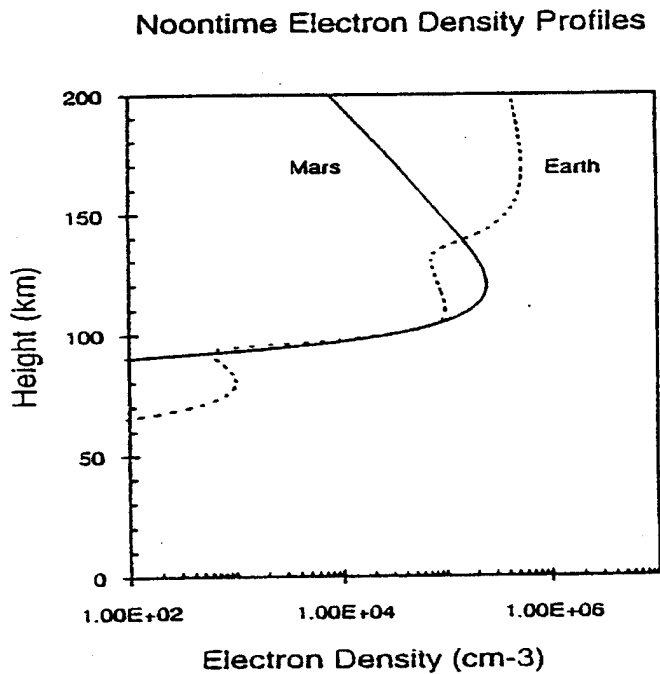
Figure 18 - Peak daytime electron peaks for Earth and Mars. (Fry, Yowell 1993)
