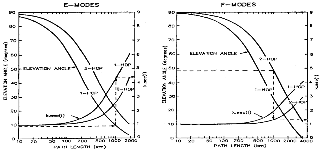
Figure 19 - Obliquity factor ( k \sec l ) and elevation angle as a function of circuit length for E and F layers. (McNamara, 1991)
