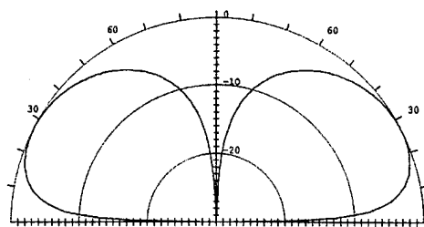
RF-1955 Elevation Pattern for Average Soil Characteristics at 30 MHz
