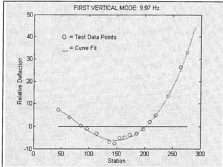
Figure 14. First Vertical Mode.
