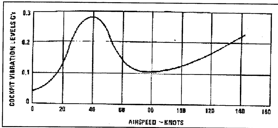
Figure 3. Helicopter Vibration Variation with Airspeed. From [Ref. 1].
