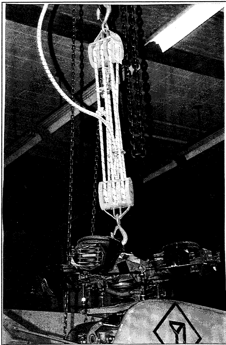
Figure 7. Helicopter Suspension System.
