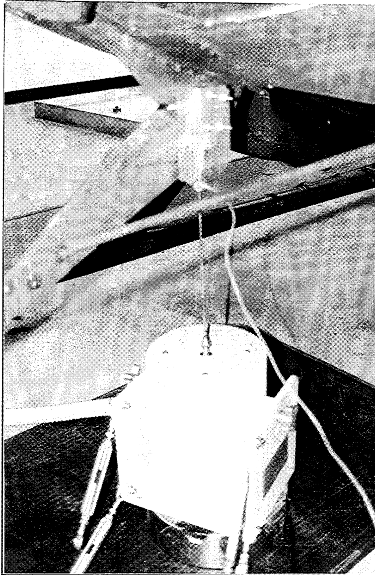
Figure 13. Vertical Excitation of Helicopter.
