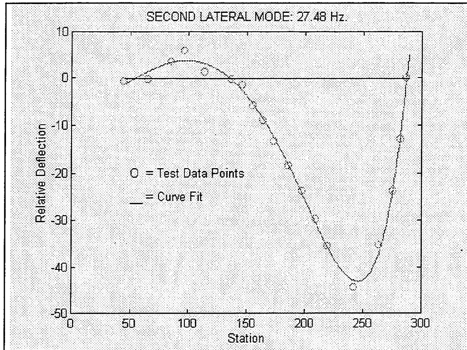
Figure 12. Second Lateral Mode.
