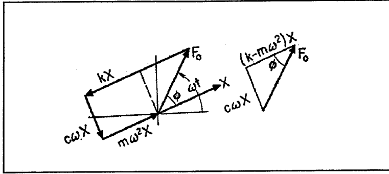
Figure 1. Vector Representation of Forced Vibration With Viscous Damping. From [Ref. 2].
