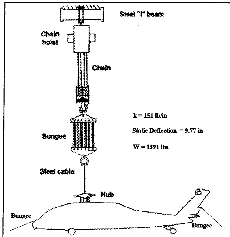
Figure 6. Typical Helicopter Vibration Suspension System Modified for OH-6A Parameters. From [Ref. 8].
