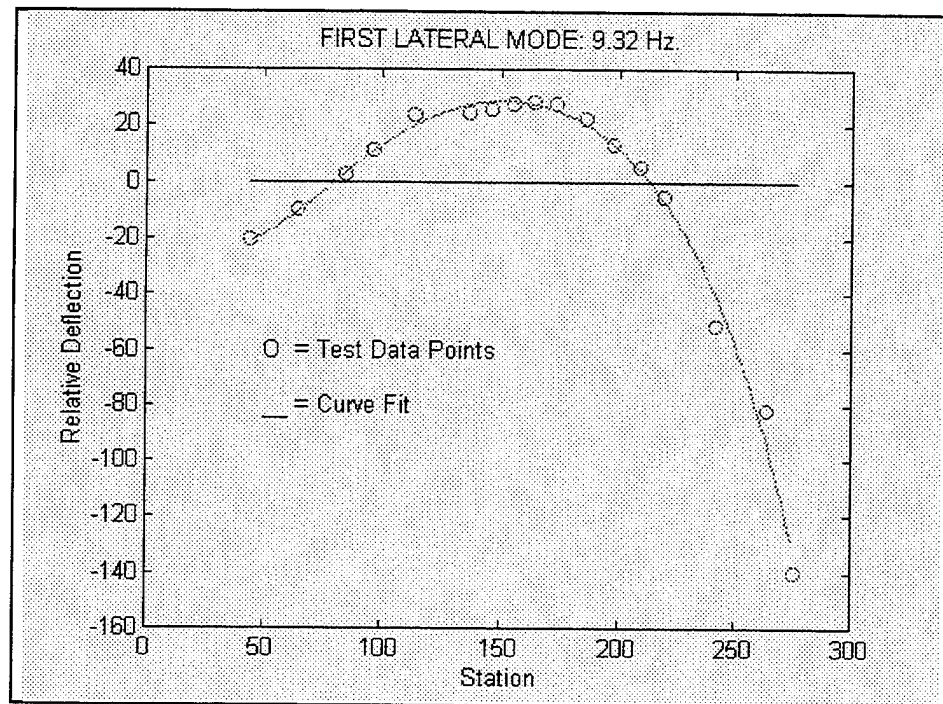
Figure 11. First Lateral Mode.
