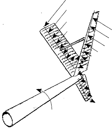
Figure 16. Motion Produced by First Torsional Mode.
