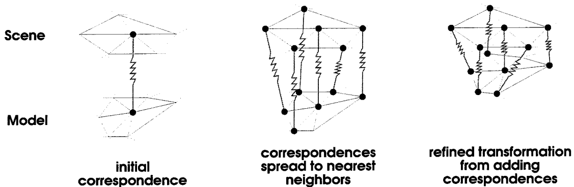
Figure 11: Illustration of the spreading of point correspondences and refinement of the match transformation in the ICPV algorithm.
