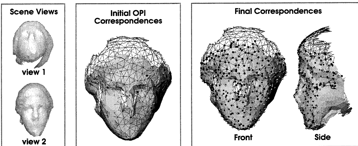
Figure 12: The registration of two views of a plastic model of the head of Venus. From left to right are shown: two camera images of the views to be registered, the registration of the views (view 1 shaded, view2 wireframe) from OPI correspondences shown as spheres, and a frontal and side view of the registration after the ICPV algorithm with established correspondences.
