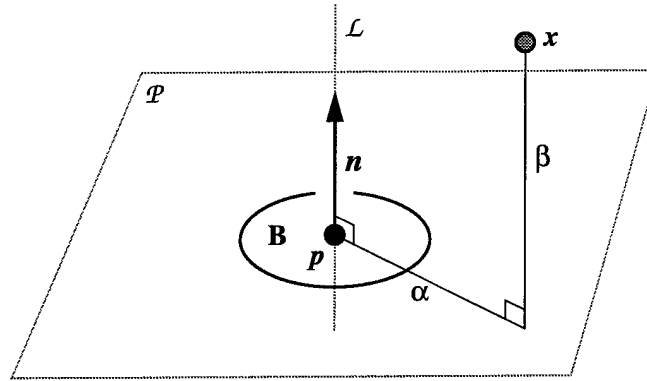
Figure 1: Oriented point basis.
