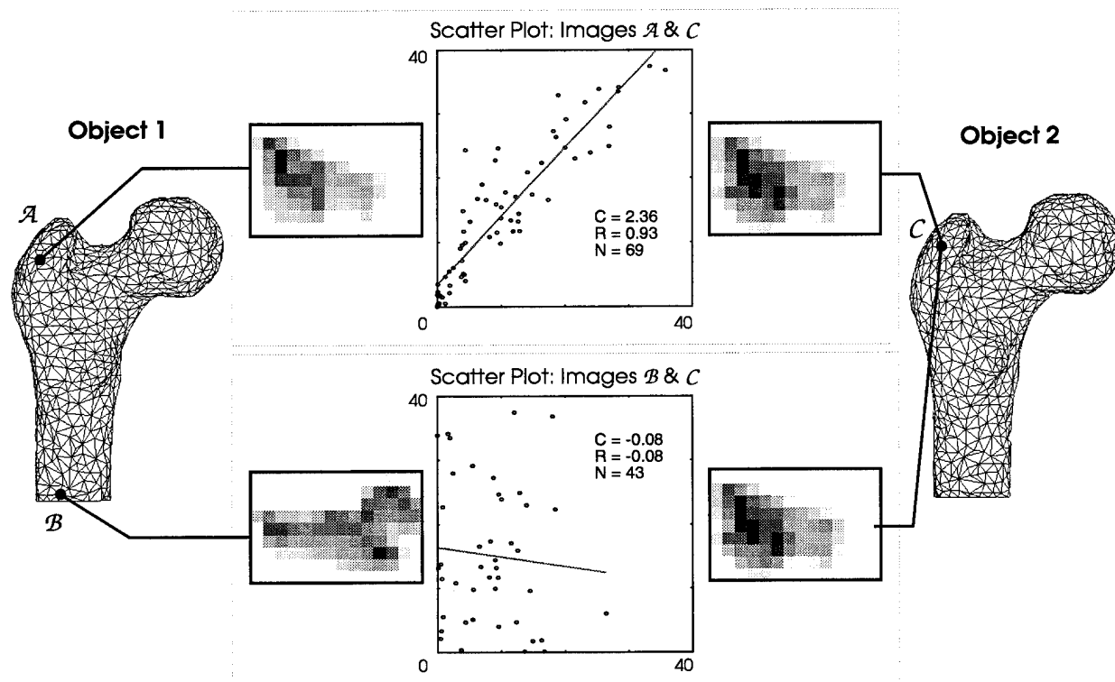
Figure 5: Comparison of spin-images visualized as scatter plots.
