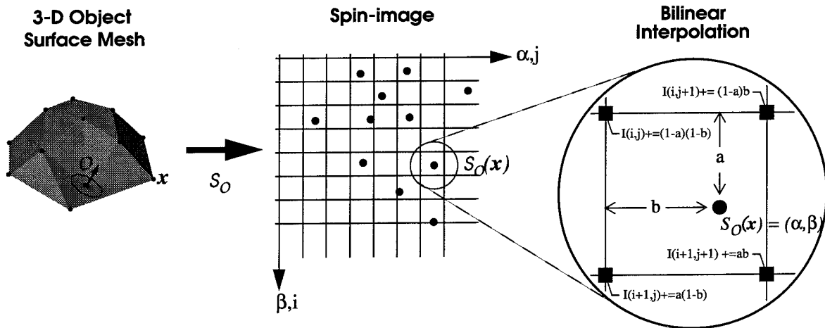
Figure 4: The addition of a point to the 2-D array representation of a spin-image.
