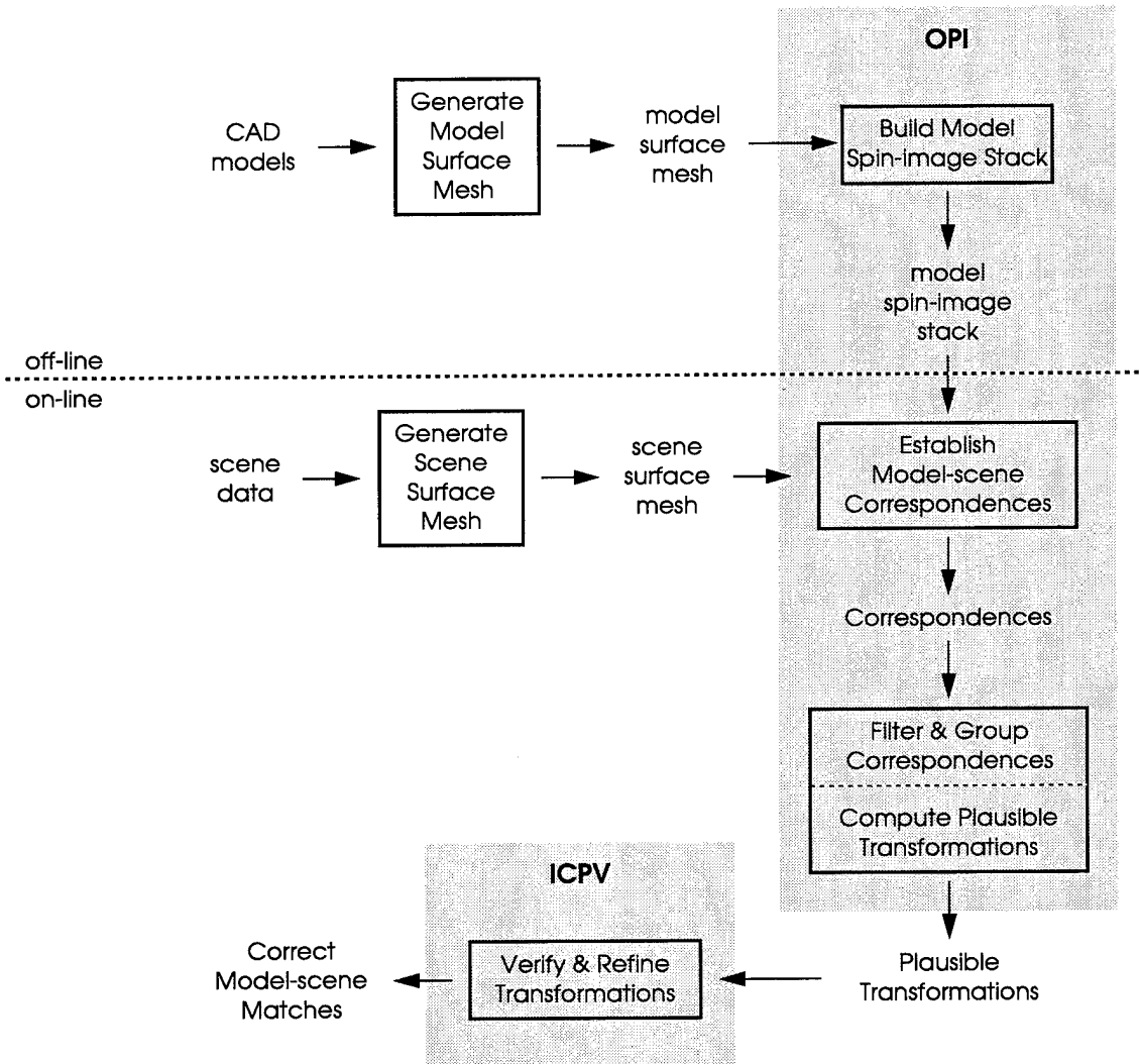
Figure 9: Object recognition block diagram.
