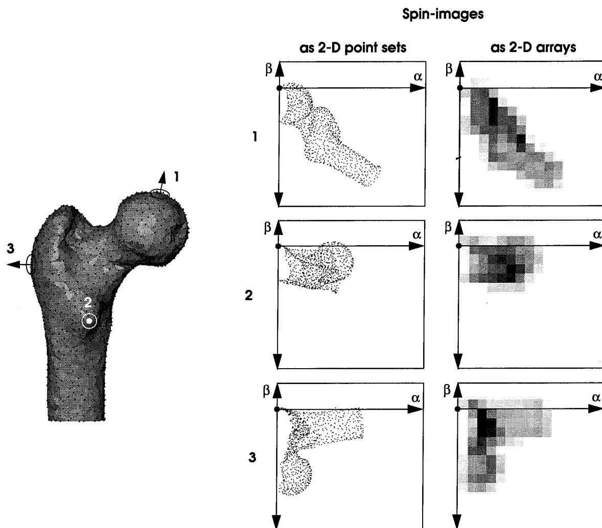
Figure 2: Points distributed on the surface of a femur bone with three oriented point bases and the spin-images associated with the three spin-maps shown as point sets and 2-D arrays viewed as greyscale images.
