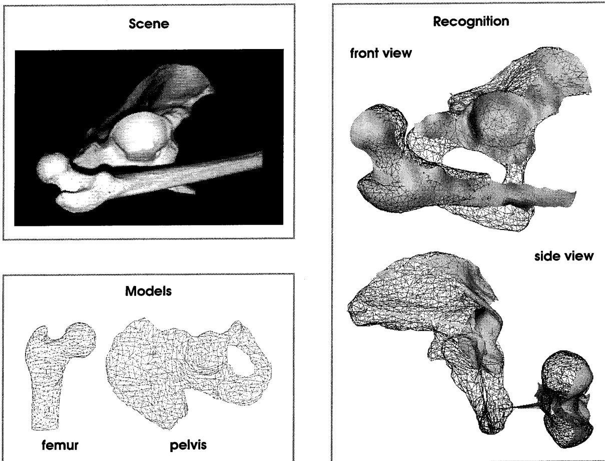
Figure 16: Simultaneous recognition of multiple anatomical models in a partial view with clutter and occlusions.
