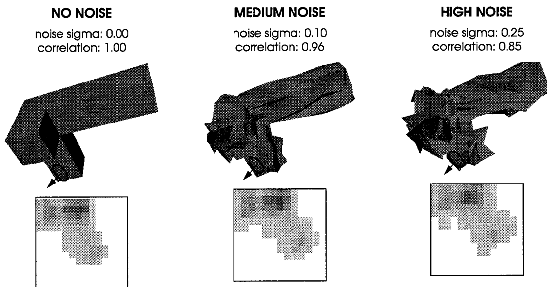
Figure 18: How scene noise effects spin images.
