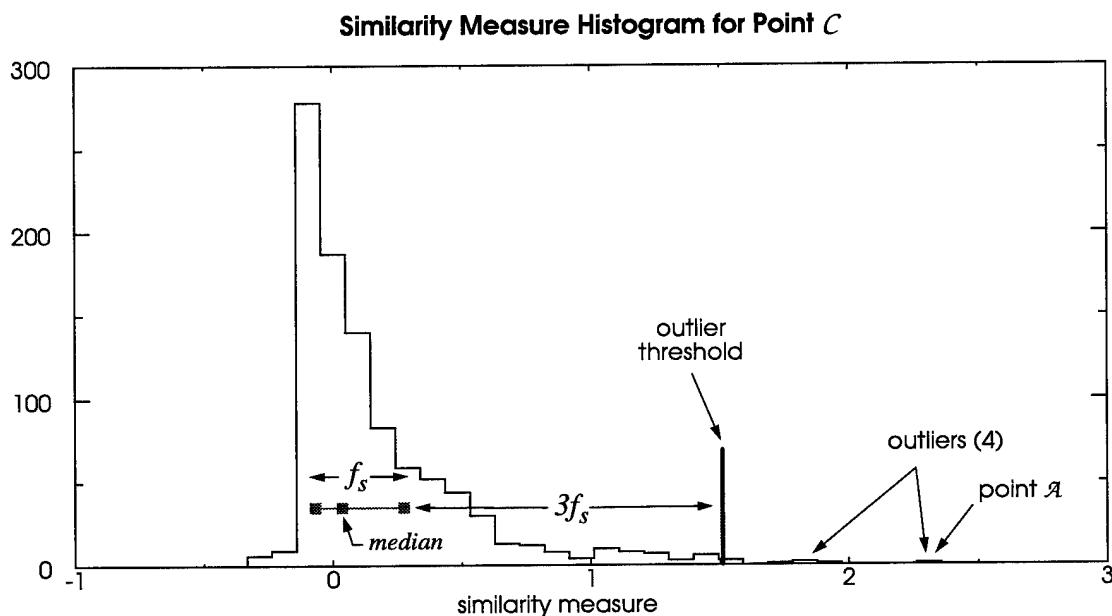
Figure 7: Similarity measure histogram for point C when compared to object 1 (from Figure 5).
