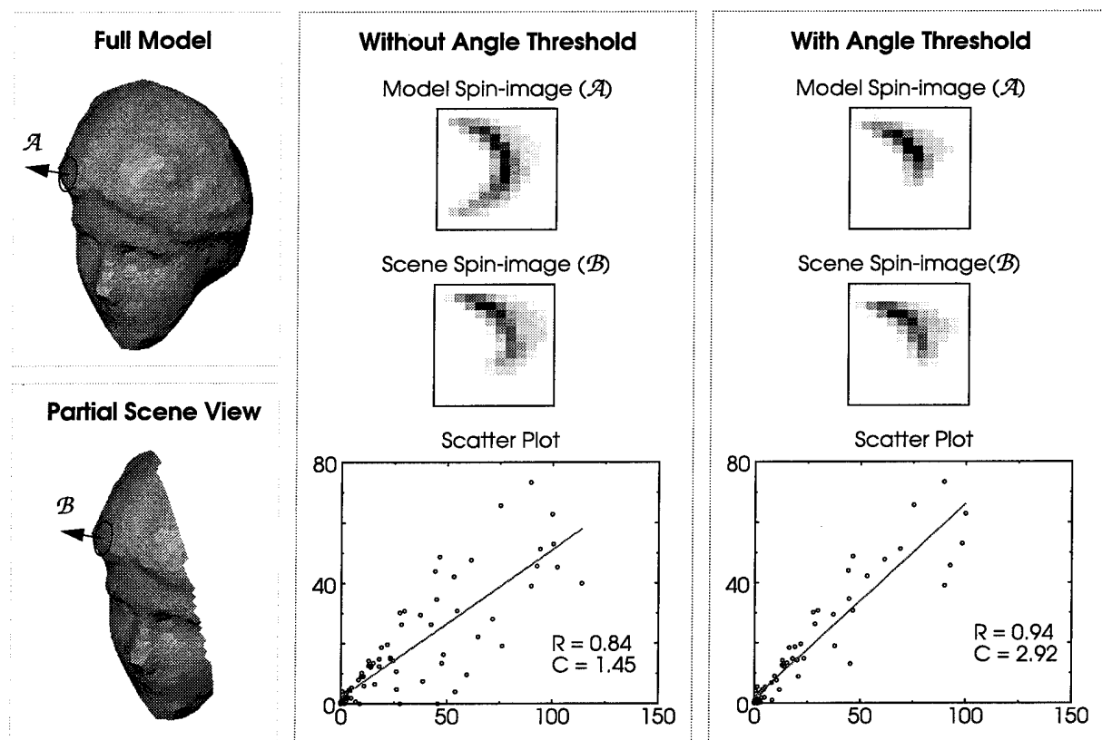
Figure 8: Effect of threshold on angle between surface normals when dealing with partial scene views.
