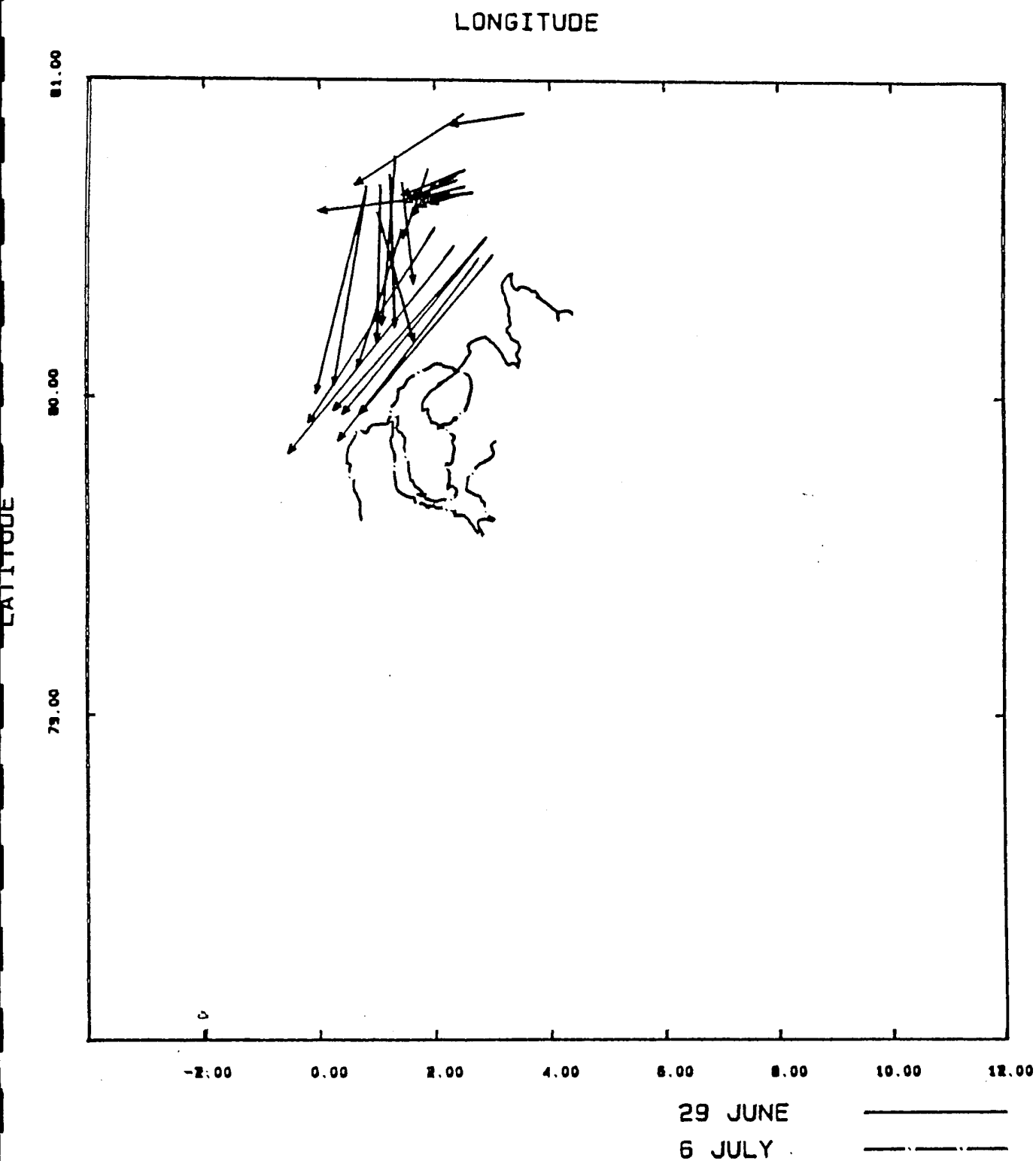
Figure 9. SAR sea ice floe vector and edge generated from manual interpretation of optically processed SAR data gathered during MIZEX-84.
