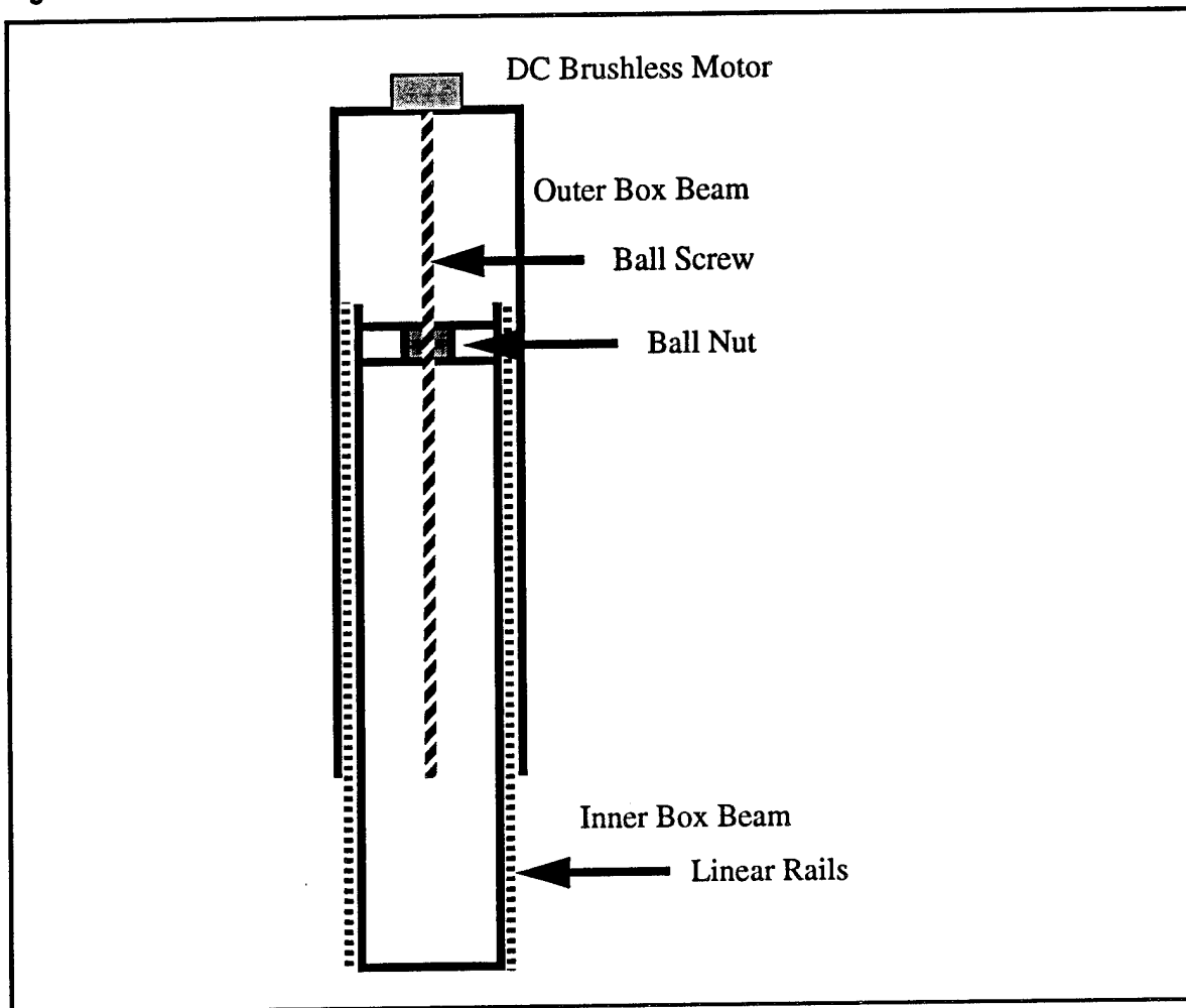
Figure 5-4 Column structure
