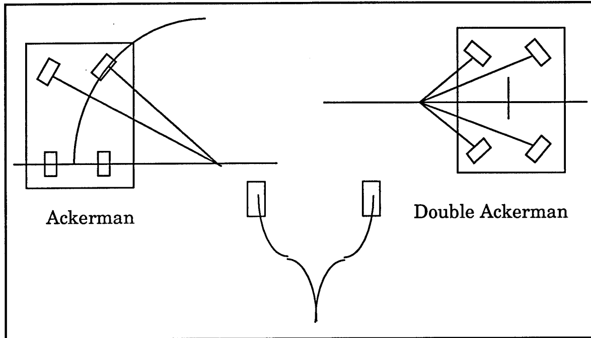
Figure 8-1 Ackerman steering.
