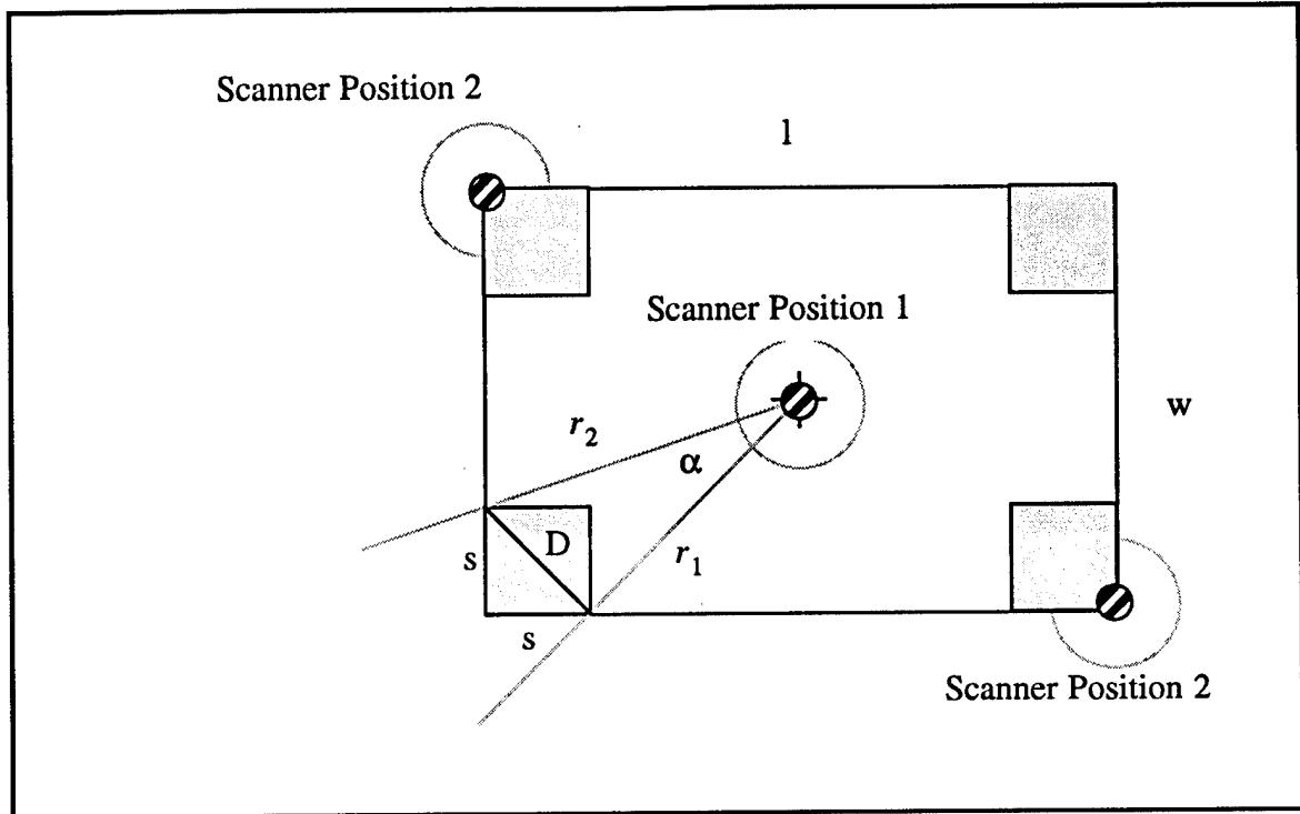
Figure 7-9 Scanner placement.
