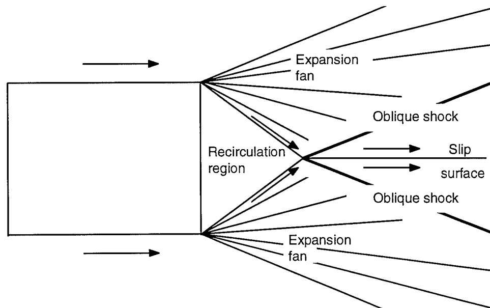
Figure 7-9 Wake Region
