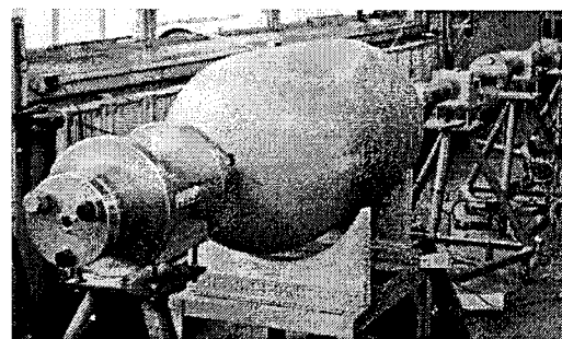
Figure 6-19 Dump Tank
