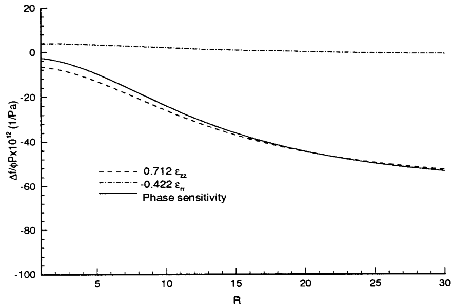
Figure 6. Strain Components and Phase Sensitivity of a Hytel-Coated Optical Fiber in Plane Strain With Hydrostatic Boundary Condition (Case b)
