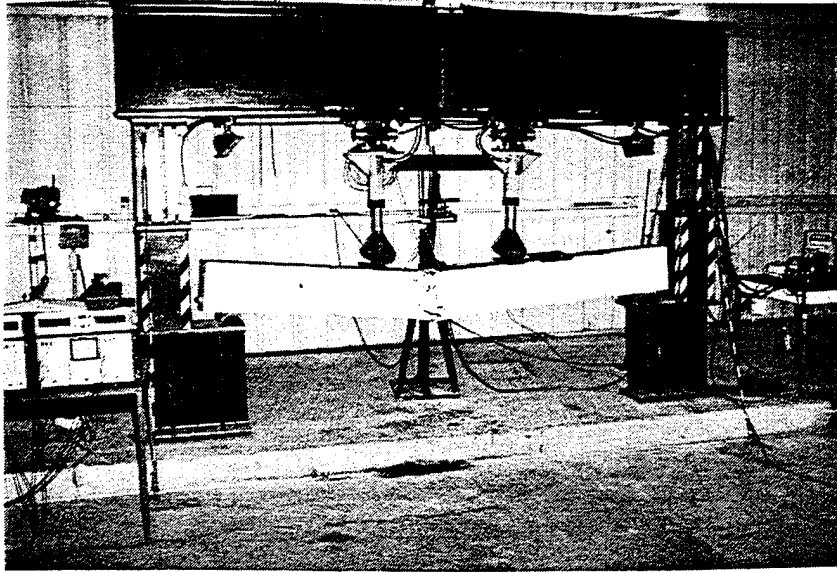
Figure 12. View 1 of the Instrumented Rebar Beam Testing Process.
