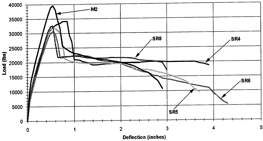
Figure 10. Load-Deflection Curves, Beam 1 (Instrumented Rebar).
