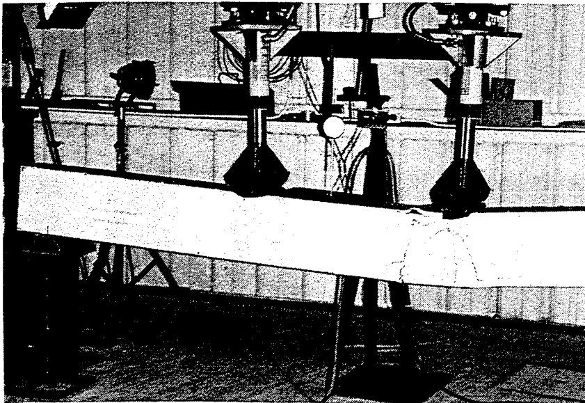
Figure 28. View 3 of the Non-Instrumented Rebar Beam Testing Process.
