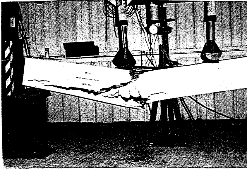
Figure 27. View 2 of the Non-Instrumented Rebar Beam Testing Process.
