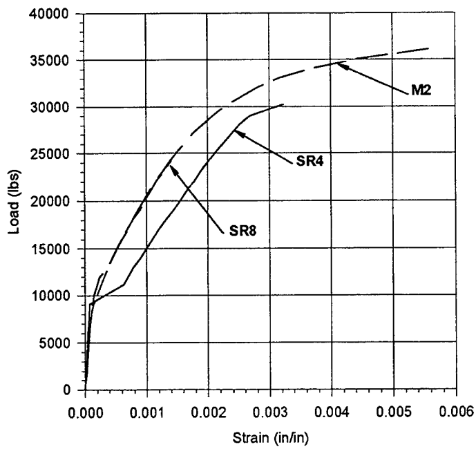
Figure 17. Strain-Load Curves, Beam 2 (Instrumented Rebar).
