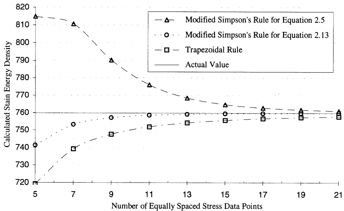
Figure 5.3. Comparison of Integration Routines.
