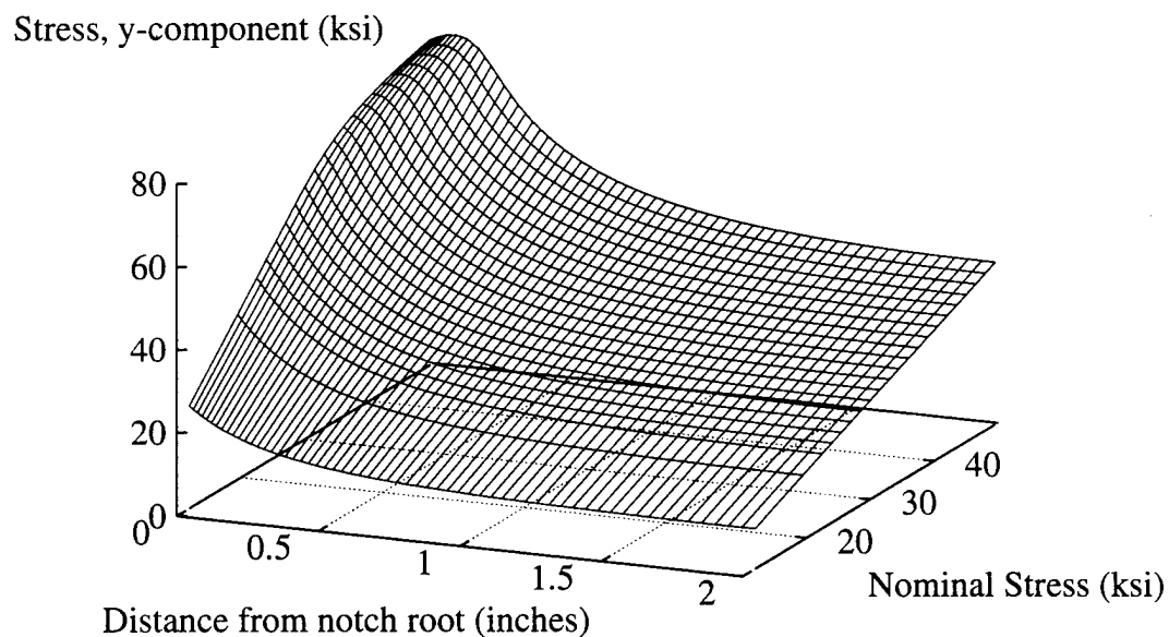
Figure 7.14. Distribution of \sigma_y Along Minimum Cross Section for Narrow Plate in Plane Strain.
