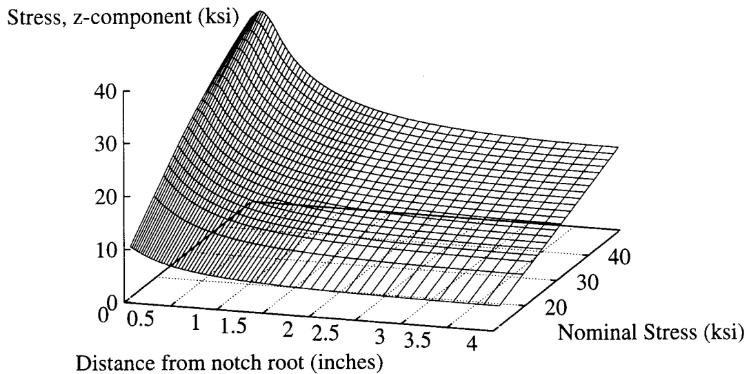
Figure 7.18. Distribution of \sigma_z Along Minimum Cross Section for Wide Plate in Plane Strain.
