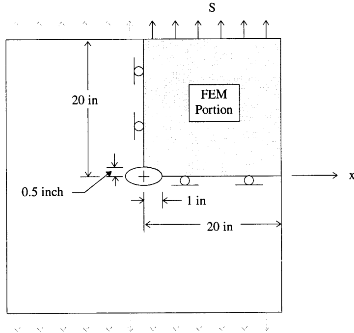
Figure 4.3 Layout of model representing an elliptical hole in an infinite plate.
