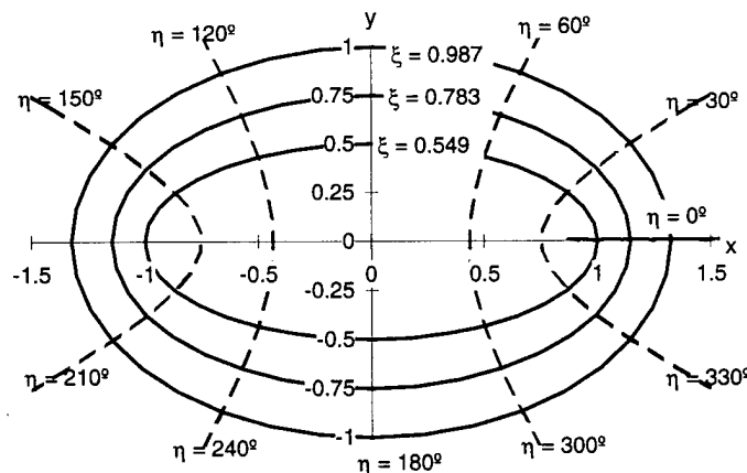
Figure 4.1. Elliptical Coordinate System.
