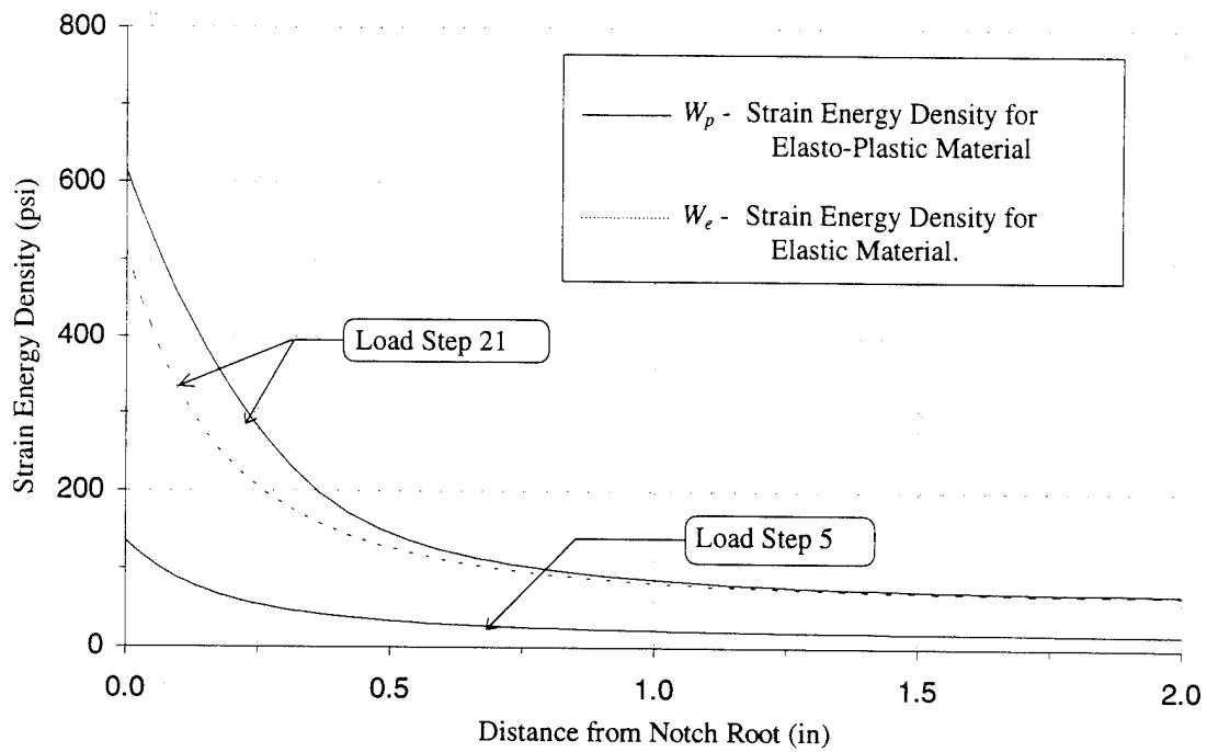
Figure 6.11. Strain Energy Density along x -axis for Narrow Plate in Plane Stress.
