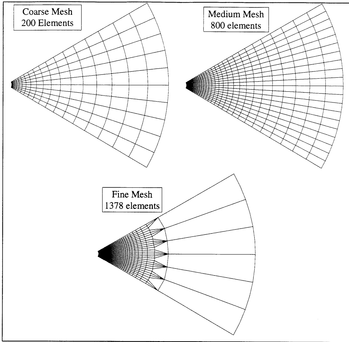
Figure 4.18. Layout of Element Meshes for Hole in an Infinite Plate.
