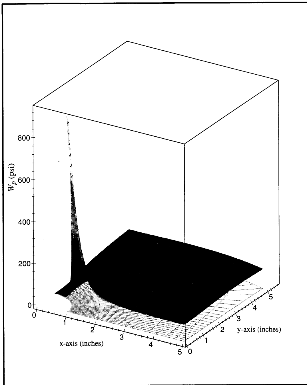
Figure 6.10. Plastic Strain Energy Density W_p for Wide Plate in Plane Stress at Load Set 21.
