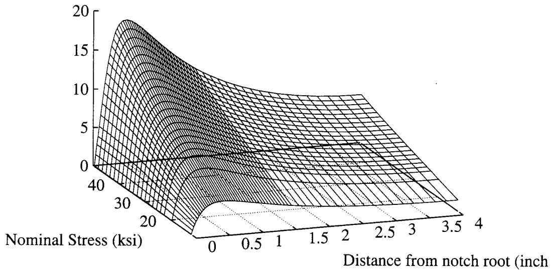
Figure 7.16. Distribution of \sigma_x Along Minimum Cross Section for Wide Plate in Plane Strain.
