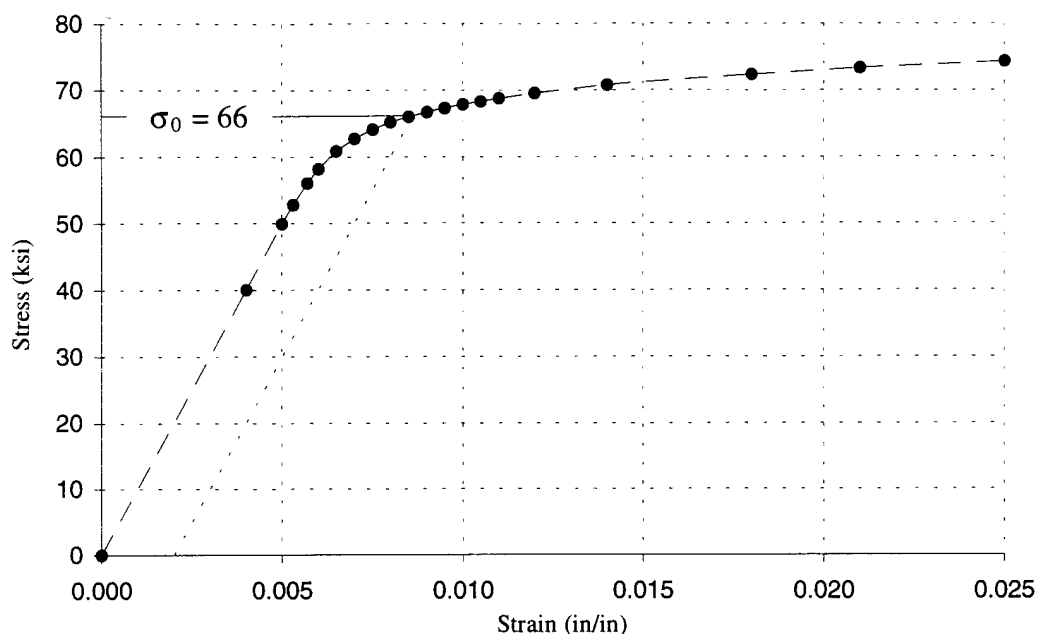
Figure 6.2 Stress-Strain Curve for 7075-T6 Aluminum.
