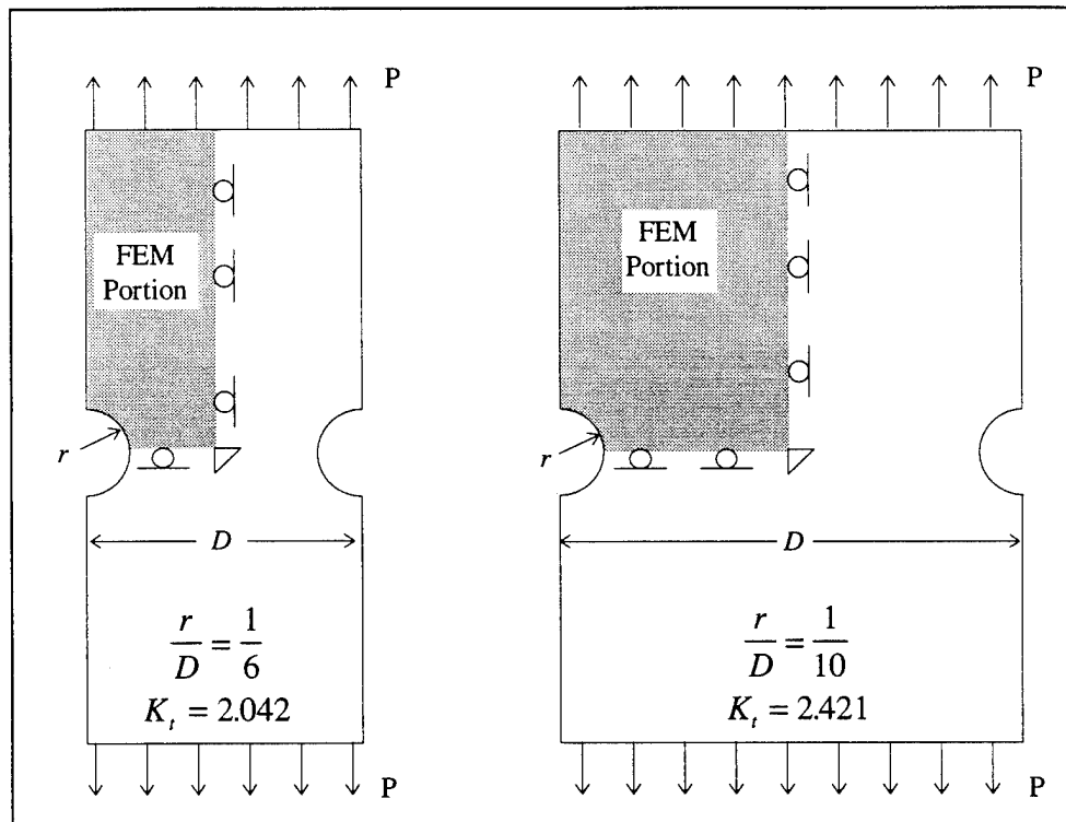
Figure 6.1. Notch Geometry and Finite Element Boundary Conditions.
