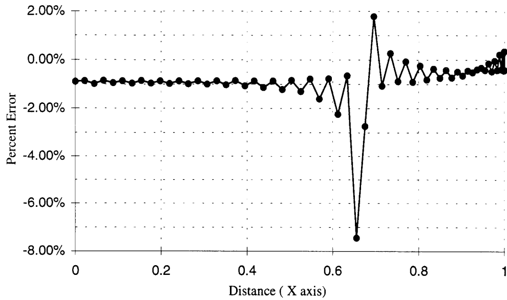
Figure 4.7 Percent Error of tangential stress \sigma_{\eta} along elliptical boundary.
