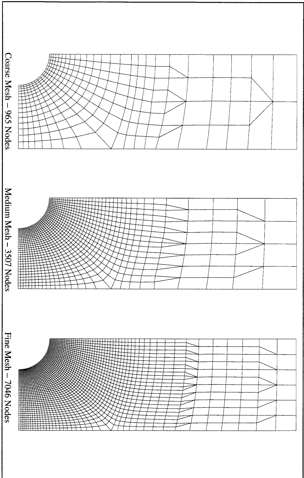
Figure 6.3. Mesh Layouts for Narrow Notched Plate.
