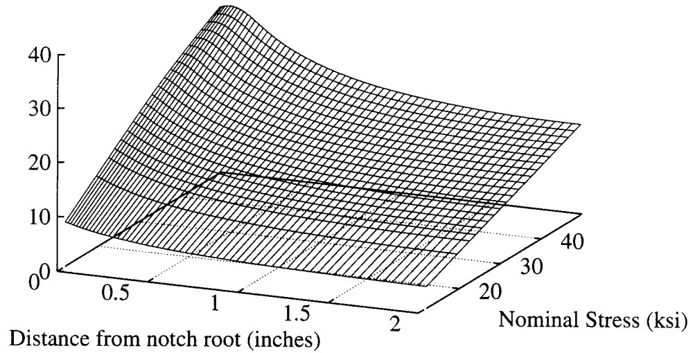
Figure 7.15. Distribution of \sigma_z Along Minimum Cross Section for Narrow Plate in Plane Strain.
