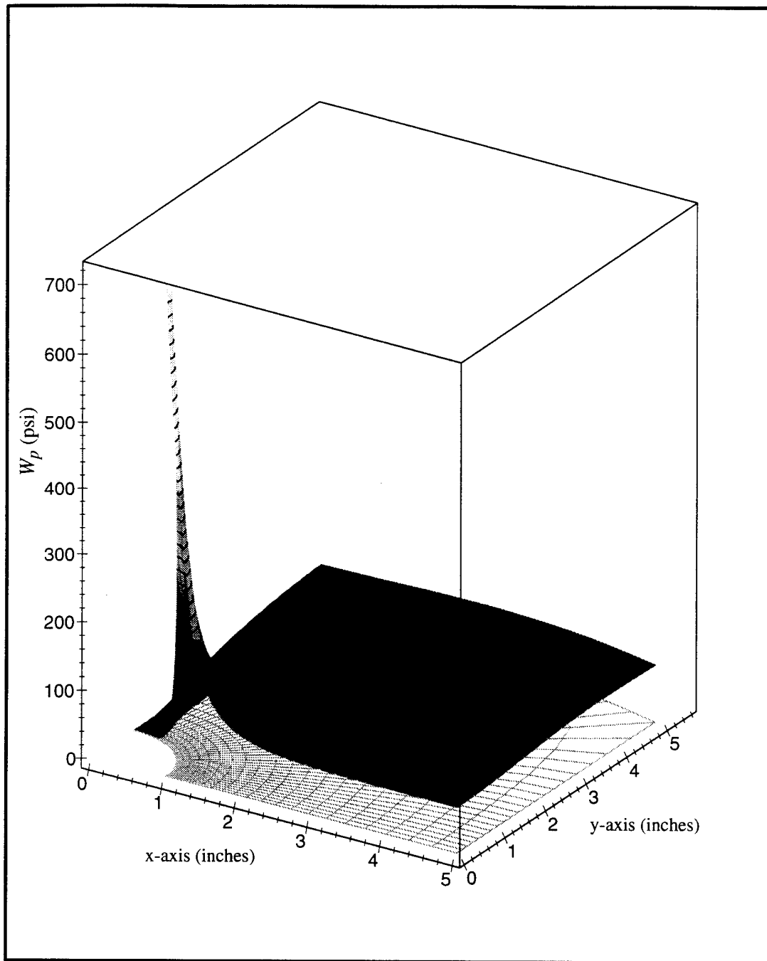
Figure 6.18. Plastic Strain Energy Density W_p for Wide Plate in Plane Strain at Load Set 21.
