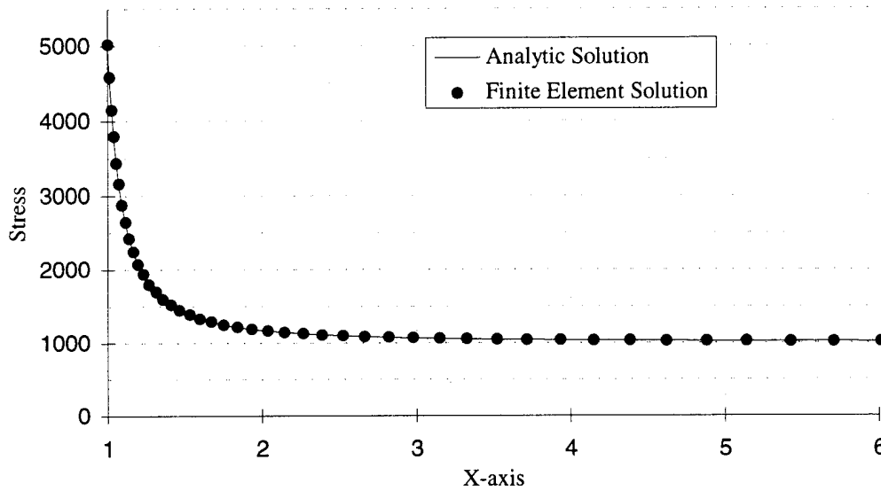
Figure 4.9. Axial stress ( \sigma_\eta ) along \eta = 0 .
