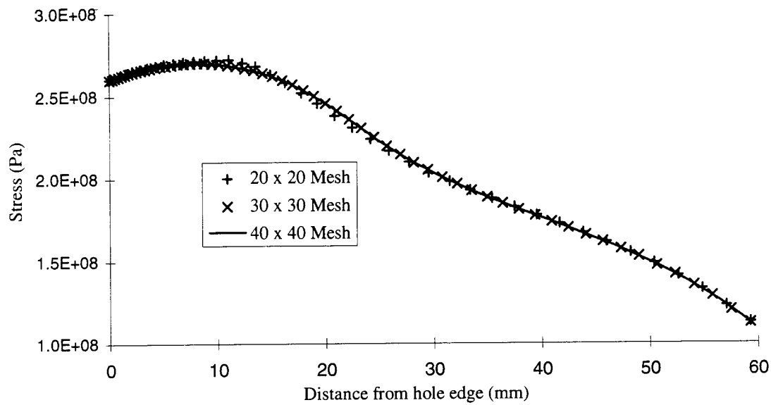
Figure 4.31. Distribution of \sigma_y for Various Mesh Sizes.
