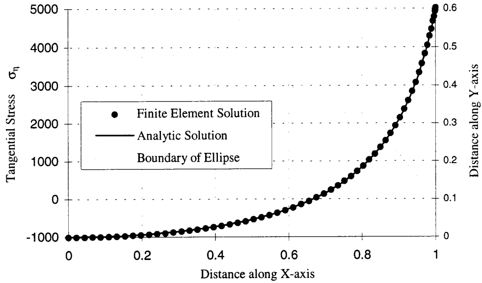
Figure 4.6. Tangential Stress \sigma_{\eta} Along Elliptical Boundary.
