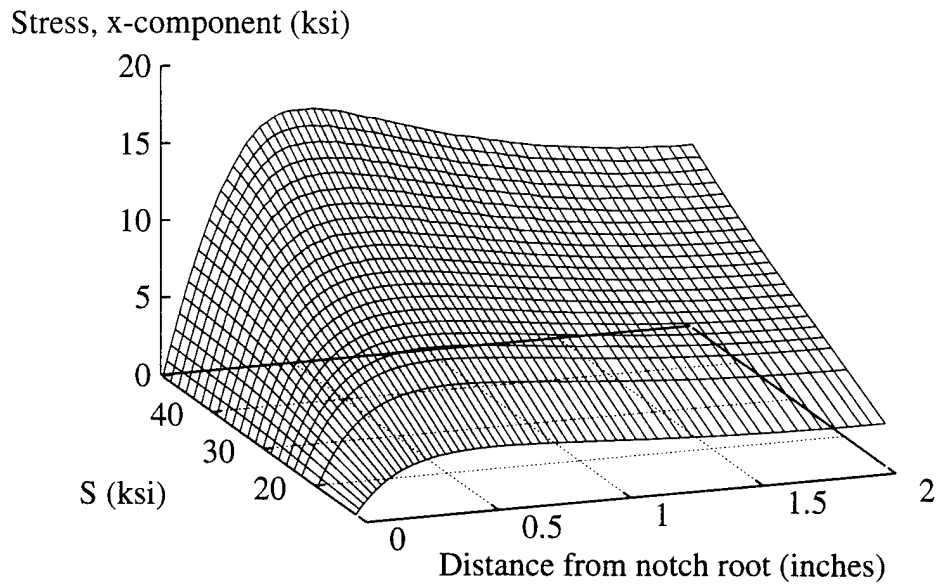
Figure 7.1. Distribution of \sigma_x Along Minimum Cross Section for Narrow Plate in Plane Stress.
