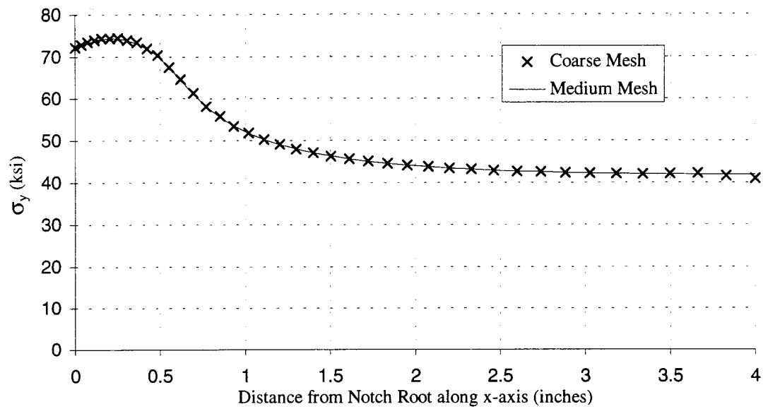
Figure 6.7. Distribution of \sigma_y for Mesh Comparison of Wide Plate FEM Model.
