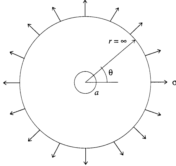
Figure 4.15 Infinite plate with circular hole
