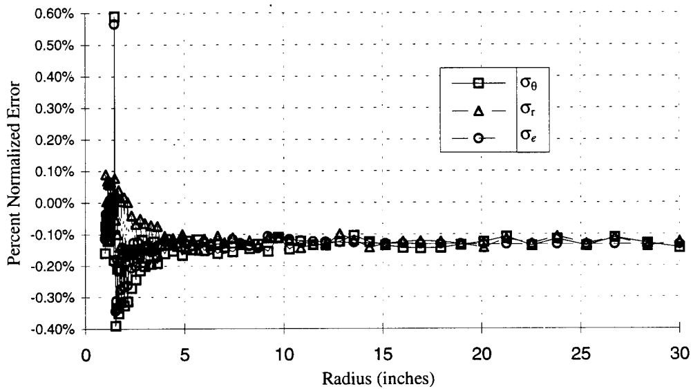
Figure 4.25. Normalized error of FEM stresses versus analytic solution for case 2.
