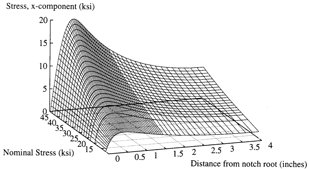
Figure 7.3. Distribution of \sigma_x Along Minimum Cross Section for Wide Plate in Plane Stress.
