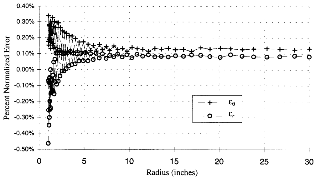
Figure 4.27. Normalized error of FEM strains versus analytic solution for case 2.
