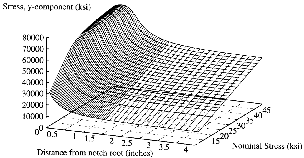
Figure 7.4. Distribution of \sigma_y Along Minimum Cross Section for Wide Plate in Plane Stress.
