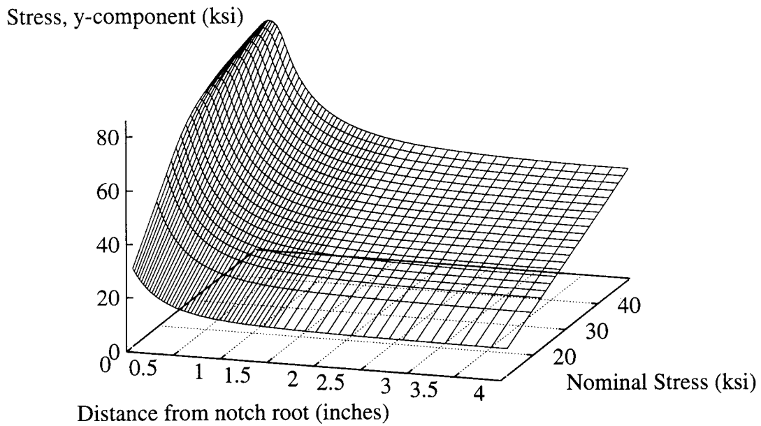
Figure 7.17. Distribution of \sigma_y Along Minimum Cross Section for Wide Plate in Plane Strain.
