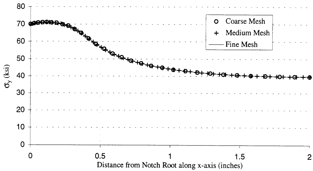
Figure 6.5. Distribution of \sigma_y for Mesh Comparison of Narrow Plate FEM Model.
