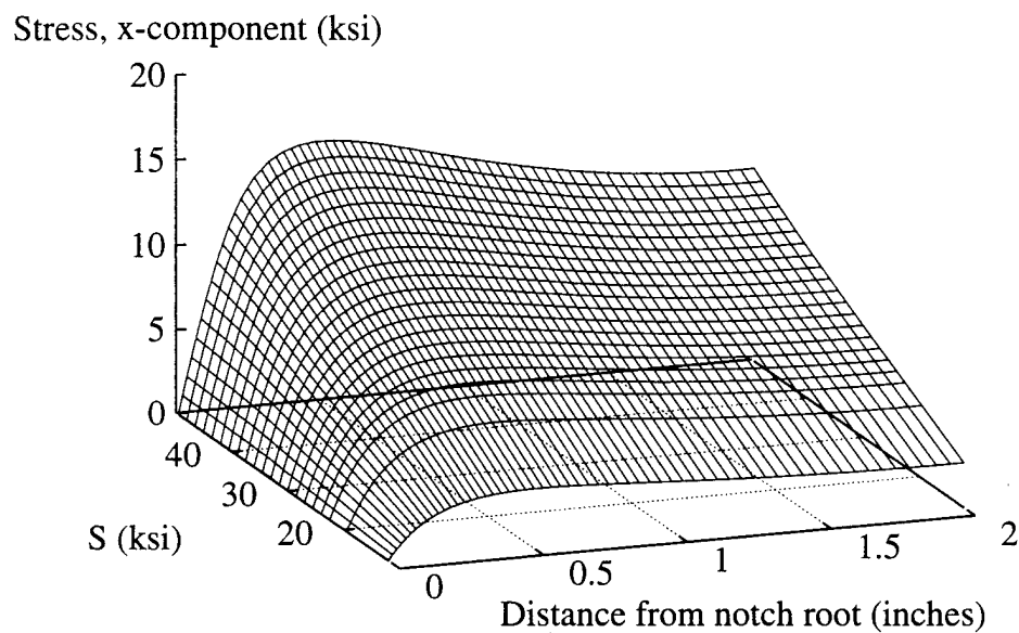
Figure 7.13. Distribution of \sigma_x Along Minimum Cross Section for Narrow Plate in Plane Strain.
