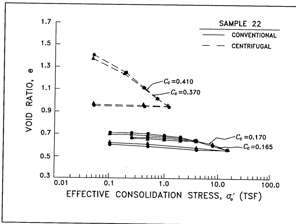
Figure 28. Soil sample 22, comparison of conventional (solid line) and centrifugal (dashed line) consolidation tests
