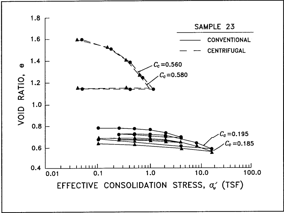
Figure 29. Soil sample 23, comparison of conventional (solid line) and centrifugal (dashed line) consolidation tests
