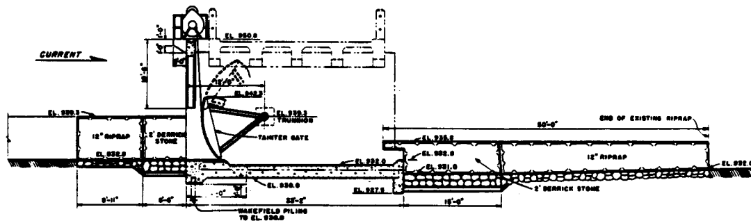
SECTION F-F
