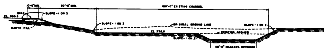
SECTION G-G
