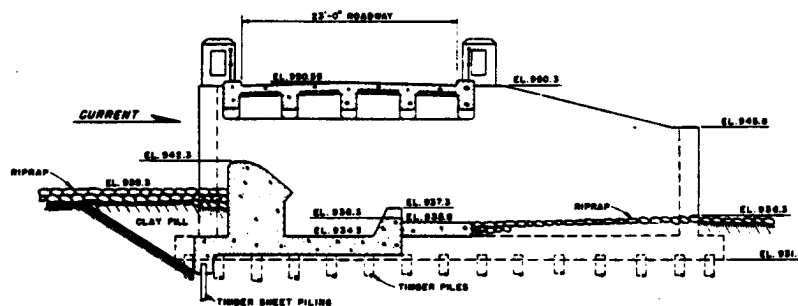
SECTION E-E
