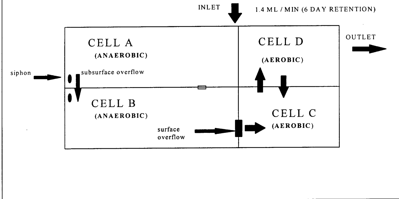
FIGURE 1A. SUBSURFACE-FLOW WETLAND MICROCOSM (W)
