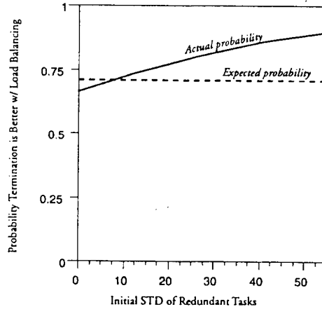
Figure 6: Probability that MLC load balancing will terminate more quickly than static load balancing, fitted using a loglinear model from actual TAMS simulation data.
