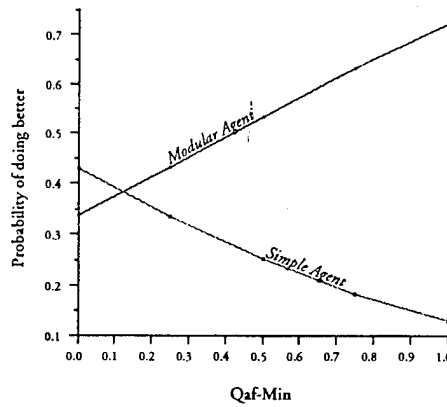
Figure 5: Plot of the probability of the modular or simple coordination styles doing better than the other (total final quality) verses the probability of task quality accumulation being MIN (AND-semantics)
