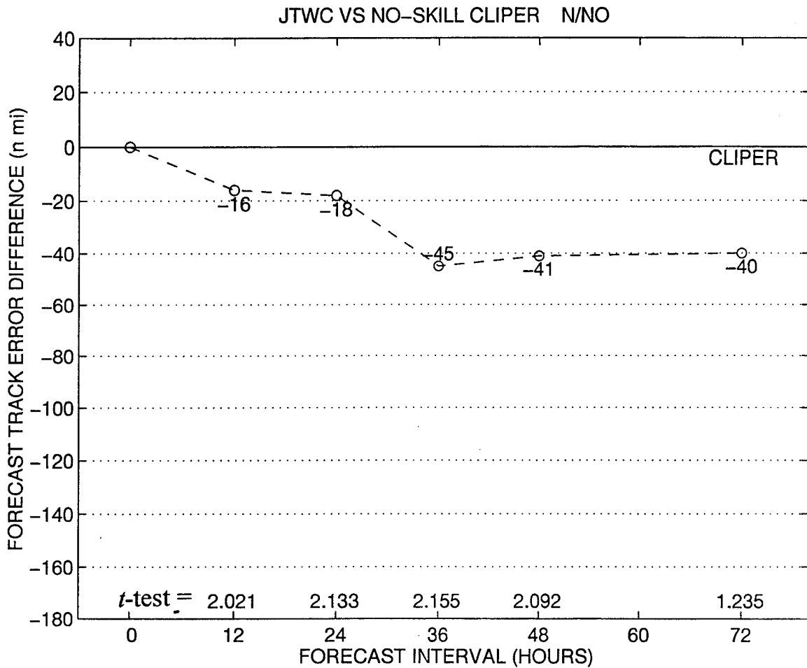
Figure 14 Evaluation of skill of JTWC forecasts as in Figure 12, except for the North-Oriented (NO) Region of the N Pattern. See Table 7 for further details.
