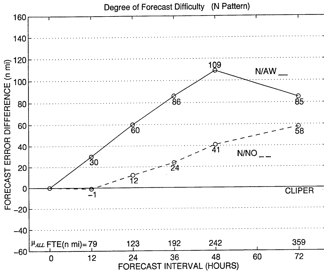
Figure 8 Degree of forecast difficulty as in Fig. 7, except for the North-oriented (N) Pattern. See Table 3 for further details.
