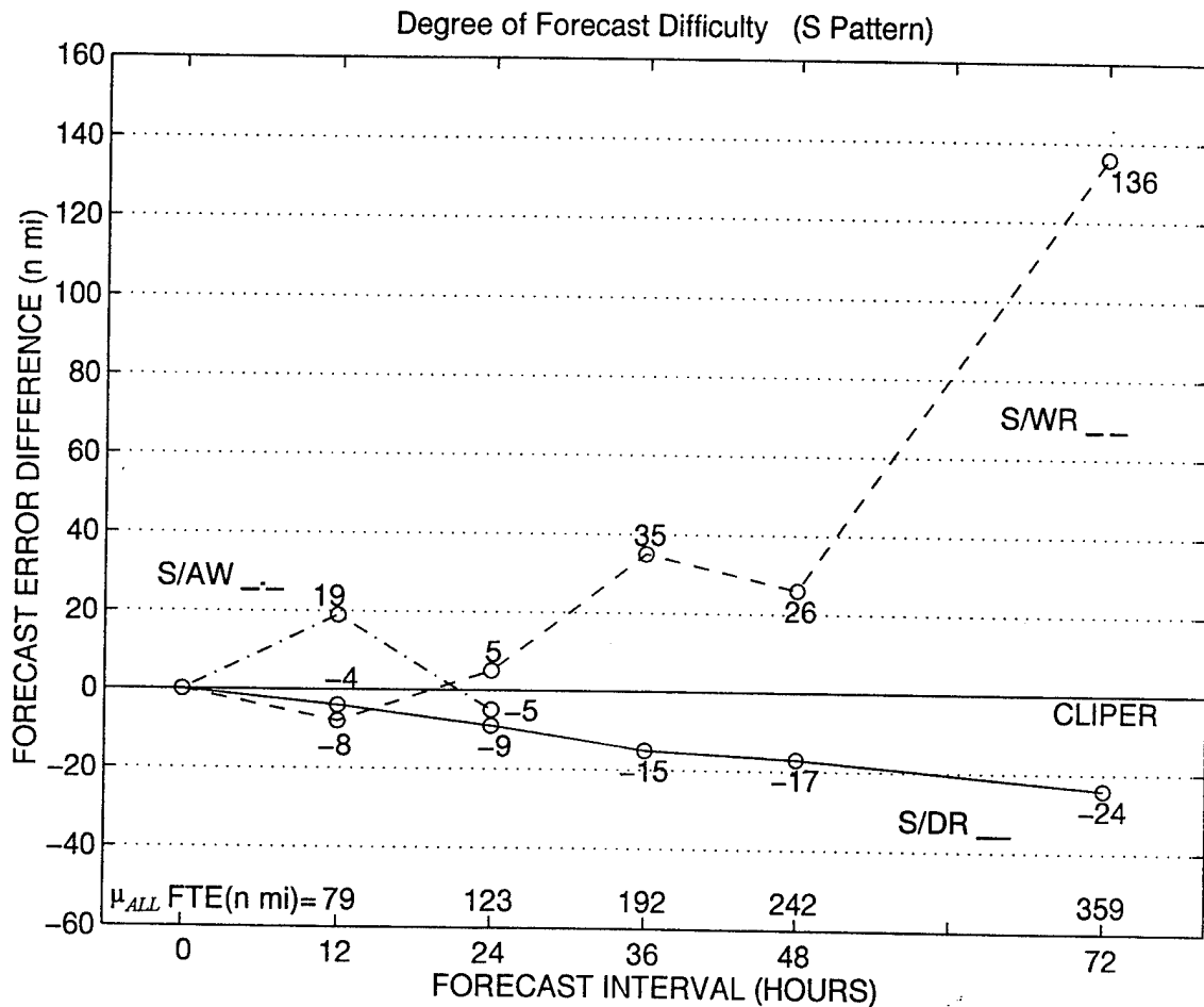
Figure 7 Degree of forecast difficulty of the Standard (S) Pattern. The CLIPER (ALL) FTEs ( \mu_{ALL} ) are indicated at the bottom of the figure and the CLIPER FTE differences ( \bar{x}_{P/R} - \mu_{ALL} ) used in Eq. (1) are the values along the plot of each Pattern/Region combination. See Table 2 for further details.
