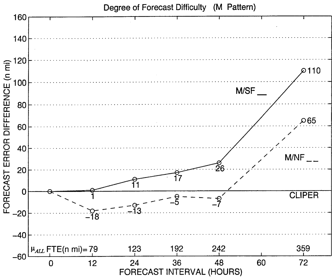
Figure 10 Degree of forecast difficulty as in Fig. 7, except for the Multiple (M) Cyclone Pattern. See Table 5 for further details.
