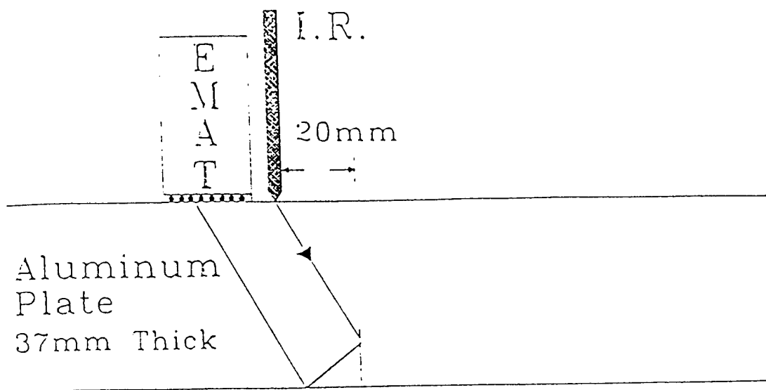
FIGURE 1. (a) Schematic diagram of single laser pulse excitation and EMAT detection of ultrasound in an aluminum plate with a one third through thickness cut simulating a crack.
