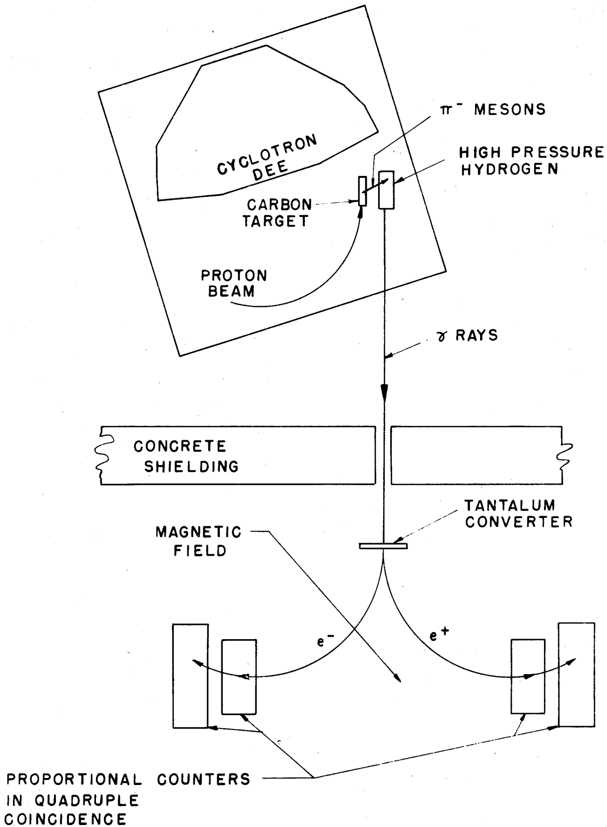
Fig. 1--Geometrical arrangement of cyclotron target, hydrogen pressure vessel, gamma ray collimators and pair spectrometer.
