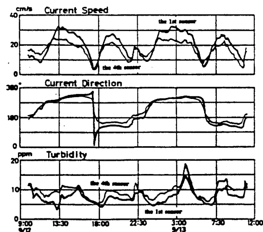
Fig. 4. Variations with time of the current speed, its direction and the turbidity got from the first and the fourth sensors of the current-shear meter.
