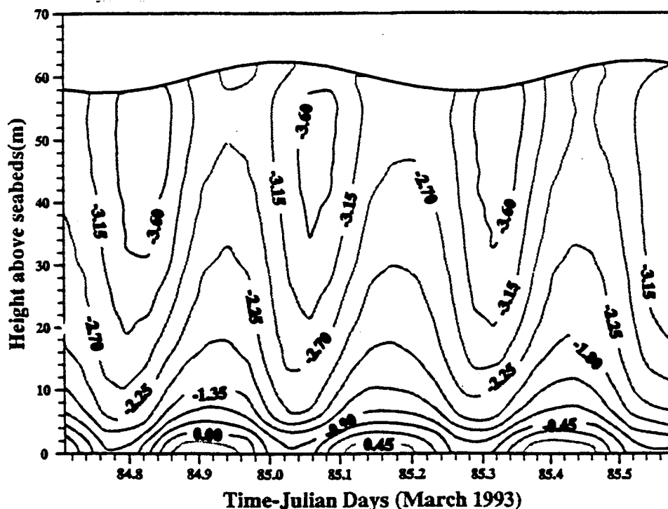
Figure 1. Variation of \log E ( \text{Wm}^{-3} ) over a 25 hour cycle from MY2.1 model at IS1 in the northern Irish Sea.
