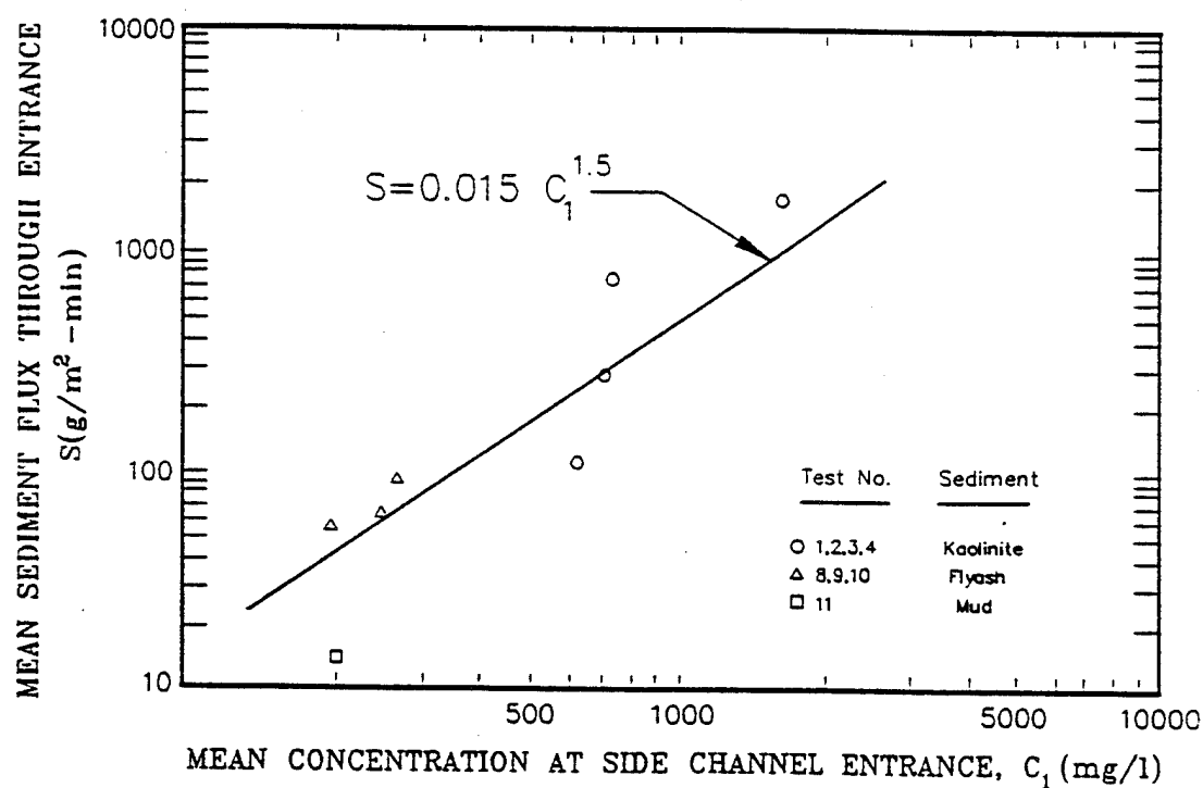
Figure 4. Mean sediment flux into the channel through entrance vs. mean concentration at entrance.
