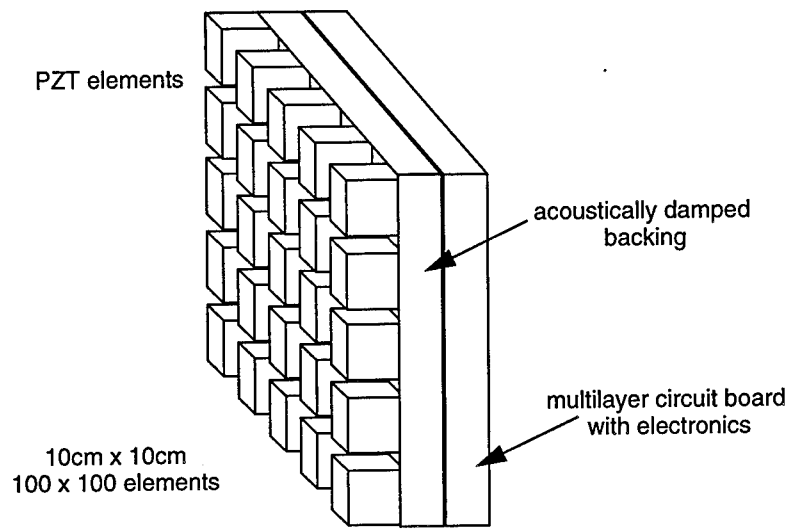
Figure 6-1. Schematic diagram of two-dimensional ultrasound array.
