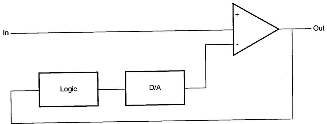
Figure 7-1. A/D Converter Block Diagram.
