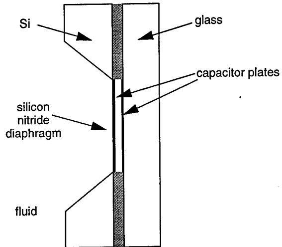
Figure 6-5. Schematic diagram of capacitive ultrasound sensor made using MEMS technology.
