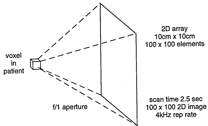
Figure 6-3. Schematic diagram of confocal two-dimensional ultrasound array.
