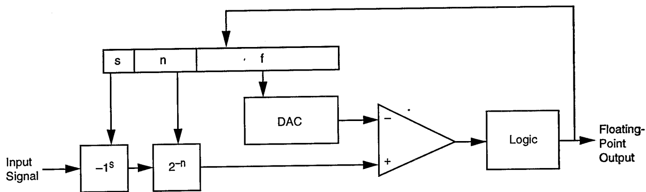
Figure 6-6. Block diagram of floating point analog-to-digital converter.
