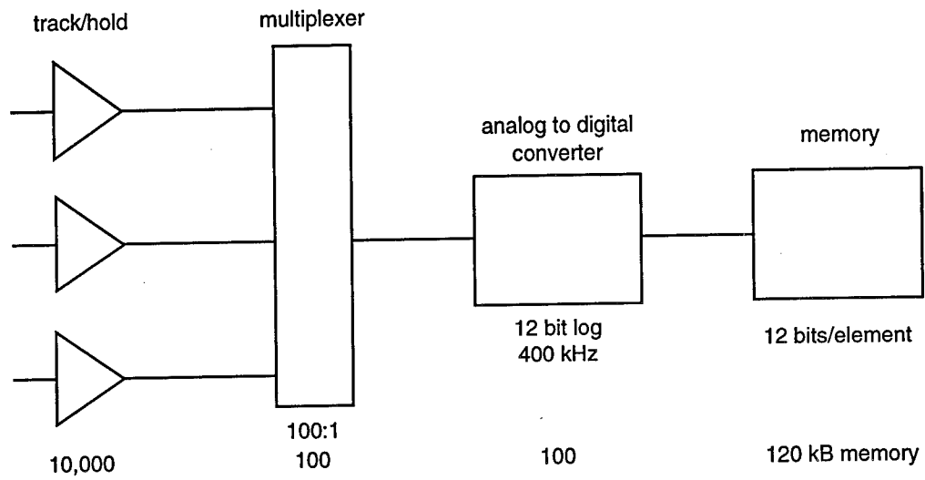
Figure 6-4. Block diagram of the electronics for confocal ultrasound array.
