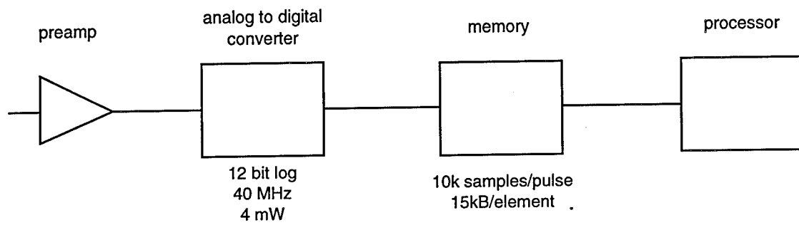
Figure 6-2. Block diagram of the receive electronics for one pixel of the array.
