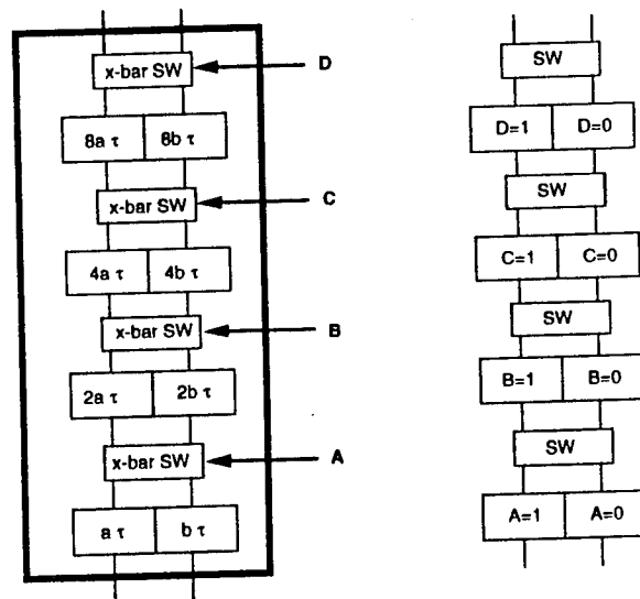
Figure 4.3.3-3 Airborne Array Four-Bit Dual Delay Network
