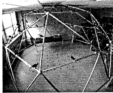
Figure 10: The V-ized Reality research platform, consisting of a dome with 51 cameras mounted on it and 51 VCRs that record the video from the cameras.
